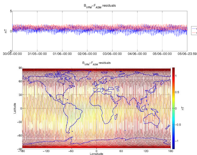
Figure 3-6: ASM-VFM residuals for S/C B, during monitoring period 30/05-05/06. In top figure are plotted: difference between |B_{VFM}| and F_{ASM} (without dB_Sun correction) (blue colour), and the residuals with dB_Sun corrections (red colour). In bottom figure residuals are presented on the world map.
