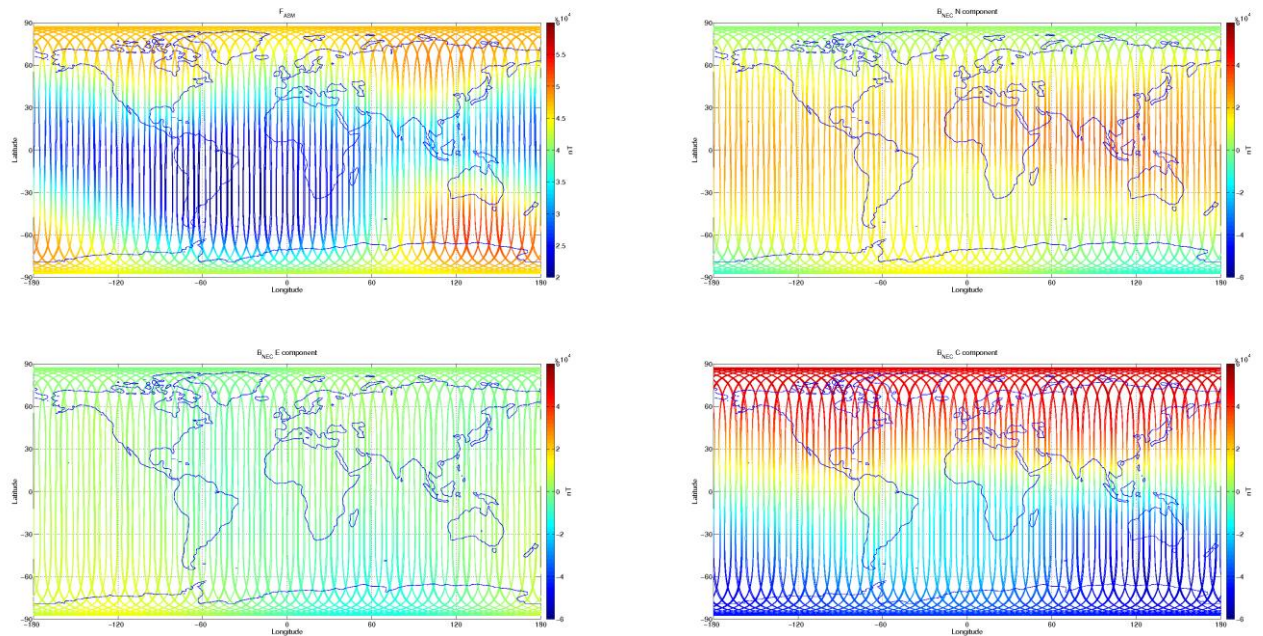
Figure 3-7: S/C A, world map plots of the geomagnetic field and components measured during monitoring period 30/05-05/06. From top to bottom: F-magnetic field from ASM measurement, B_{NEC} components (North, East, and Centre) of magnetic field from VFM measurement.
