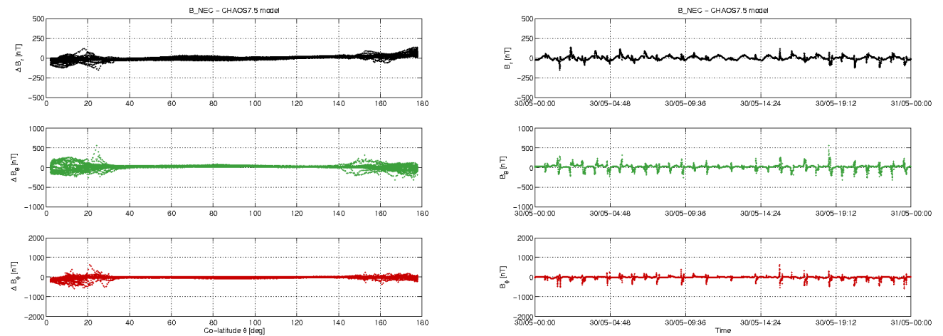
Figure 3-11: S/C B day 30/05: time series of B_{NEC} - B_{Chaos} residuals (right) and B_{NEC} - B_{Chaos} vs colatitude (left).
