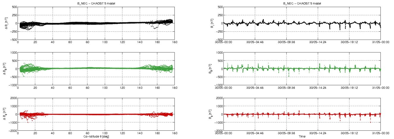
Figure 3-10: S/C A day 30/05: time series of B_{NEC} - B_{Chaos} residuals (right) and B_{NEC} - B_{Chaos} vs colatitude (left).
