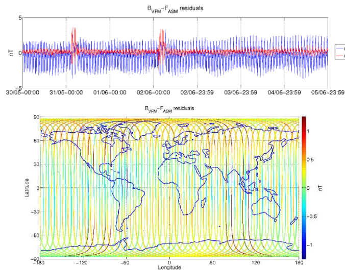
Figure 3-5: ASM-VFM residuals for S/C A, during monitoring period 30/05-05/06. In top figure are plotted: difference between |B_{VFM}| and F_{ASM} (without dB_{Sun} correction) (blue colour), and the residuals with dB_{Sun} corrections (red colour). In bottom figure residuals are presented on the world map.
