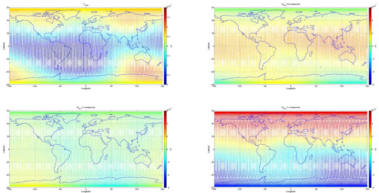
Figure 3-8: S/C B, world map plots of the geomagnetic field and components measured during monitoring period 30/05-05/06. From top to bottom: F-magnetic field from ASM measurement, B_{NEC} components (North, East, and Centre) of magnetic field from VFM measurement.
