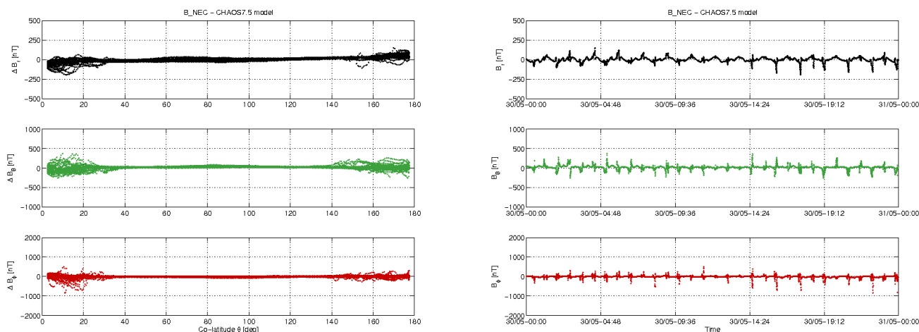
Figure 3-12: S/C C day 30/05: time series of B_{NEC} - B_{CHAOS} residuals (right) and B_{NEC} - B_{CHAOS} vs colatitude (left)
