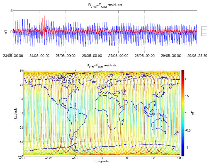
Figure 3-5: ASM-VFM residuals for S/C A, during monitoring period 23/05-29/05. In top figure are plotted: difference between |B_{VFM}| and F_{ASM} (without dB_{Sun} correction) (blue colour), and the residuals with dB_{Sun} corrections (red colour). In bottom figure residuals are presented on the world map.
