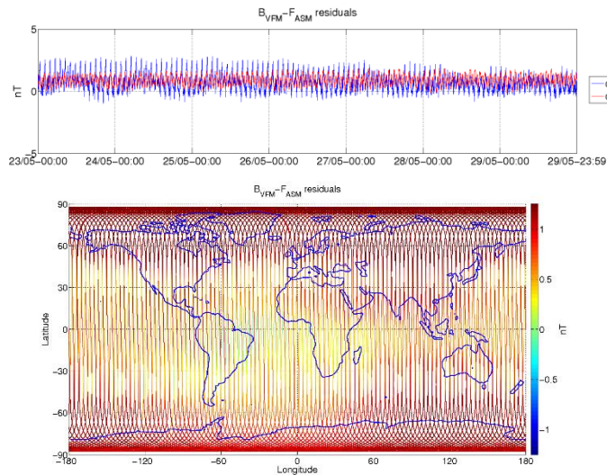
Figure 3-6: ASM-VFM residuals for S/C B, during monitoring period 23/05-29/05. In top figure are plotted: difference between |B_{VFM}| and F_{ASM} (without dB_{Sun} correction) (blue colour), and the residuals with dB_{Sun} corrections (red colour). In bottom figure residuals are presented on the world map.
