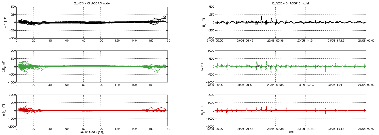
Figure 3-10: S/C A day 23/05: time series of B_{NEC} - B_{Chaos} residuals (right) and B_{NEC} - B_{Chaos} vs colatitude (left).
