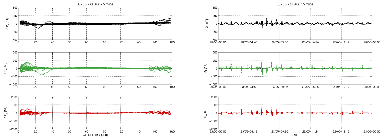
Figure 3-11: S/C B day 23/05: time series of B_{NEC} - B_{Chaos} residuals (right) and B_{NEC} - B_{Chaos} vs colatitude (left).
