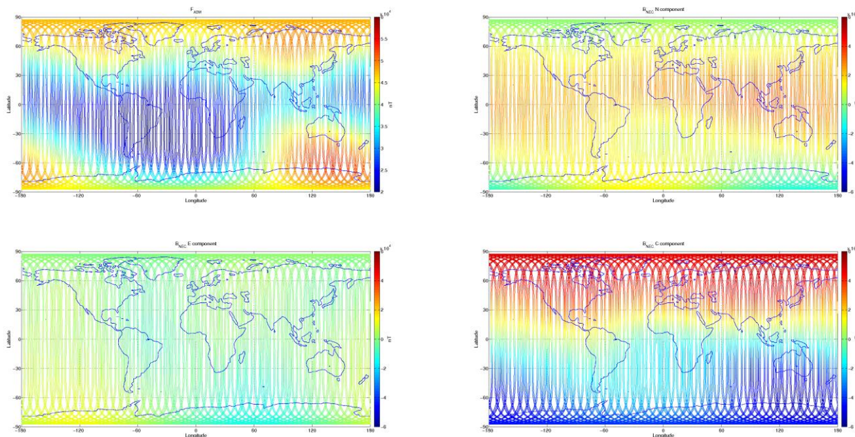
Figure 3-7: S/C A, world map plots of the geomagnetic field and components measured during monitoring period 23/05-29/05. From top to bottom: F-magnetic field from ASM measurement, B_{NEC} components (North, East, and Centre) of magnetic field from VFM measurement.
