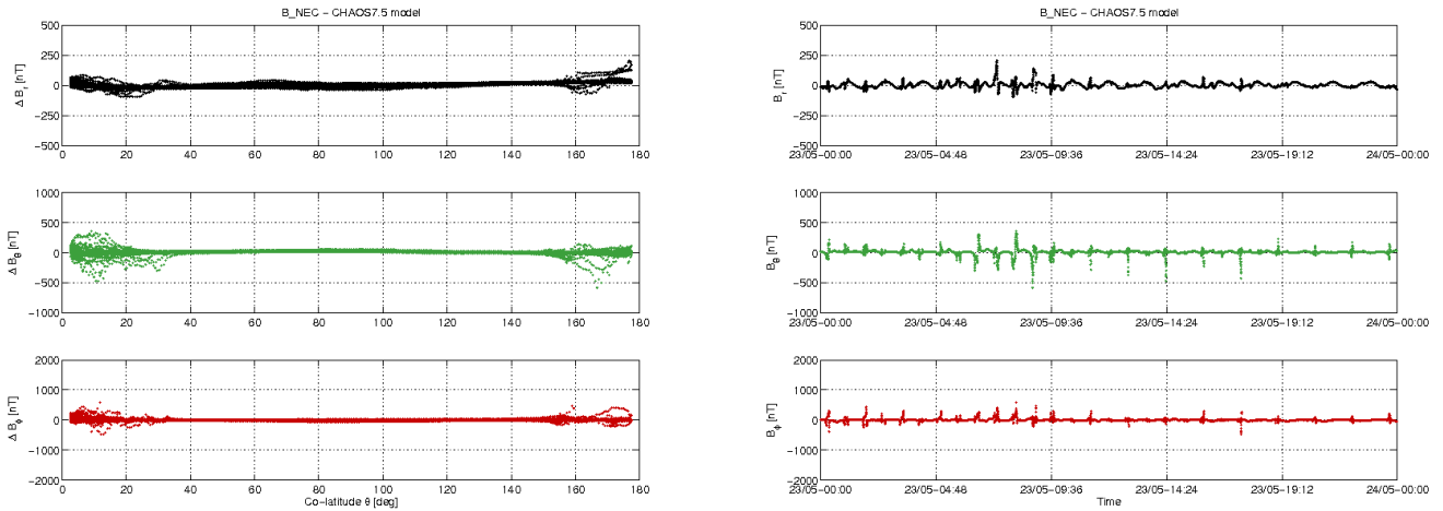
Figure 3-12: S/C C day 23/05: time series of B_{NEC} - B_{Chaos} residuals (right) and B_{NEC} - B_{Chaos} vs colatitude (left)
