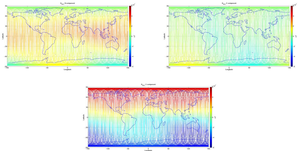
Figure 3-9: S/C C, world map plots of the geomagnetic field and components measured during monitoring period 16/05-22/05. From top to bottom: B_{NEC} components (North, East, and Centre) of magnetic field from VFM measurement.
