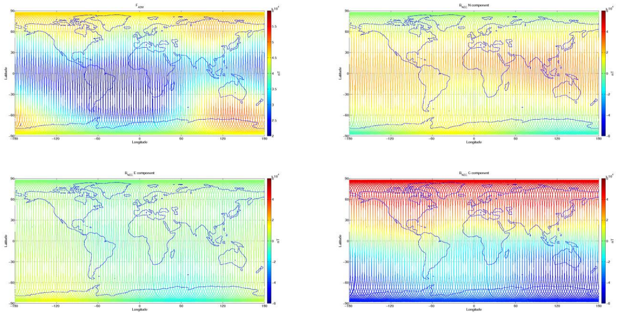
Figure 3-8: S/C B, world map plots of the geomagnetic field and components measured during monitoring period 16/05-22/05. From top to bottom: F-magnetic field from ASM measurement, B_{NEC} components (North, East, and Centre) of magnetic field from VFM measurement.
