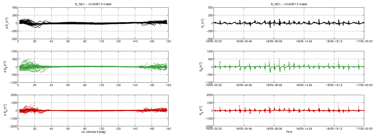
Figure 3-11: S/C B day 16/05: time series of B_{NEC} - B_{Chaos} residuals (right) and B_{NEC} - B_{Chaos} vs colatitude (left).
