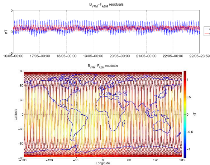
Figure 3-6: ASM-VFM residuals for S/C B, during monitoring period 16/05-22/05. In top figure are plotted: difference between |B_{VFM}| and F_{ASM} (without dB_{Sun} correction) (blue colour), and the residuals with dB_{Sun} corrections (red colour). In bottom figure residuals are presented on the world map.
