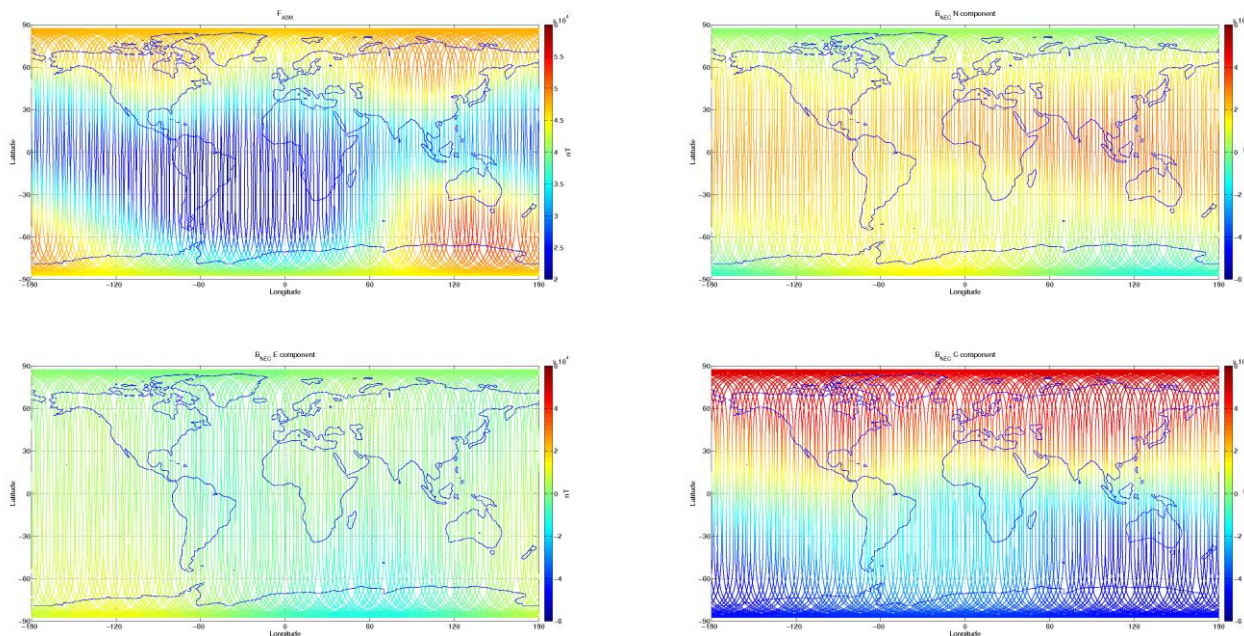
Figure 3-7: S/C A, world map plots of the geomagnetic field and components measured during monitoring period 16/05-22/05. From top to bottom: F-magnetic field from ASM measurement, B_{NEC} components (North, East, and Centre) of magnetic field from VFM measurement.
