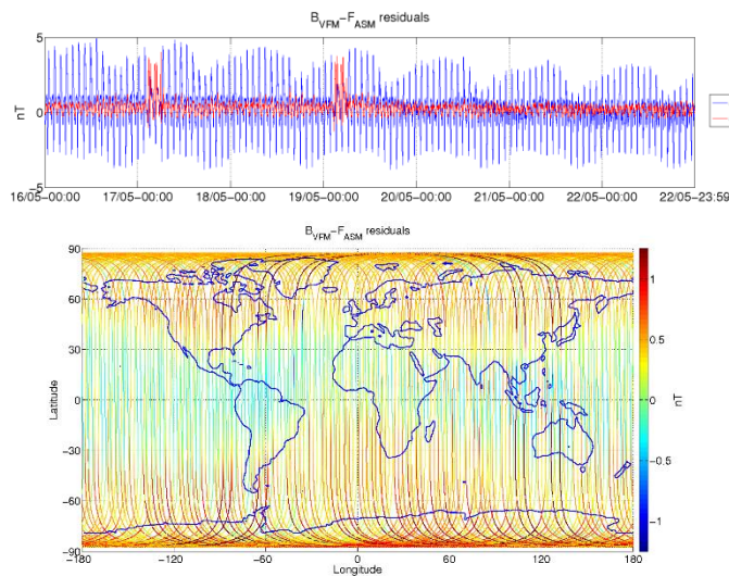
Figure 3-5: ASM-VFM residuals for S/C A, during monitoring period 16/05-22/05. In top figure are plotted: difference between |B_{VFM}| and F_{ASM} (without dB_{Sun} correction) (blue colour), and the residuals with dB_{Sun} corrections (red colour). In bottom figure residuals are presented on the world map.
