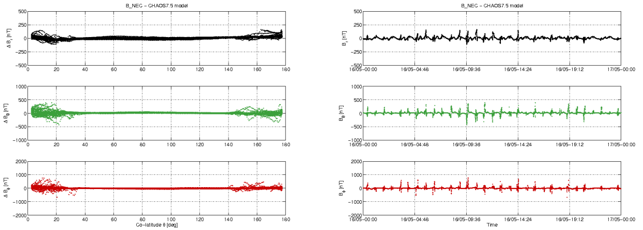
Figure 3-12: S/C C day 16/05: time series of B_{NEC} - B_{Chaos} residuals (right) and B_{NEC} - B_{Chaos} vs colatitude (left)
