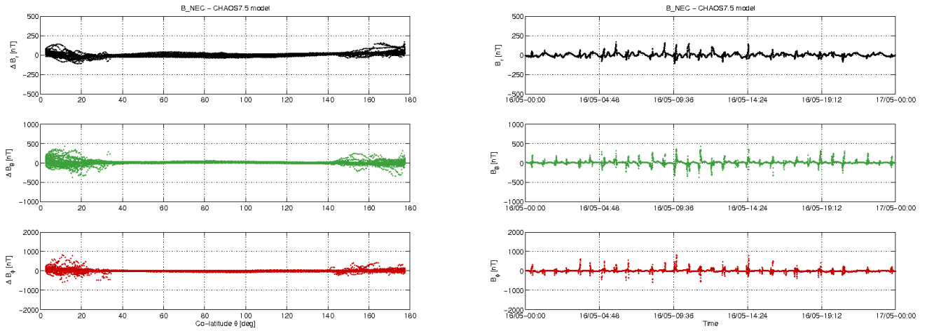
Figure 3-10: S/C A day 16/05: time series of B_{NEC} - B_{Chaos} residuals (right) and B_{NEC} - B_{Chaos} vs colatitude (left).
