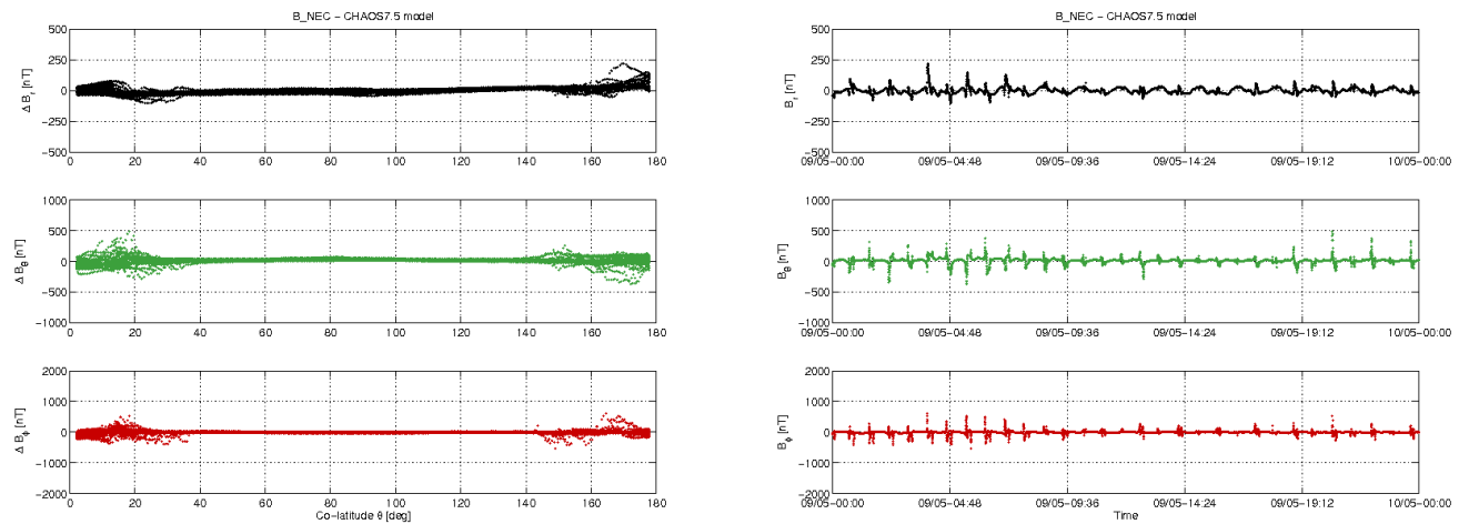
Figure 3-11: S/C B day 09/05: time series of B_{NEC} - B_{Chaos} residuals (right) and B_{NEC} - B_{Chaos} vs colatitude (left).
