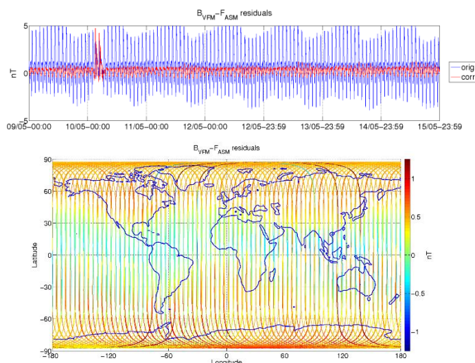
Figure 3-5: ASM-VFM residuals for S/C A, during monitoring period 09/05-15/05. In top figure are plotted: difference between |B_{VFM}| and F_{ASM} (without dB_Sun correction) (blue colour), and the residuals with dB_Sun corrections (red colour). In bottom figure residuals are presented on the world map.
