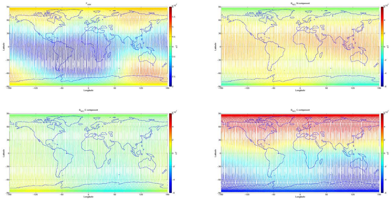
Figure 3-8: S/C B, world map plots of the geomagnetic field and components measured during monitoring period 09/05-15/05. From top to bottom: F-magnetic field from ASM measurement, B_{NEC} components (North, East, and Centre) of magnetic field from VFM measurement.
