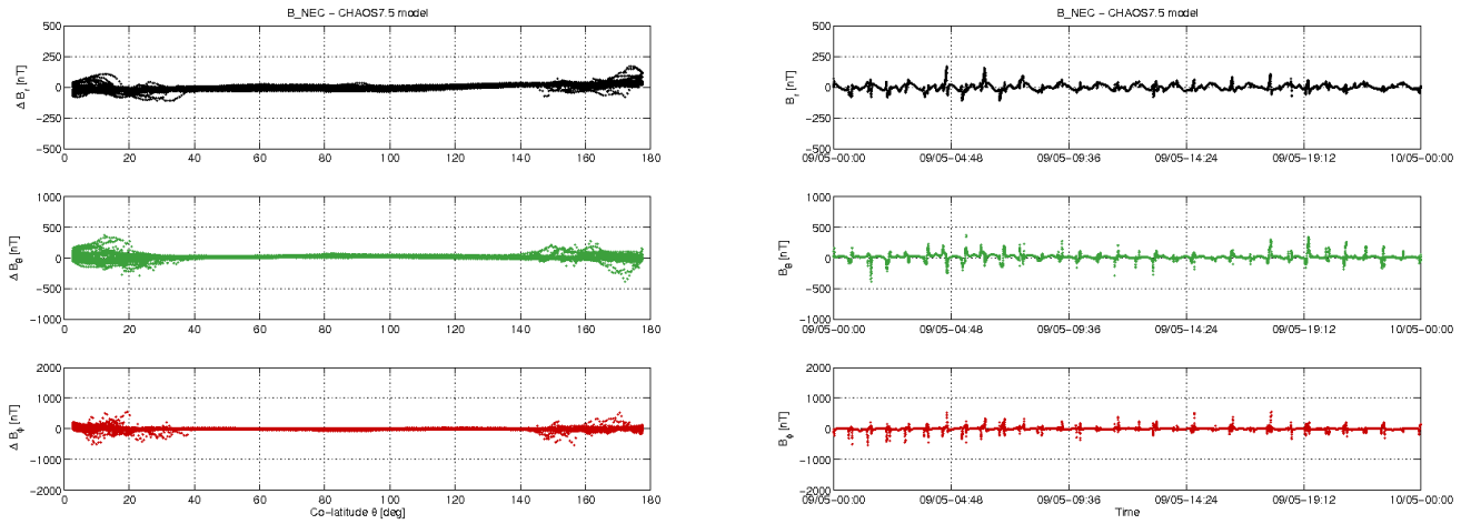
Figure 3-10: S/C A day 09/05: time series of B_{NEC} - B_{Chaos} residuals (right) and B_{NEC} - B_{Chaos} vs colatitude (left).
