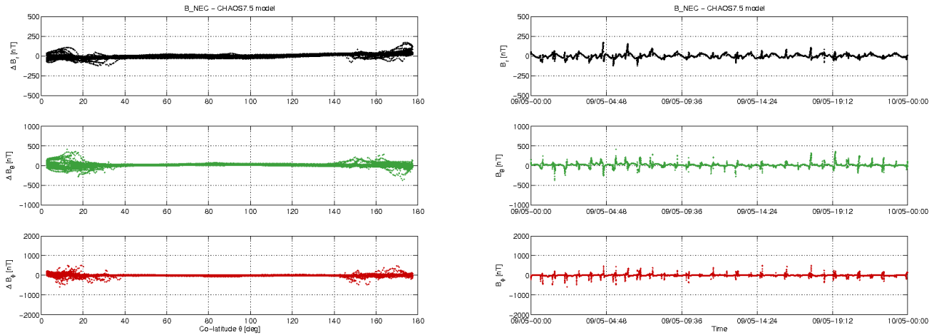
Figure 3-12: S/C C day 09/05: time series of B_{NEC} - B_{Chaos} residuals (right) and B_{NEC} - B_{Chaos} vs colatitude (left)
