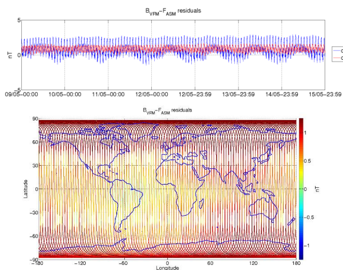
Figure 3-6: ASM-VFM residuals for S/C B, during monitoring period 09/05-15/05. In top figure are plotted: difference between |B_{VFM}| and F_{ASM} (without dB_{Sun} correction) (blue colour), and the residuals with dB_{Sun} corrections (red colour). In bottom figure residuals are presented on the world map.
