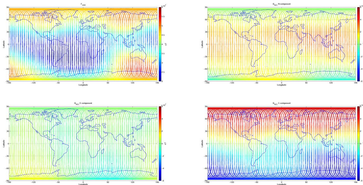
Figure 3-7: S/C A, world map plots of the geomagnetic field and components measured during monitoring period 09/05-15/05. From top to bottom: F-magnetic field from ASM measurement, B_{NEC} components (North, East, and Centre) of magnetic field from VFM measurement.
