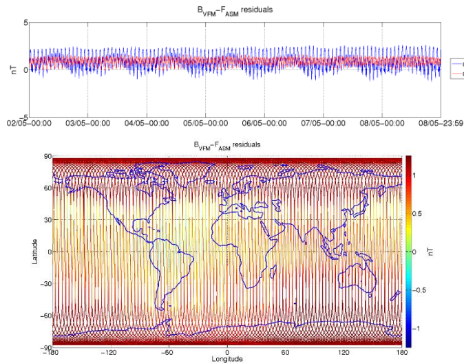
Figure 3-6: ASM-VFM residuals for S/C B, during monitoring period 02/05-08/05. In top figure are plotted: difference between |B_{VFM}| and F_{ASM} (without dB_{Sun} correction) (blue colour), and the residuals with dB_{Sun} corrections (red colour). In bottom figure residuals are presented on the world map.
