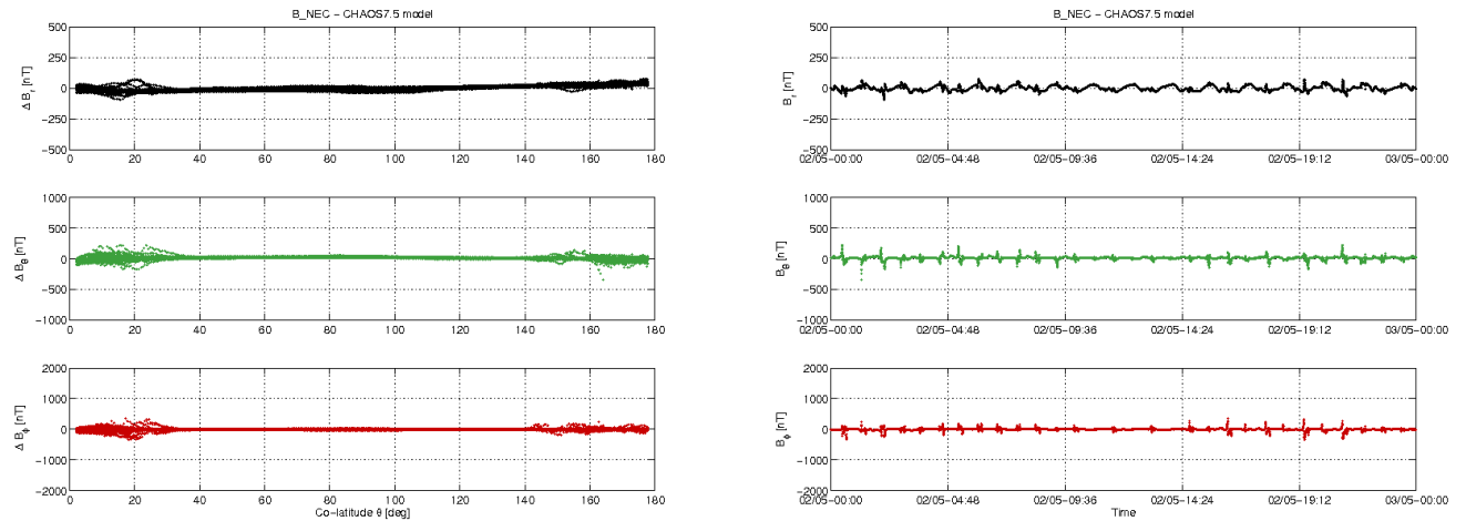
Figure 3-11: S/C B day 02.05: time series of B_{NEC} - B_{Chaos} residuals (right) and B_{NEC} - B_{Chaos} vs colatitude (left).
