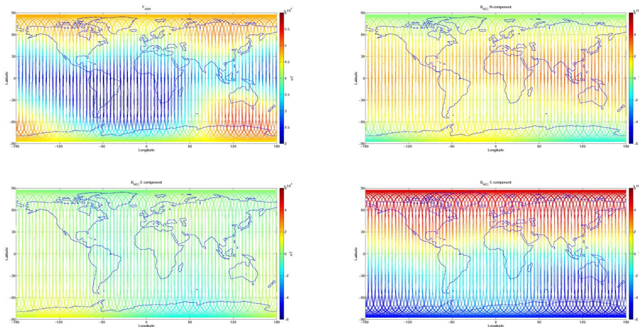
Figure 3-7: S/C A, world map plots of the geomagnetic field and components measured during monitoring period 02/05-08/05. From top to bottom: F-magnetic field from ASM measurement, B_{NEC} components (North, East, and Centre) of magnetic field from VFM measurement.
