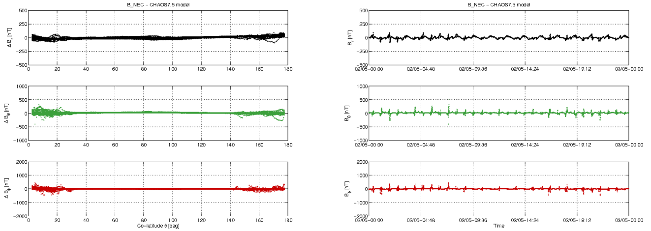
Figure 3-10: S/C A day 02.05: time series of B_{NEC} - B_{Chaos} residuals (right) and B_{NEC} - B_{Chaos} vs colatitude (left).
