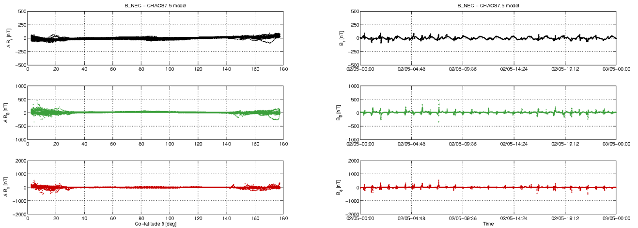
Figure 3-12: S/C C day 02.05: time series of B_{NEC} - B_{Chaos} residuals (right) and B_{NEC} - B_{Chaos} vs colatitude (left)
