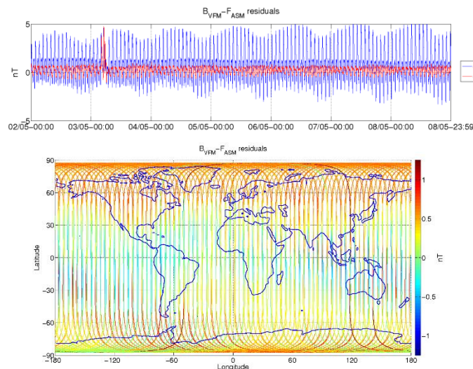
Figure 3-5: ASM-VFM residuals for S/C A, during monitoring period 02/05-08/05. In top figure are plotted: difference between |B_{VFM}| and F_{ASM} (without dB_Sun correction) (blue colour), and the residuals with dB_Sun corrections (red colour). In bottom figure residuals are presented on the world map.
