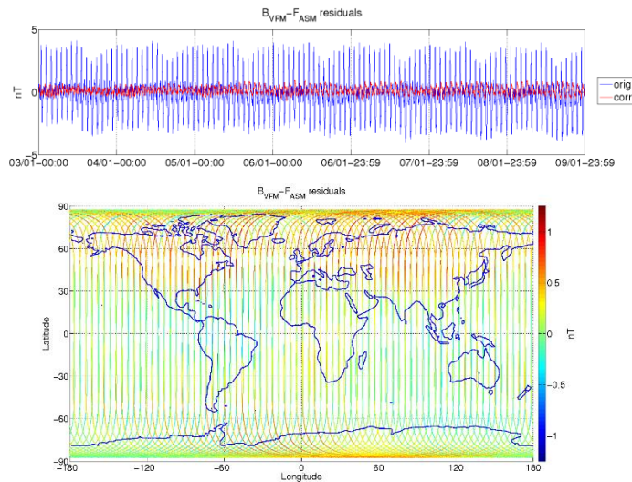
Figure 3-5: ASM-VFM residuals for S/C A, during monitoring period 03/01-09/01. In top figure are plotted: difference between |B_{VFM}| and F_{ASM} (without dB_{Sun} correction) (blue colour), and the residuals with dB_{Sun} corrections (red colour). In bottom figure residuals are presented on the world map.
