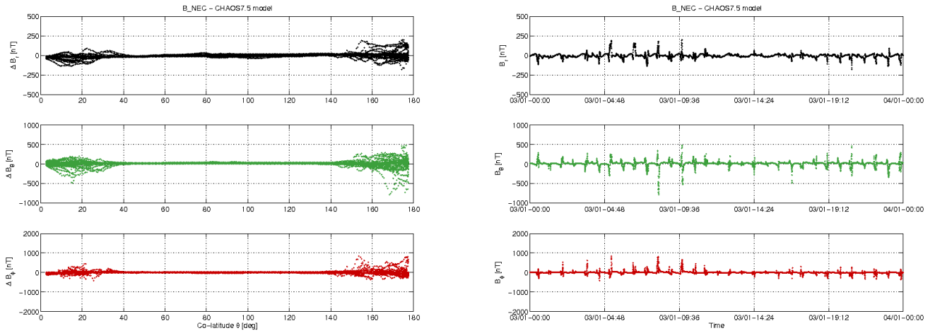
Figure 3-10: S/C A day 03.01: time series of B_{NEC} - B_{Chaos} residuals (right) and B_{NEC} - B_{Chaos} vs colatitude (left).
