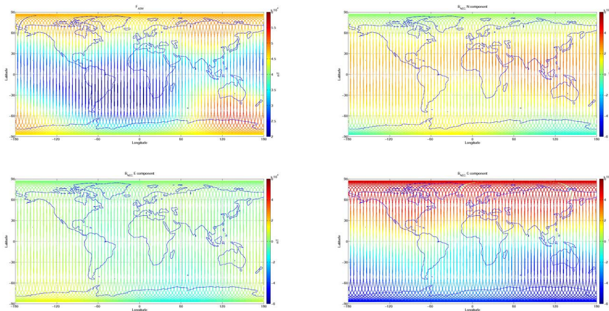
Figure 3-7: S/C A, world map plots of the geomagnetic field and components measured during monitoring period 03/01-09/01. From top to bottom: F-magnetic field from ASM measurement, B_{NEC} components (North, East, and Centre) of magnetic field from VFM measurement.
