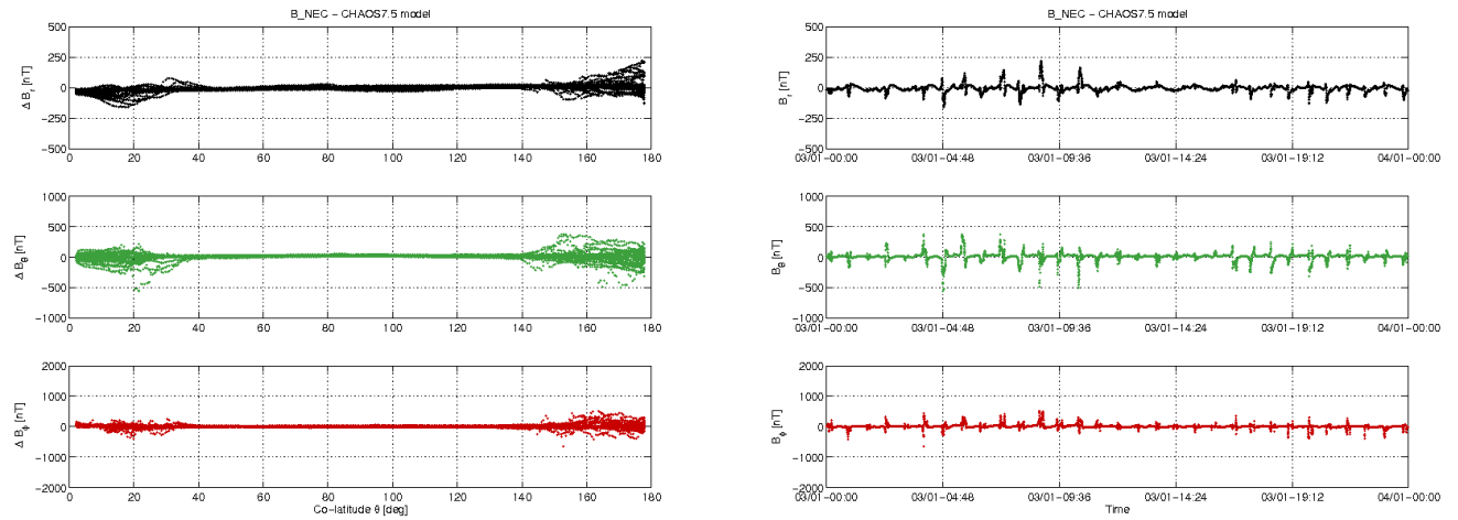
Figure 3-11: S/C B day 03.01: time series of B_{NEC} - B_{Chaos} residuals (right) and B_{NEC} - B_{Chaos} vs colatitude (left).
