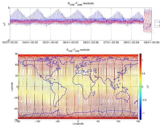
Figure 3-6: ASM-VFM residuals for S/C B, during monitoring period 03/01-09/01. In top figure are plotted: difference between |B_{VFM}| and F_{ASM} (without dB_{Sun} correction) (blue colour), and the residuals with dB_{Sun} corrections (red colour). In bottom figure residuals are presented on the world map.
