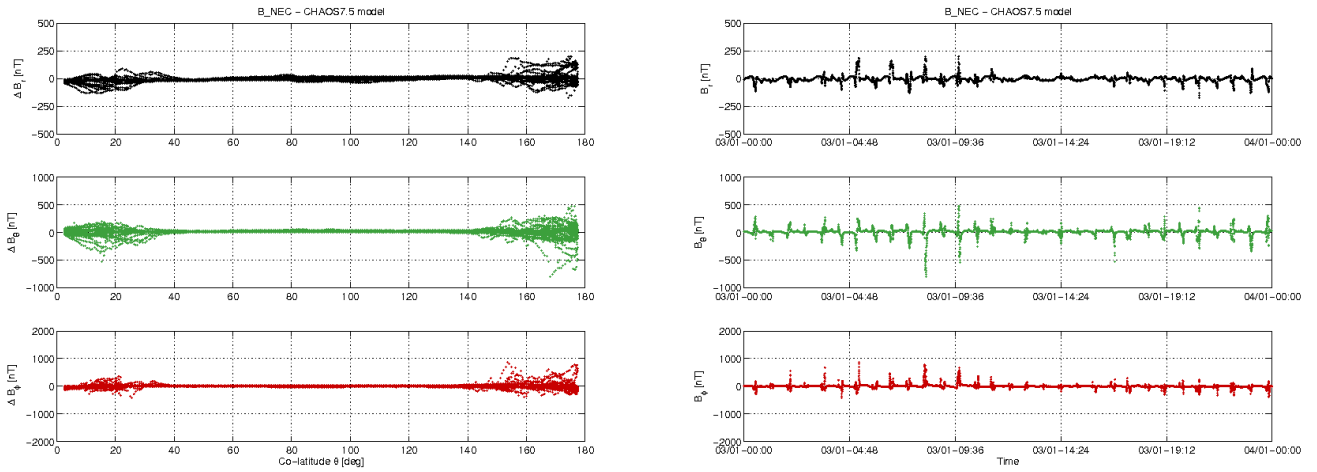
Figure 3-12: S/C C day 03.01: time series of B_{NEC} - B_{Chaos} residuals (right) and B_{NEC} - B_{Chaos} vs colatitude (left)
