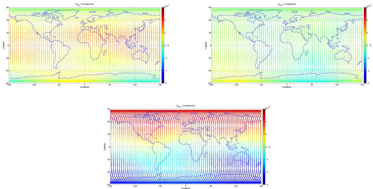
Figure 3-9: S/C C, world map plots of the geomagnetic field and components measured during monitoring period 03/01-09/01. From top to bottom: B_{NEC} components (North, East, and Centre) of magnetic field from VFM measurement.
