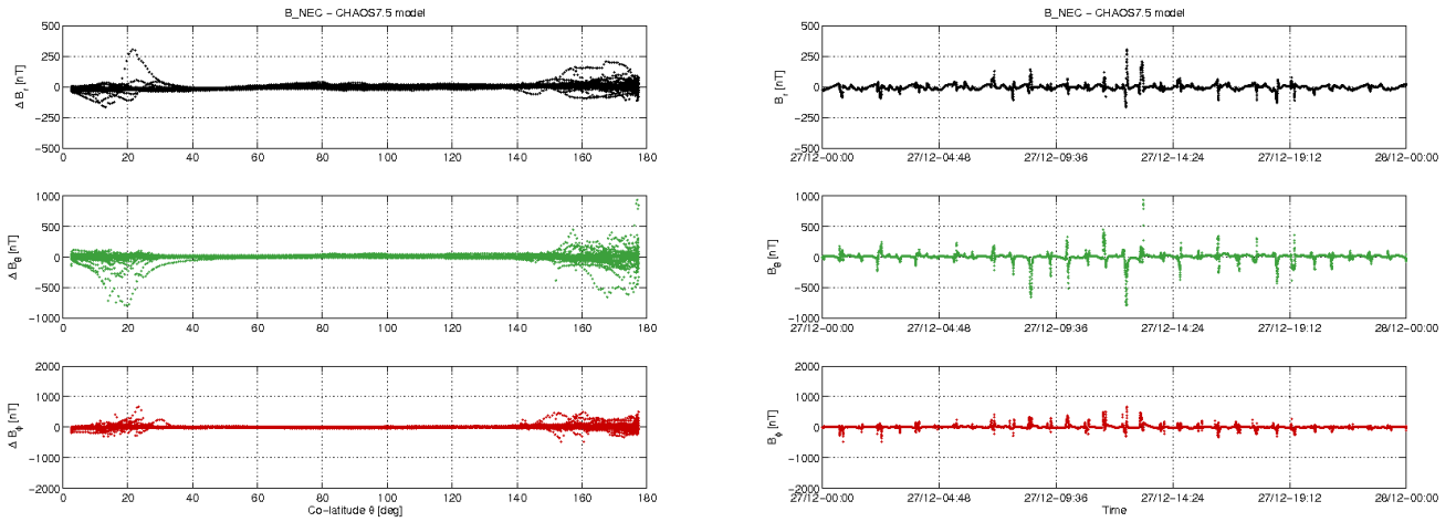
Figure 3-12: S/C C day 27.12: time series of B_{NEC} - B_{Chaos} residuals (right) and B_{NEC} - B_{Chaos} vs colatitude (left)
