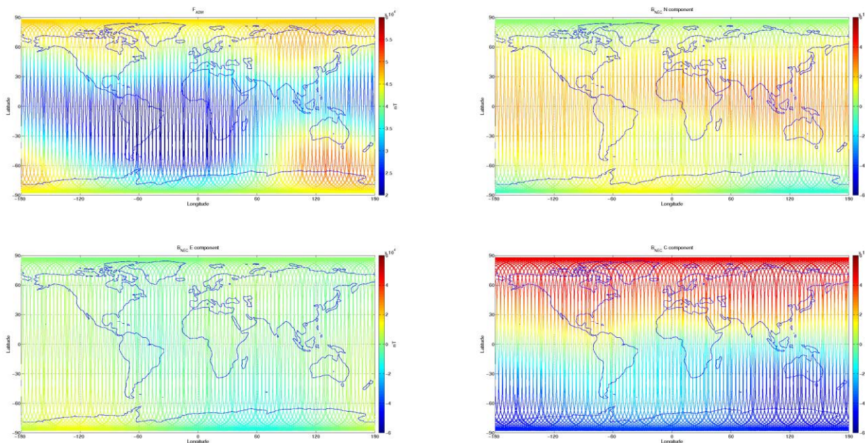
Figure 3-8: S/C B, world map plots of the geomagnetic field and components measured during monitoring period 27/12-02/01. From top to bottom: F-magnetic field from ASM measurement, B_{NEC} components (North, East, and Centre) of magnetic field from VFM measurement.
