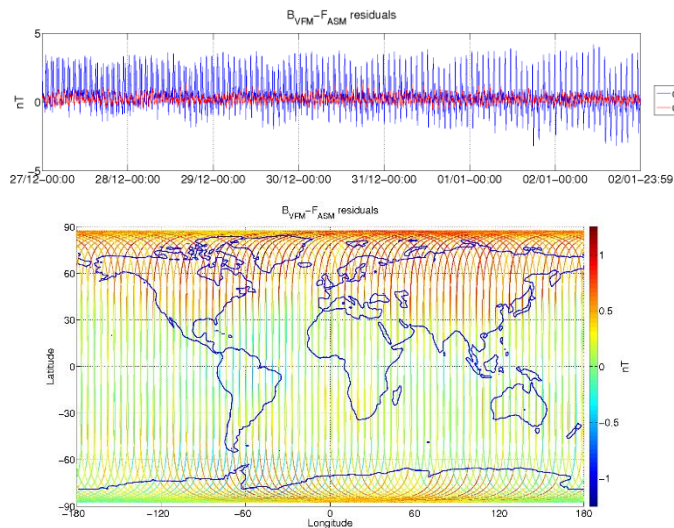
Figure 3-5: ASM-VFM residuals for S/C A, during monitoring period 27/12-02/01. In top figure are plotted: difference between |B_{VFM}| and F_{ASM} (without dB_{Sun} correction) (blue colour), and the residuals with dB_{Sun} corrections (red colour). In bottom figure residuals are presented on the world map.
