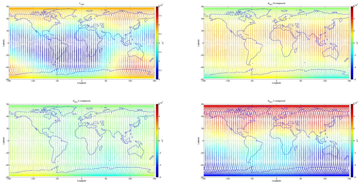
Figure 3-7: S/C A, world map plots of the geomagnetic field and components measured during monitoring period 27/12-02/01. From top to bottom: F-magnetic field from ASM measurement, B_{NEC} components (North, East, and Centre) of magnetic field from VFM measurement.
