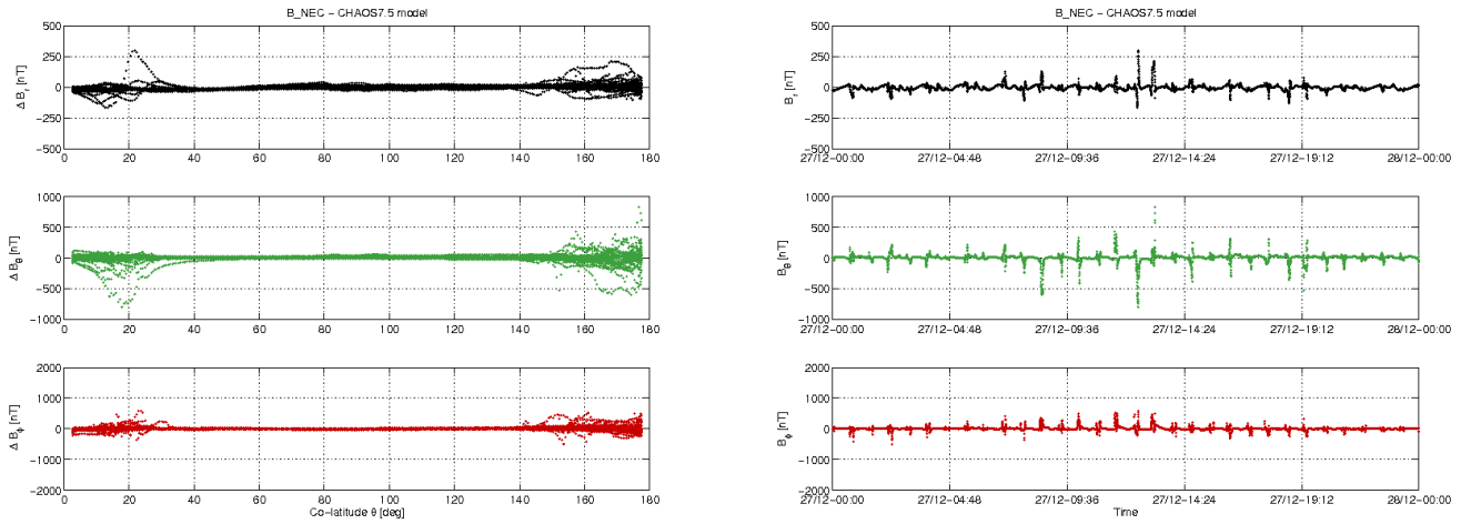
Figure 3-10: S/C A day 27.12: time series of B_{NEC} - B_{Chaos} residuals (right) and B_{NEC} - B_{Chaos} vs colatitude (left).
