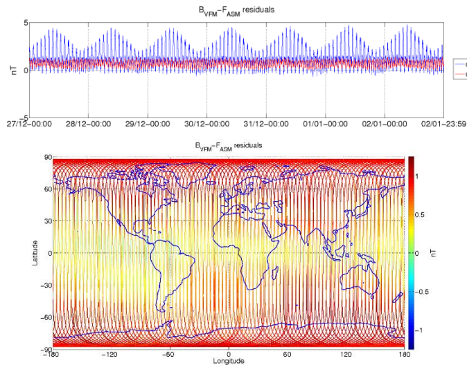
Figure 3-6: ASM-VFM residuals for S/C B, during monitoring period 27/12-02/01. In top figure are plotted: difference between |B_{VFM}| and F_{ASM} (without dB_{Sun} correction) (blue colour), and the residuals with dB_{Sun} corrections (red colour). In bottom figure residuals are presented on the world map.
