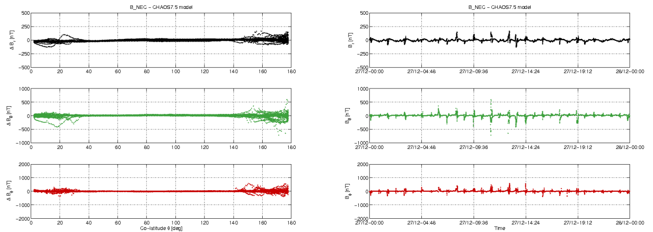
Figure 3-11: S/C B day 27.12: time series of B_{NEC} - B_{Chaos} residuals (right) and B_{NEC} - B_{Chaos} vs colatitude (left).
