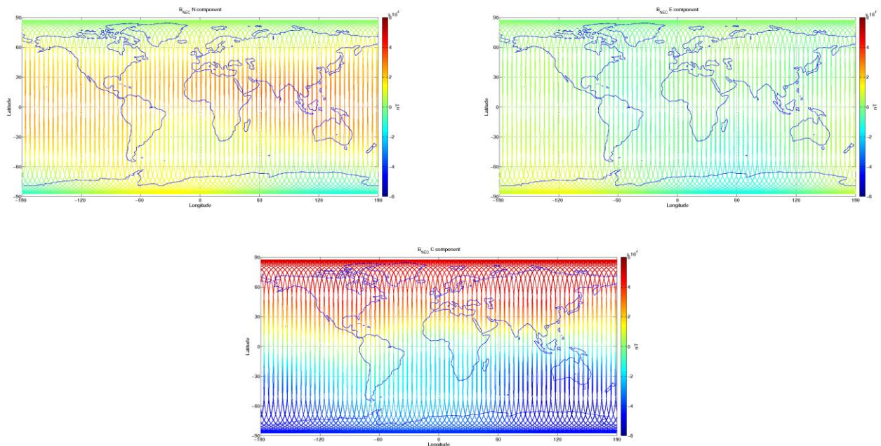
Figure 3-9: S/C C, world map plots of the geomagnetic field and components measured during monitoring period 27/12-02/01. From top to bottom: B_{NEC} components (North, East, and Centre) of magnetic field from VFM measurement.
