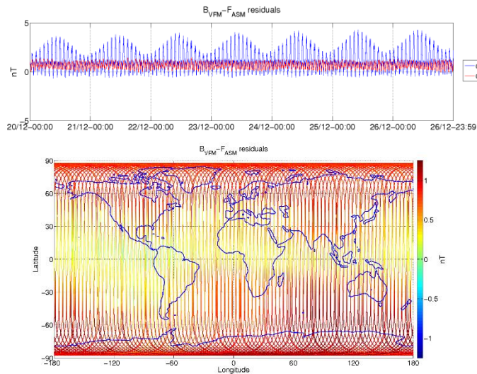
Figure 3-6: ASM-VFM residuals for S/C B, during monitoring period 20/12-26/12. In top figure are plotted: difference between |B_{VFM}| and F_{ASM} (without dB_{Sun} correction) (blue colour), and the residuals with dB_{Sun} corrections (red colour). In bottom figure residuals are presented on the world map.
