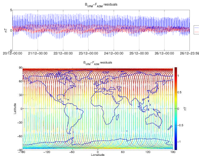
Figure 3-5: ASM-VFM residuals for S/C A, during monitoring period 20/12-26/12. In top figure are plotted: difference between |B_{VFM}| and F_{ASM} (without dB_Sun correction) (blue colour), and the residuals with dB_Sun corrections (red colour). In bottom figure residuals are presented on the world map.
