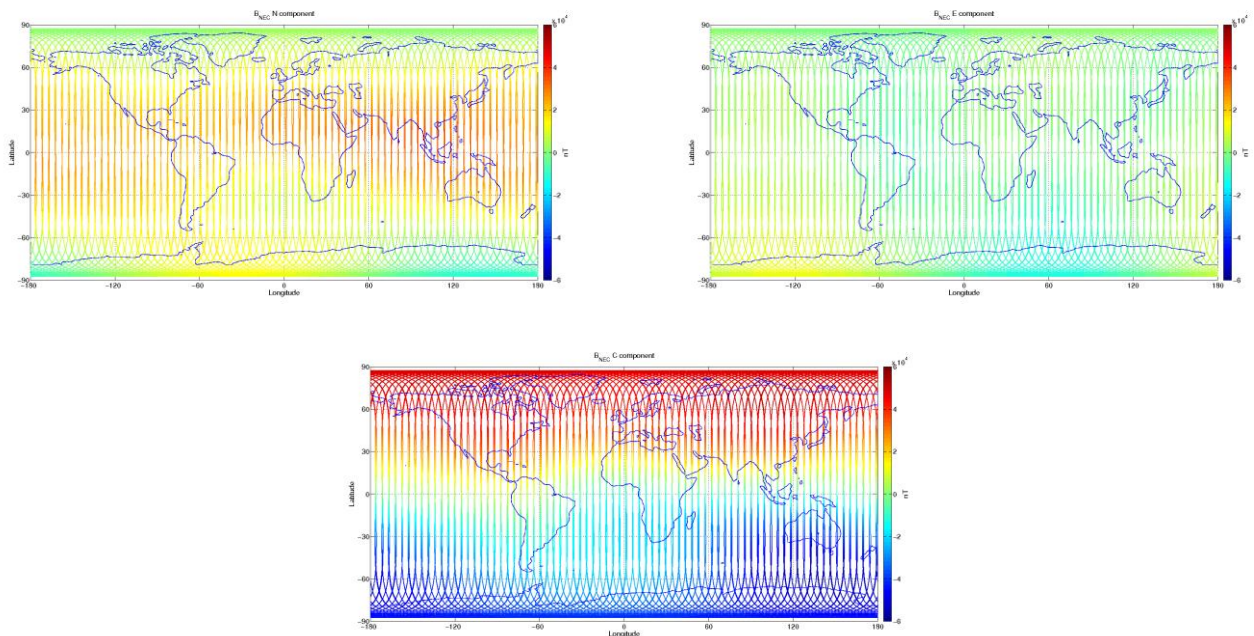
Figure 3-9: S/C C, world map plots of the geomagnetic field and components measured during monitoring period 20/12-26/12. From top to bottom: B_{NEC} components (North, East, and Centre) of magnetic field from VFM measurement.
