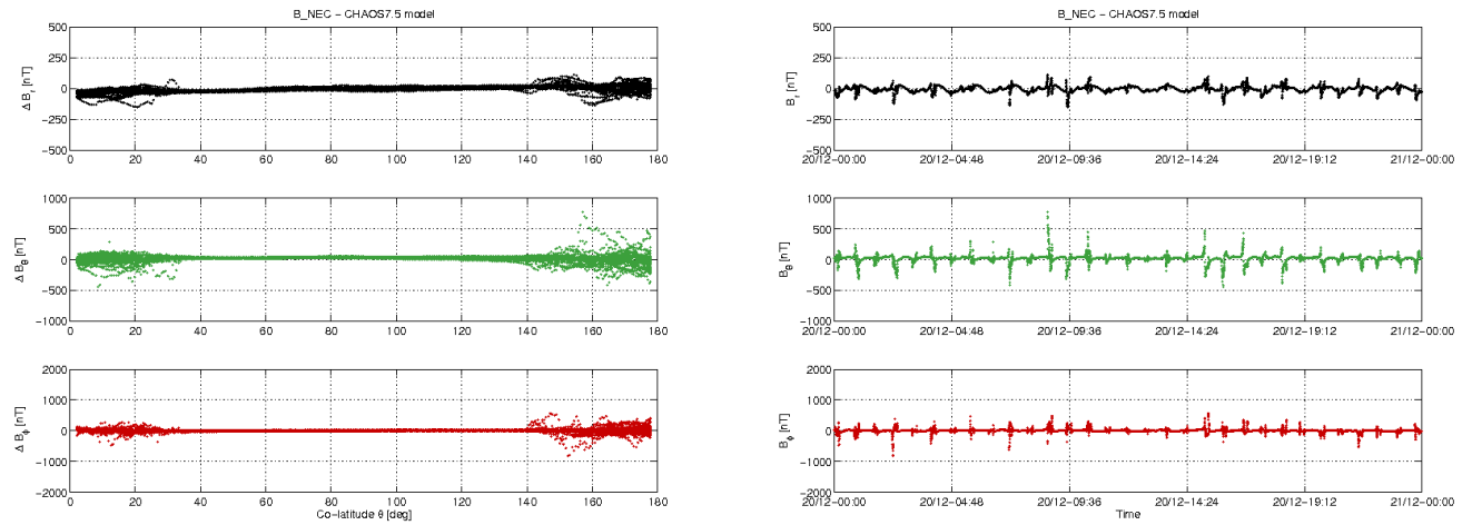
Figure 3-11: S/C B day 20.12: time series of B_{NEC} - B_{Chaos} residuals (right) and B_{NEC} - B_{Chaos} vs colatitude (left).
