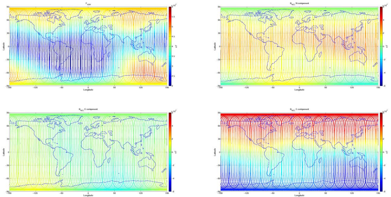
Figure 3-8: S/C B, world map plots of the geomagnetic field and components measured during monitoring period 20/12-26/12. From top to bottom: F-magnetic field from ASM measurement, B_{NEC} components (North, East, and Centre) of magnetic field from VFM measurement.
