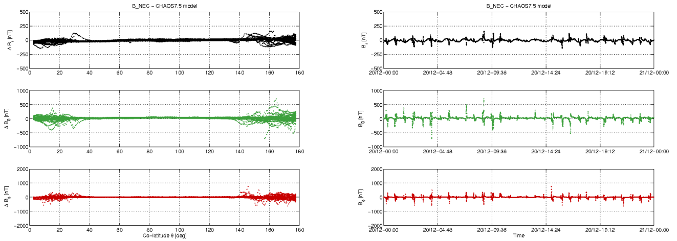
Figure 3-10: S/C A day 20.12: time series of B_{NEC} - B_{Chaos} residuals (right) and B_{NEC} - B_{Chaos} vs colatitude (left).
