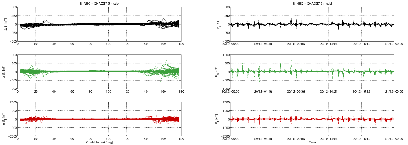
Figure 3-12: S/C C day 20.12: time series of B_{NEC} - B_{Chaos} residuals (right) and B_{NEC} - B_{Chaos} vs colatitude (left)
