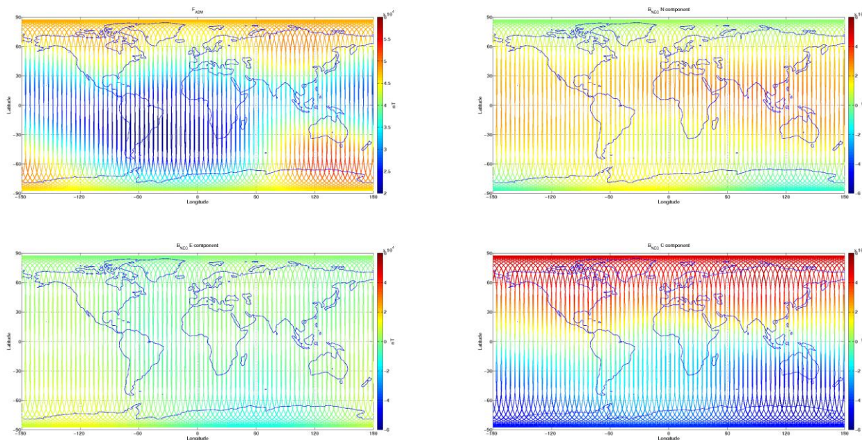
Figure 3-7: S/C A, world map plots of the geomagnetic field and components measured during monitoring period 20/12-26/12. From top to bottom: F-magnetic field from ASM measurement, B_{NEC} components (North, East, and Centre) of magnetic field from VFM measurement.
