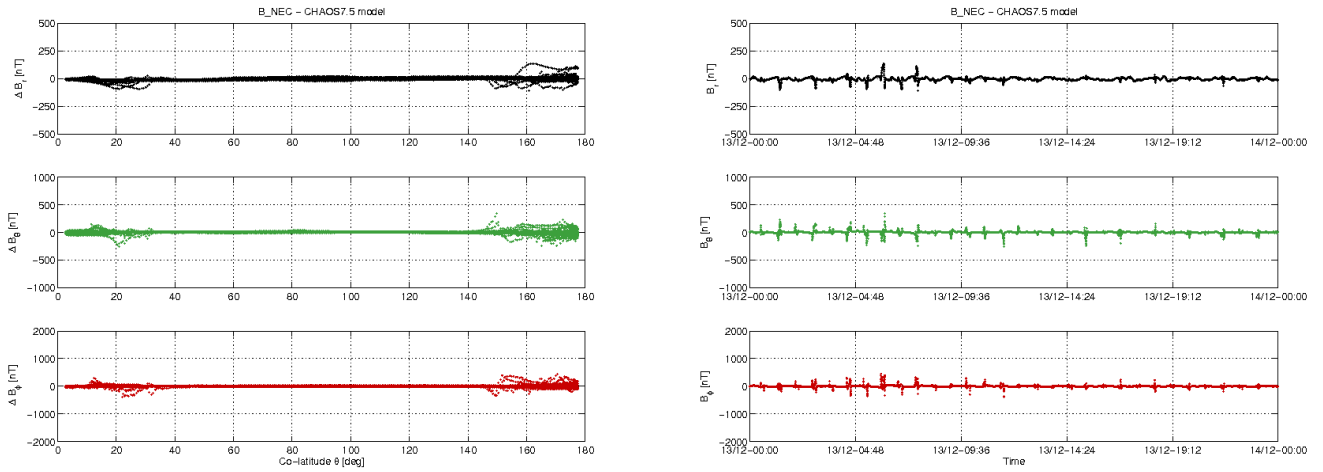
Figure 3-10: S/C A day 13.12: time series of B_{NEC} - B_{Chaos} residuals (right) and B_{NEC} - B_{Chaos} vs colatitude (left).
