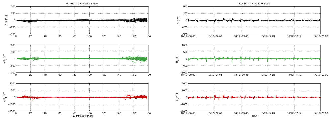
Figure 3-11: S/C B day 13.12: time series of B_{NEC} - B_{Chaos} residuals (right) and B_{NEC} - B_{Chaos} vs colatitude (left).
