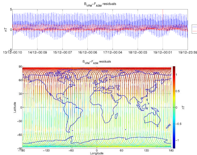
Figure 3-5: ASM-VFM residuals for S/C A, during monitoring period 13/12-19/12. In top figure are plotted: difference between |B_{VFM}| and F_{ASM} (without dB_{Sun} correction) (blue colour), and the residuals with dB_{Sun} corrections (red colour). In bottom figure residuals are presented on the world map.
