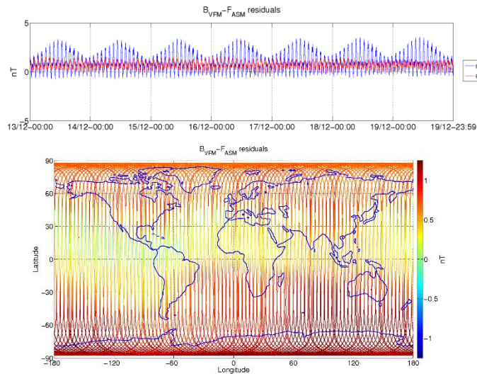
Figure 3-6: ASM-VFM residuals for S/C B, during monitoring period 13/12-19/12. In top figure are plotted: difference between |B_{VFM}| and F_{ASM} (without dB_{Sun} correction) (blue colour), and the residuals with dB_{Sun} corrections (red colour). In bottom figure residuals are presented on the world map.
