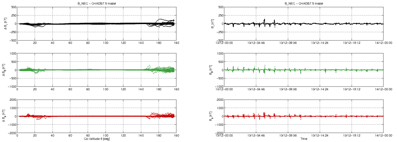
Figure 3-12: S/C C day 13/12: time series of B_{NEC} - B_{Chaos} residuals (right) and B_{NEC} - B_{Chaos} vs colatitude (left)
