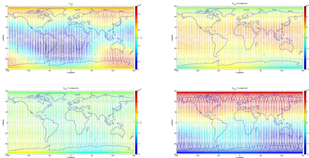
Figure 3-7: S/C A, world map plots of the geomagnetic field and components measured during monitoring period 13/12-19/12. From top to bottom: F-magnetic field from ASM measurement, B_{NEC} components (North, East, and Centre) of magnetic field from VFM measurement.
