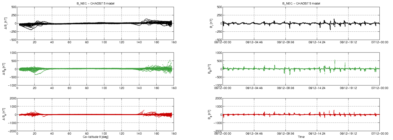
Figure 3-10: S/C A day 06.12: time series of B_{NEC} - B_{Chaos} residuals (right) and B_{NEC} - B_{Chaos} vs colatitude (left).
