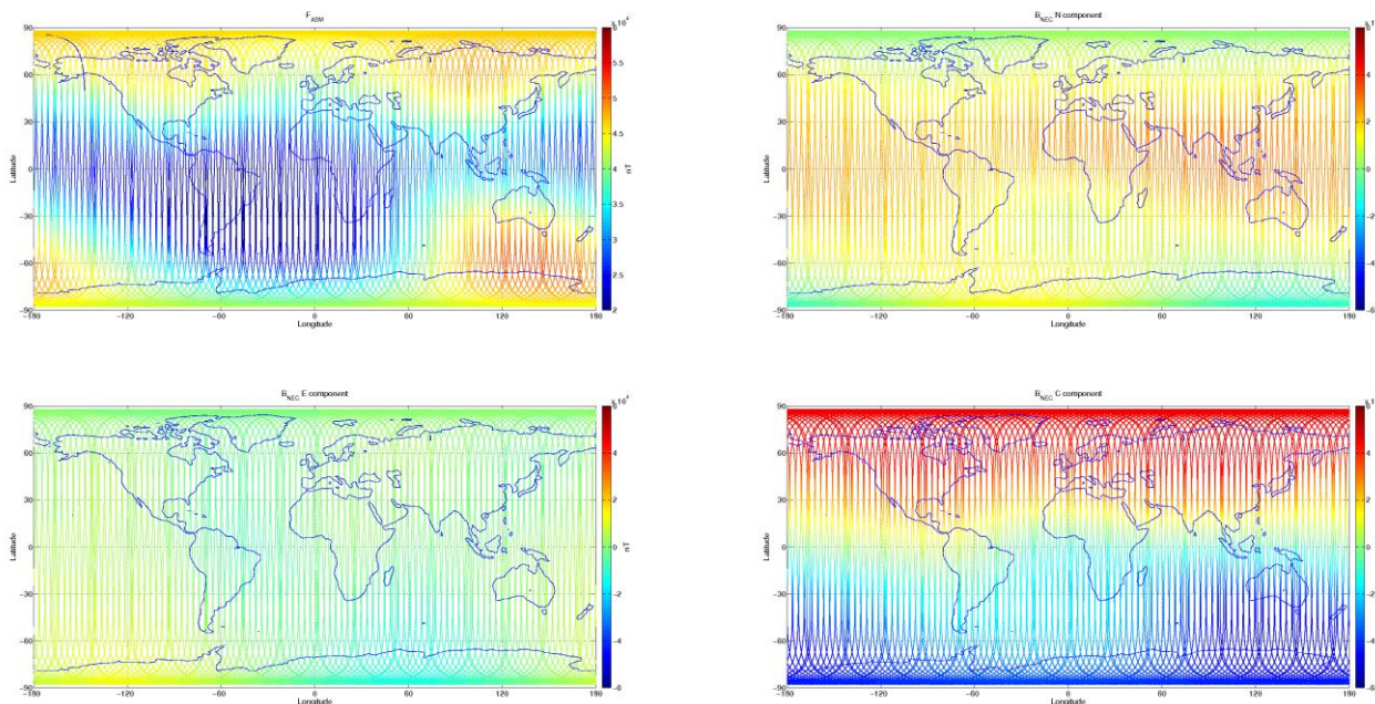
Figure 3-8: S/C B, world map plots of the geomagnetic field and components measured during monitoring period 06/12-12/12. From top to bottom: F-magnetic field from ASM measurement, B_{NEC} components (North, East, and Centre) of magnetic field from VFM measurement.
