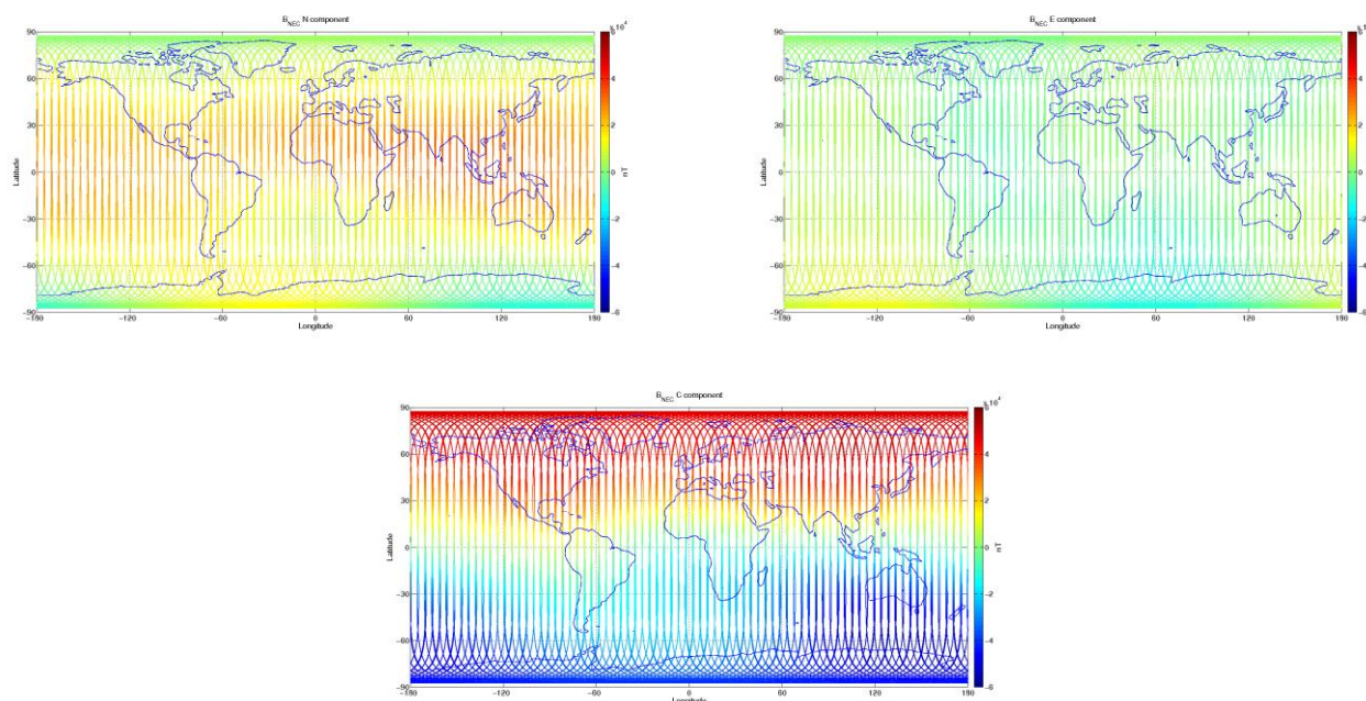
Figure 3-9: S/C C, world map plots of the geomagnetic field and components measured during monitoring period 06/12-12/12. From top to bottom: B_{NEC} components (North, East, and Centre) of magnetic field from VFM measurement.
