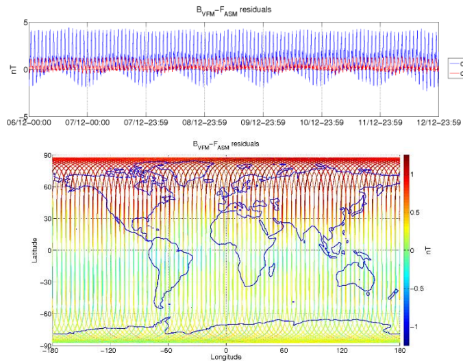
Figure 3-5: ASM-VFM residuals for S/C A, during monitoring period 06/12-12/12. In top figure are plotted: difference between |B_{VFM}| and F_{ASM} (without dB_{Sun} correction) (blue colour), and the residuals with dB_{Sun} corrections (red colour). In bottom figure residuals are presented on the world map.
