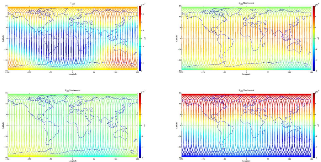
Figure 3-7: S/C A, world map plots of the geomagnetic field and components measured during monitoring period 06/12-12/12. From top to bottom: F-magnetic field from ASM measurement, B_{NEC} components (North, East, and Centre) of magnetic field from VFM measurement.
