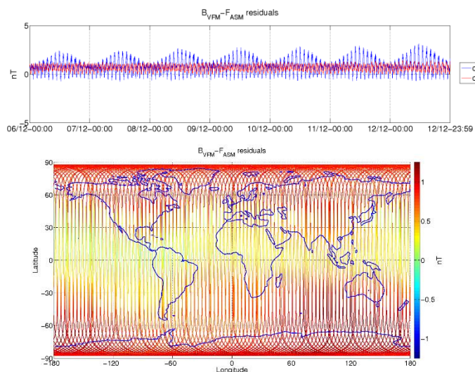
Figure 3-6: ASM-VFM residuals for S/C B, during monitoring period 06/12-12/12. In top figure are plotted: difference between |B_{VFM}| and F_{ASM} (without dB_{Sun} correction) (blue colour), and the residuals with dB_{Sun} corrections (red colour). In bottom figure residuals are presented on the world map.
