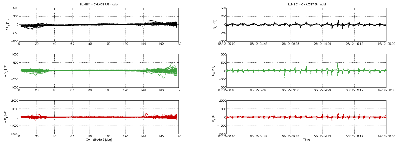
Figure 3-11: S/C B day 06.12: time series of B_{NEC} - B_{Chaos} residuals (right) and B_{NEC} - B_{Chaos} vs colatitude (left).
