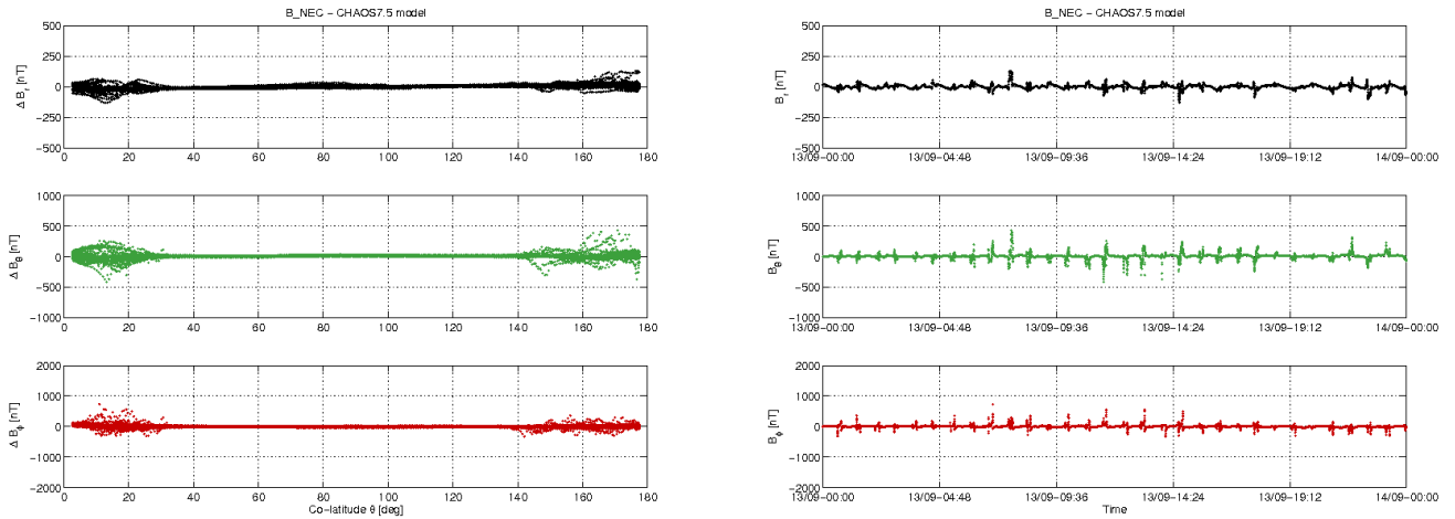
Figure 3-12: S/C C day 13.09: time series of B_{NEC} - B_{Chaos} residuals (right) and B_{NEC} - B_{Chaos} vs colatitude (left)
