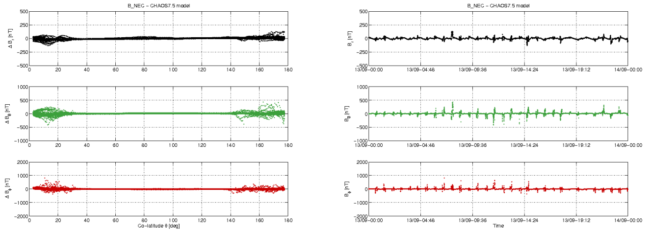
Figure 3-10: S/C A day 13.09: time series of B_{NEC} - B_{Chao5} residuals (right) and B_{NEC} - B_{Chao5} vs colatitude (left).
