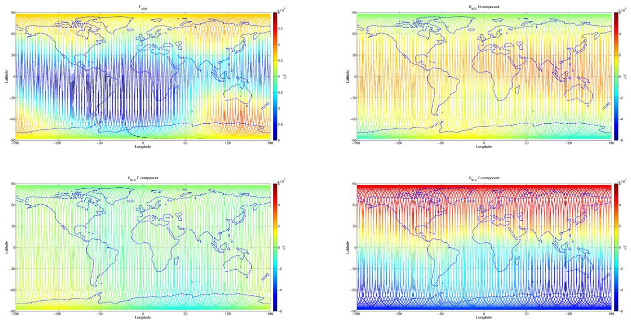
Figure 3-8: S/C B, world map plots of the geomagnetic field and components measured during monitoring period 13/09-19/09. From top to bottom: F-magnetic field from ASM measurement, B_{NEC} components (North, East, and Centre) of magnetic field from VFM measurement.
