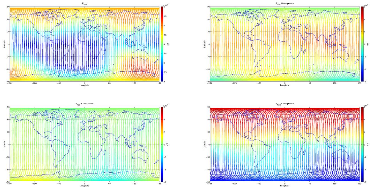
Figure 3-7: S/C A, world map plots of the geomagnetic field and components measured during monitoring period 13/09-19/09. From top to bottom: F-magnetic field from ASM measurement, B_{NEC} components (North, East, and Centre) of magnetic field from VFM measurement.
