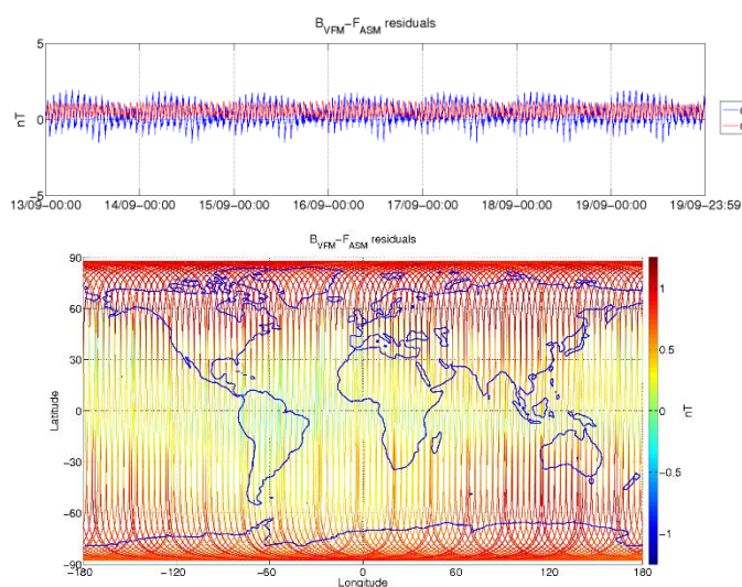
Figure 3-6: ASM-VFM residuals for S/C B, during monitoring period 13/09-19/09. In top figure are plotted: difference between |B_{VFM}| and F_{ASM} (without dB_{Sun} correction) (blue colour), and the residuals with dB_{Sun} corrections (red colour). In bottom figure residuals are presented on the world map.
