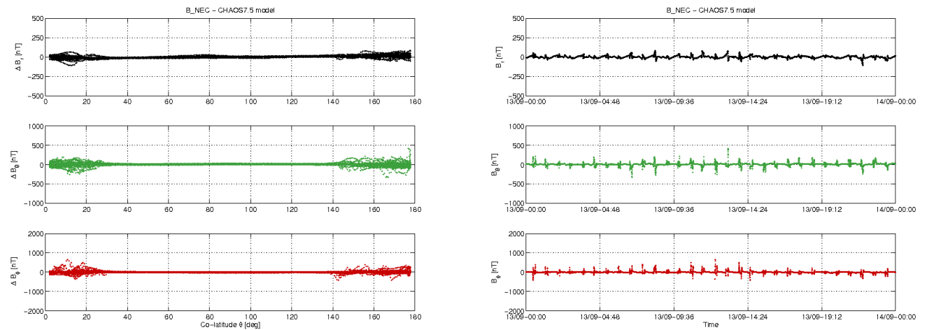
Figure 3-11: S/C B day 13.09: time series of B_{NEC} - B_{Chao5} residuals (right) and B_{NEC} - B_{Chao5} vs colatitude (left).
