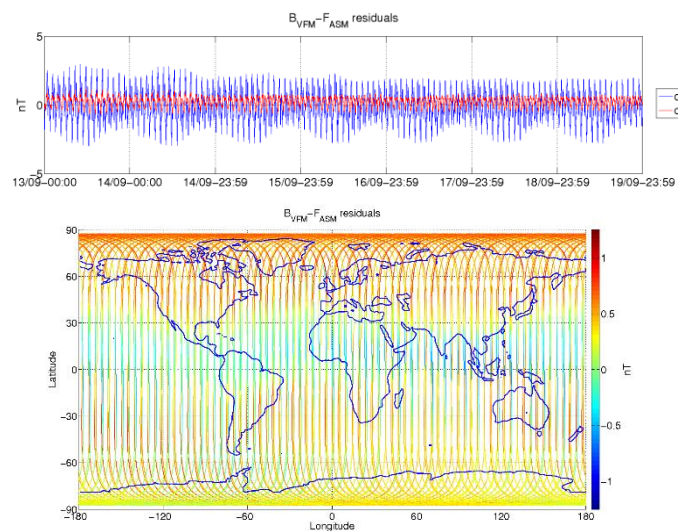
Figure 3-5: ASM-VFM residuals for S/C A, during monitoring period 13/09-19/09. In top figure are plotted: difference between |B_{VFM}| and F_{ASM} (without dB_{Sun} correction) (blue colour), and the residuals with dB_{Sun} corrections (red colour). In bottom figure residuals are presented on the world map.
