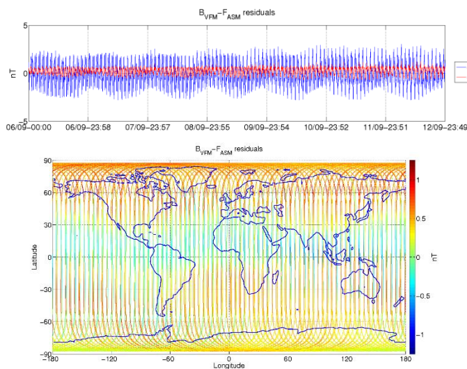
Figure 3-5: ASM-VFM residuals for S/C A, during monitoring period 06/09-12/09. In top figure are plotted: difference between |B_{VFM}| and F_{ASM} (without dB_{Sun} correction) (blue colour), and the residuals with dB_{Sun} corrections (red colour). In bottom figure residuals are presented on the world map.
