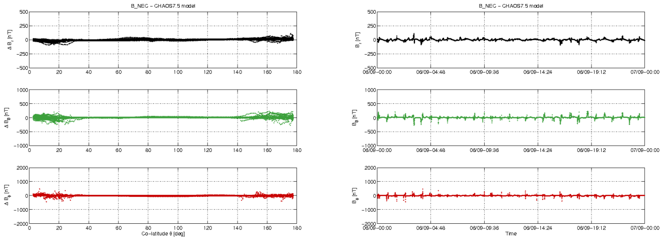
Figure 3-12: S/C C day 06.09: time series of B_{NEC} - B_{Chaos} residuals (right) and B_{NEC} - B_{Chaos} vs colatitude (left)
