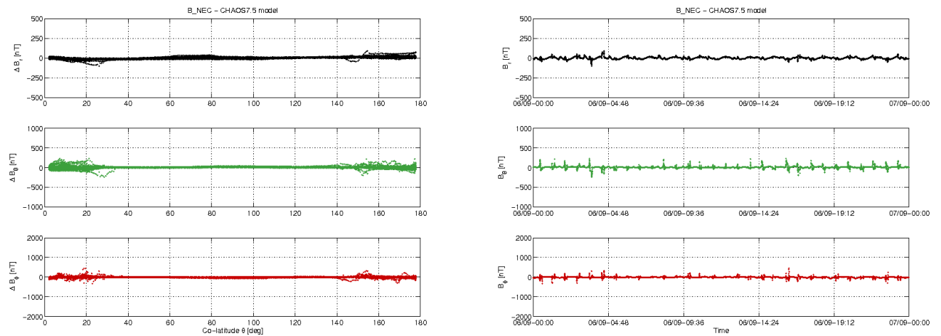
Figure 3-11: S/C B day 06.09: time series of B_{NEC} - B_{Chaos} residuals (right) and B_{NEC} - B_{Chaos} vs colatitude (left).
