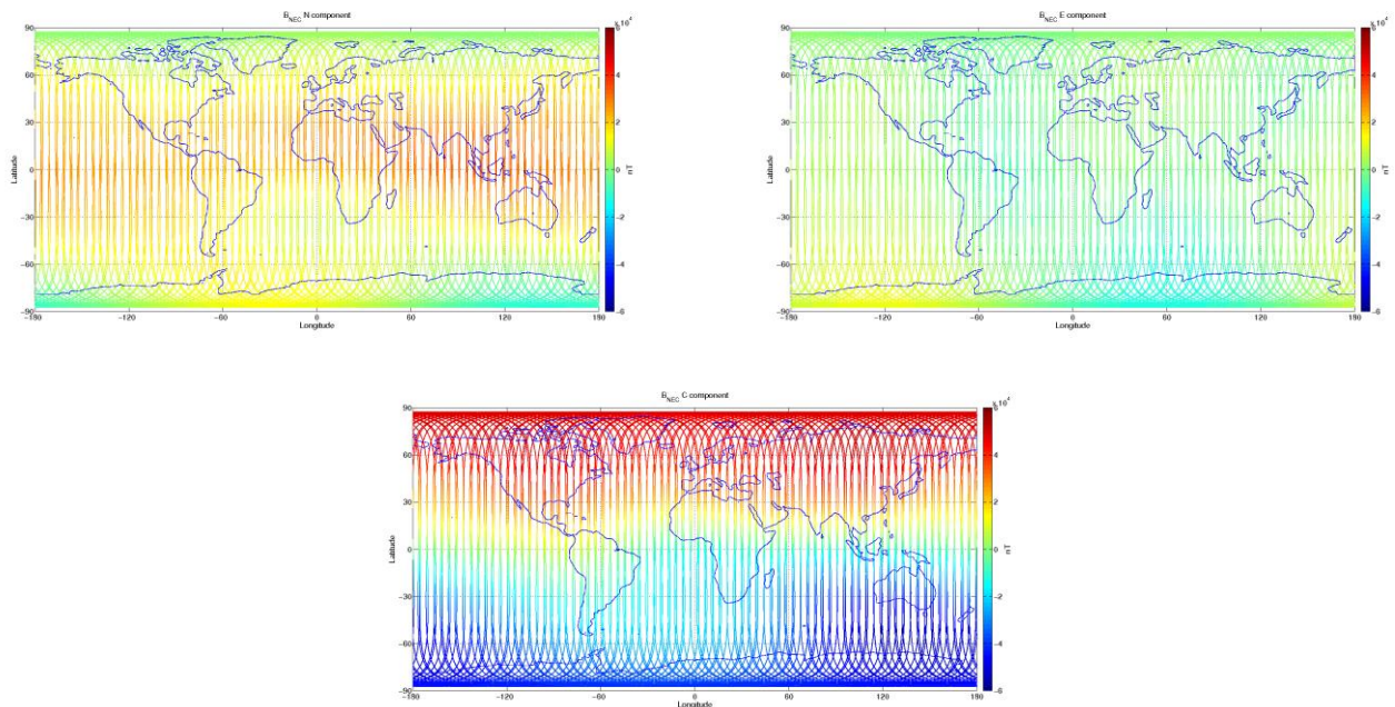
Figure 3-9: S/C C, world map plots of the geomagnetic field and components measured during monitoring period 06/09-12/09. From top to bottom: B_{NEC} components (North, East, and Centre) of magnetic field from VFM measurement.
