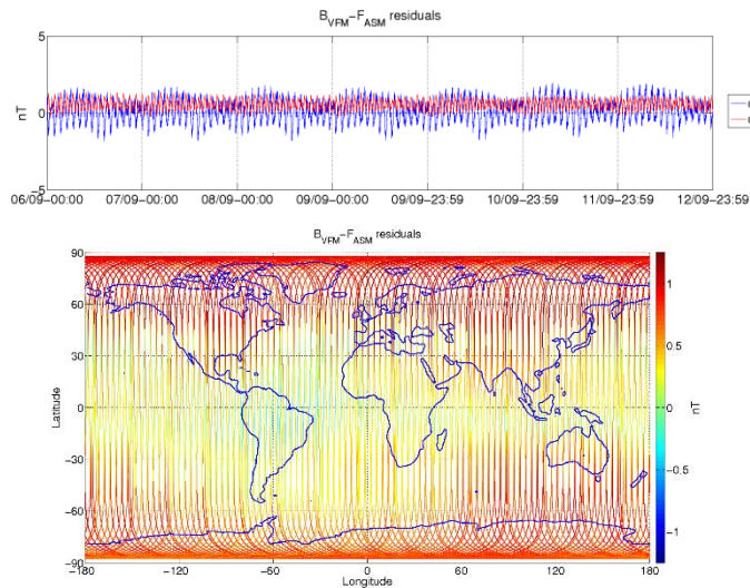
Figure 3-6: ASM-VFM residuals for S/C B, during monitoring period 06/09-12/09. In top figure are plotted: difference between |B_{VFM}| and F_{ASM} (without dB_{Sun} correction) (blue colour), and the residuals with dB_{Sun} corrections (red colour). In bottom figure residuals are presented on the world map.
