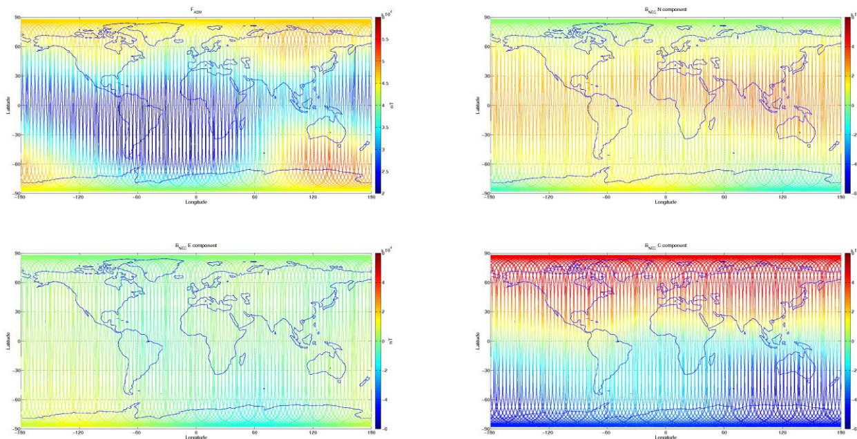
Figure 3-8: S/C B, world map plots of the geomagnetic field and components measured during monitoring period 06/09-12/09. From top to bottom: F-magnetic field from ASM measurement, B_{NEC} components (North, East, and Centre) of magnetic field from VFM measurement.
