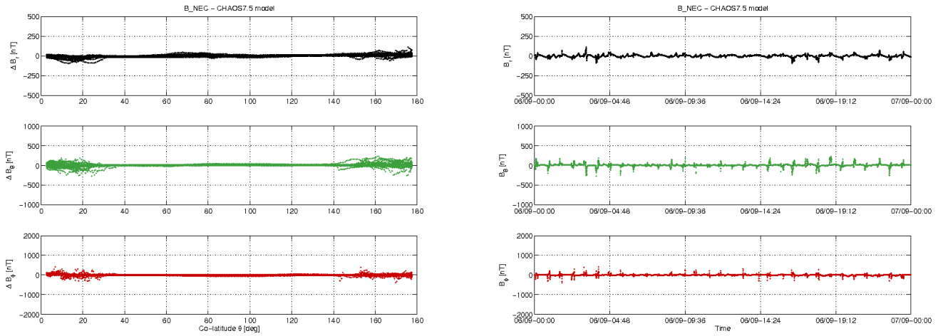
Figure 3-10: S/C A day 06.09: time series of B_{NEC} - B_{Chaos} residuals (right) and B_{NEC} - B_{Chaos} vs colatitude (left).
