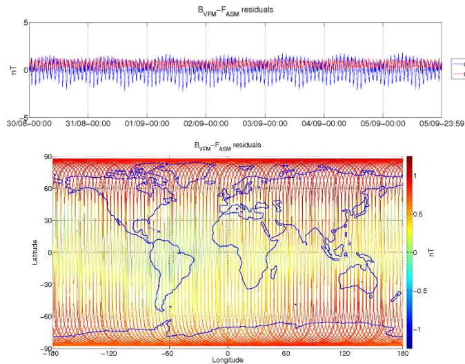
Figure 3-6: ASM-VFM residuals for S/C B, during monitoring period 30/08-05/09. In top figure are plotted: difference between |B_{VFM}| and F_{ASM} (without dB_{Sun} correction) (blue colour), and the residuals with dB_{Sun} corrections (red colour). In bottom figure residuals are presented on the world map.
