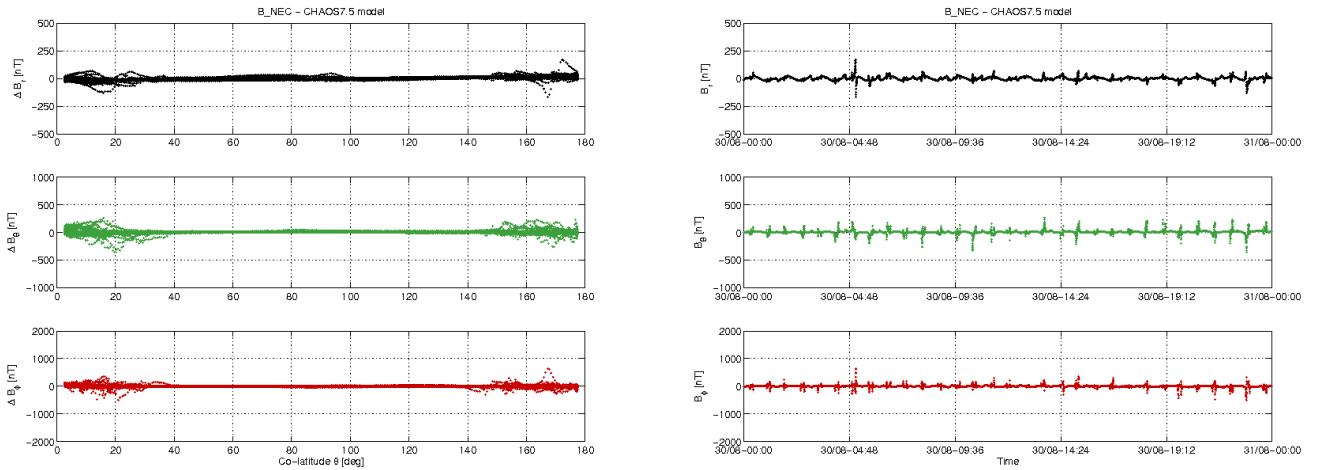
Figure 3-12: S/C C day 30.08: time series of B_{NEC} - B_{Chaos} residuals (right) and B_{NEC} - B_{Chaos} vs colatitude (left)
