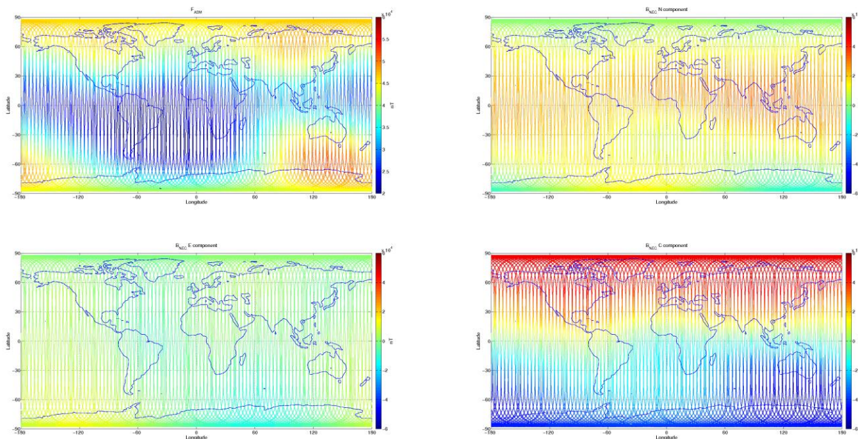
Figure 3-8: S/C B, world map plots of the geomagnetic field and components measured during monitoring period 30/08-05/09. From top to bottom: F-magnetic field from ASM measurement, B_{NEC} components (North, East, and Centre) of magnetic field from VFM measurement.
