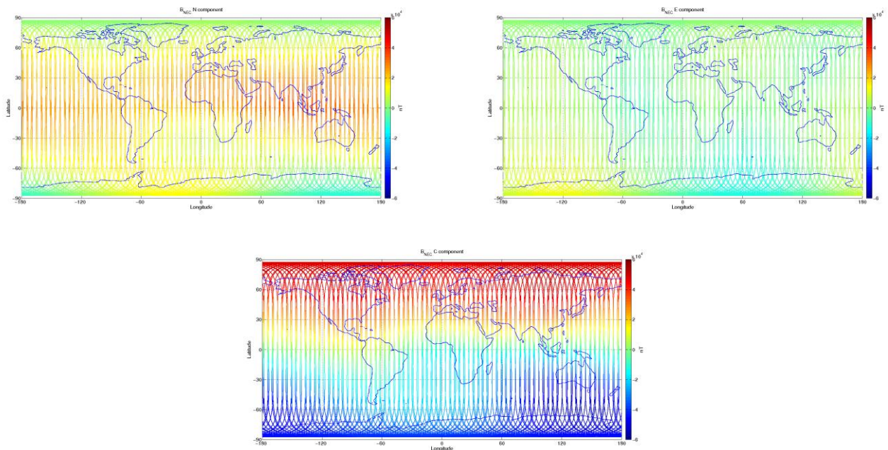
Figure 3-9: S/C C, world map plots of the geomagnetic field and components measured during monitoring period 30/08-05/09. From top to bottom: B_{NEC} components (North, East, and Centre) of magnetic field from VFM measurement.
