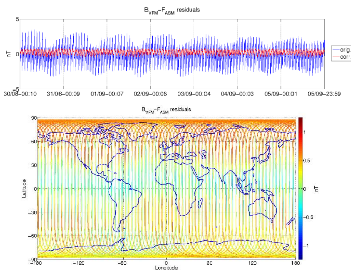
Figure 3-5: ASM-VFM residuals for S/C A, during monitoring period 30/08-05/09. In top figure are plotted: difference between |B_{VFM}| and F_{ASM} (without dB_{Sun} correction) (blue colour), and the residuals with dB_{Sun} corrections (red colour). In bottom figure residuals are presented on the world map.
