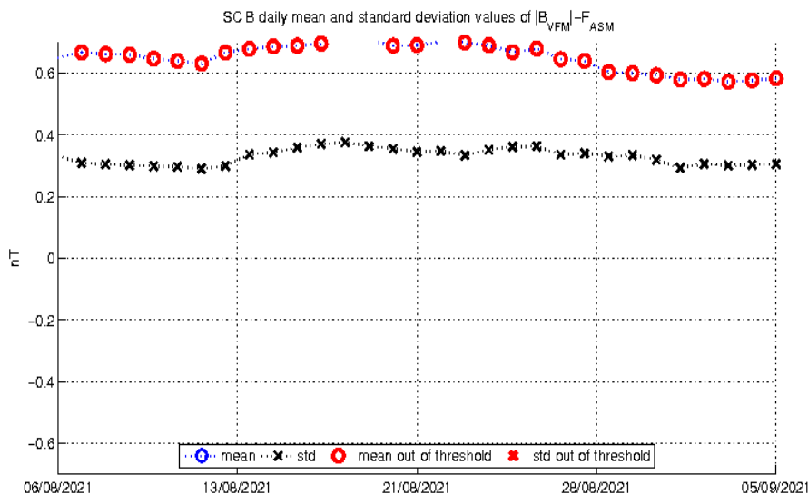
Figure 3-4: Daily mean and standard deviation values of ASM-VFM residuals (defined as dF = |B_{VFM}| - F_{ASM} ) for S/C B.
