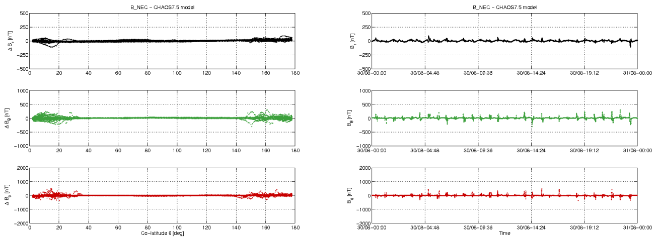
Figure 3-11: S/C B day 30.08: time series of B_{NEC} - B_{Chaos} residuals (right) and B_{NEC} - B_{Chaos} vs colatitude (left).
