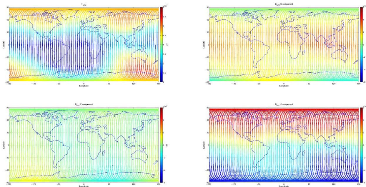
Figure 3-7: S/C A, world map plots of the geomagnetic field and components measured during monitoring period 30/08-05/09. From top to bottom: F-magnetic field from ASM measurement, B_{NEC} components (North, East, and Centre) of magnetic field from VFM measurement.
