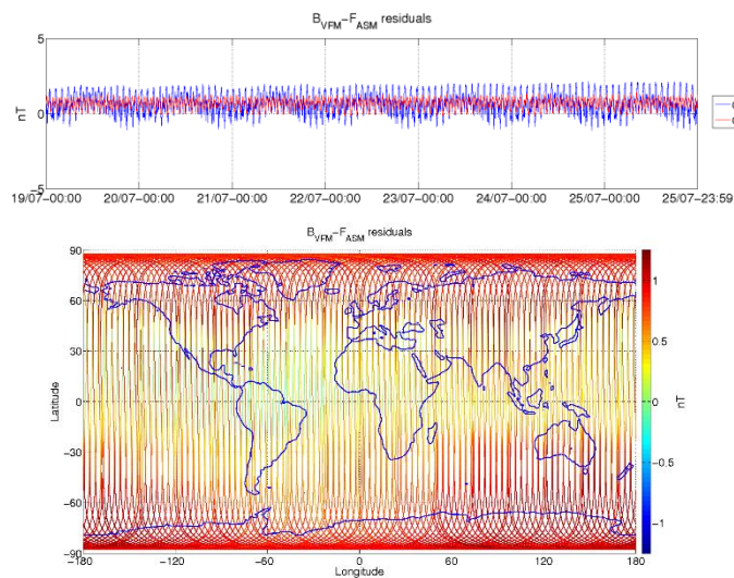
Figure 3-6: ASM-VFM residuals for S/C B, during monitoring period 19/07-25/07. In top figure are plotted: difference between |B_{VFM}| and F_{ASM} (without dB_{Sun} correction) (blue colour), and the residuals with dB_{Sun} corrections (red colour). In bottom figure residuals are presented on the world map.
