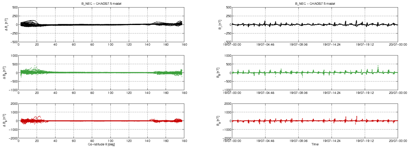
Figure 3-12: S/C C day 19:07: time series of B_{NEC} - B_{Chaos} residuals (right) and B_{NEC} - B_{Chaos} vs colatitude (left)
