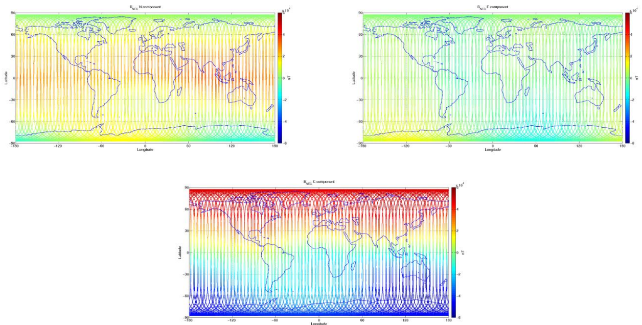
Figure 3-9: S/C C, world map plots of the geomagnetic field and components measured during monitoring period 19/07-25/07. From top to bottom: B_{NEC} components (North, East, and Centre) of magnetic field from VFM measurement.
