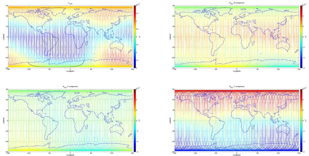
Figure 3-7: S/C A, world map plots of the geomagnetic field and components measured during monitoring period 19/07-25/07. From top to bottom: F-magnetic field from ASM measurement, B_{NEC} components (North, East, and Centre) of magnetic field from VFM measurement.
