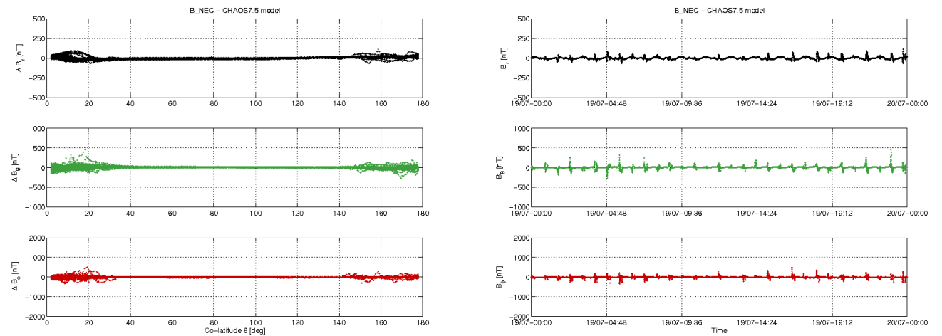
Figure 3-11: S/C B day 19.07: time series of B_{NEC} - B_{Chaos} residuals (right) and B_{NEC} - B_{Chaos} vs colatitude (left).
