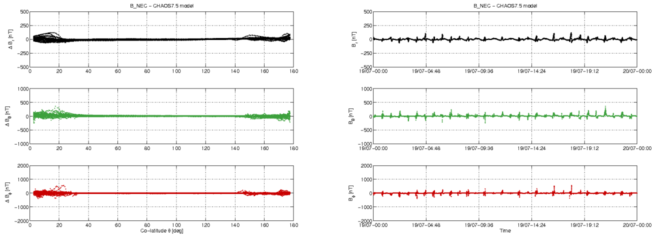
Figure 3-10: S/C A day 19.07: time series of B_{NEC} - B_{Chaos} residuals (right) and B_{NEC} - B_{Chaos} vs colatitude (left).
