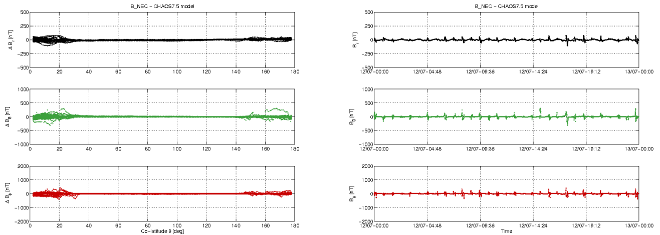
Figure 3-11: S/C B day 12.07: time series of B_{NEC} - B_{Chaos} residuals (right) and B_{NEC} - B_{Chaos} vs colatitude (left).
