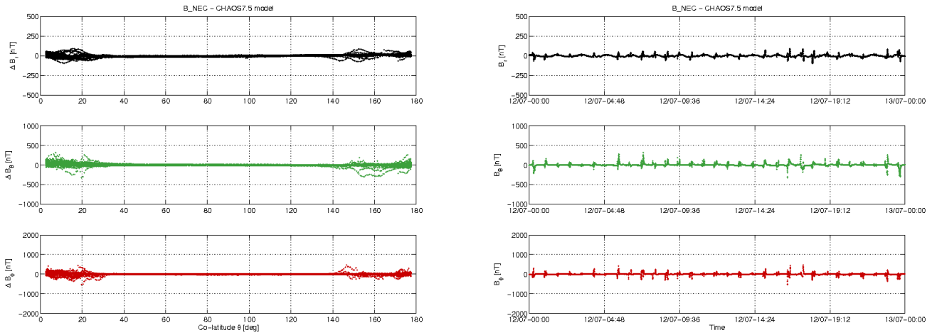
Figure 3-12: S/C C day 12.07: time series of B_{NEC} - B_{Chaos} residuals (right) and B_{NEC} - B_{Chaos} vs colatitude (left)
