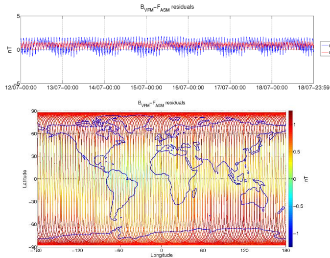
Figure 3-6: ASM-VFM residuals for S/C B, during monitoring period 12/07-18/07. In top figure are plotted: difference between |B_{VFM}| and F_{ASM} (without dB_{Sun} correction) (blue colour), and the residuals with dB_{Sun} corrections (red colour). In bottom figure residuals are presented on the world map.
