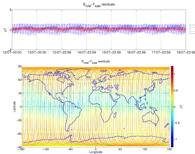
Figure 3-5: ASM-VFM residuals for S/C A, during monitoring period 12/07-18/07. In top figure are plotted: difference between |B_{VFM}| and F_{ASM} (without dB_{Sun} correction) (blue colour), and the residuals with dB_{Sun} corrections (red colour). In bottom figure residuals are presented on the world map.
