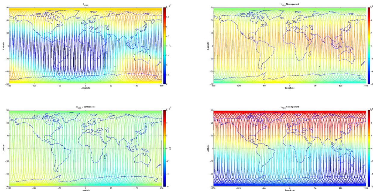
Figure 3-8: S/C B, world map plots of the geomagnetic field and components measured during monitoring period 12/07-18/07. From top to bottom: F-magnetic field from ASM measurement, B_{NEC} components (North, East, and Centre) of magnetic field from VFM measurement.
