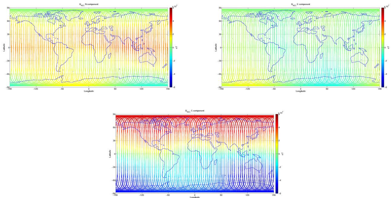
Figure 3-9: S/C C, world map plots of the geomagnetic field and components measured during monitoring period 12/07-18/07. From top to bottom: B_{NEC} components (North, East, and Centre) of magnetic field from VFM measurement.
