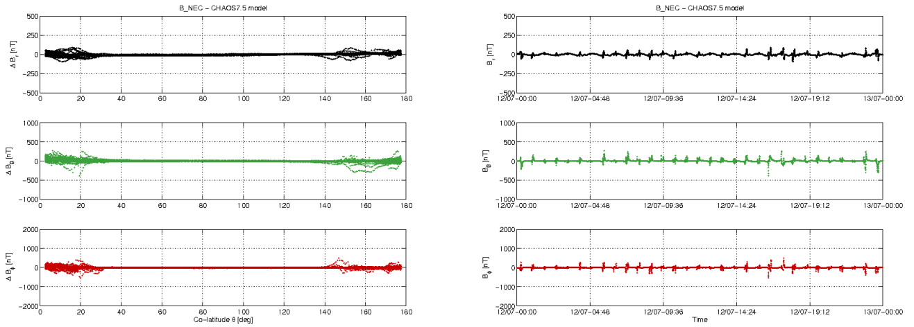
Figure 3-10: S/C A day 12.07: time series of B_{NEC} - B_{Chaos} residuals (right) and B_{NEC} - B_{Chaos} vs colatitude (left).
