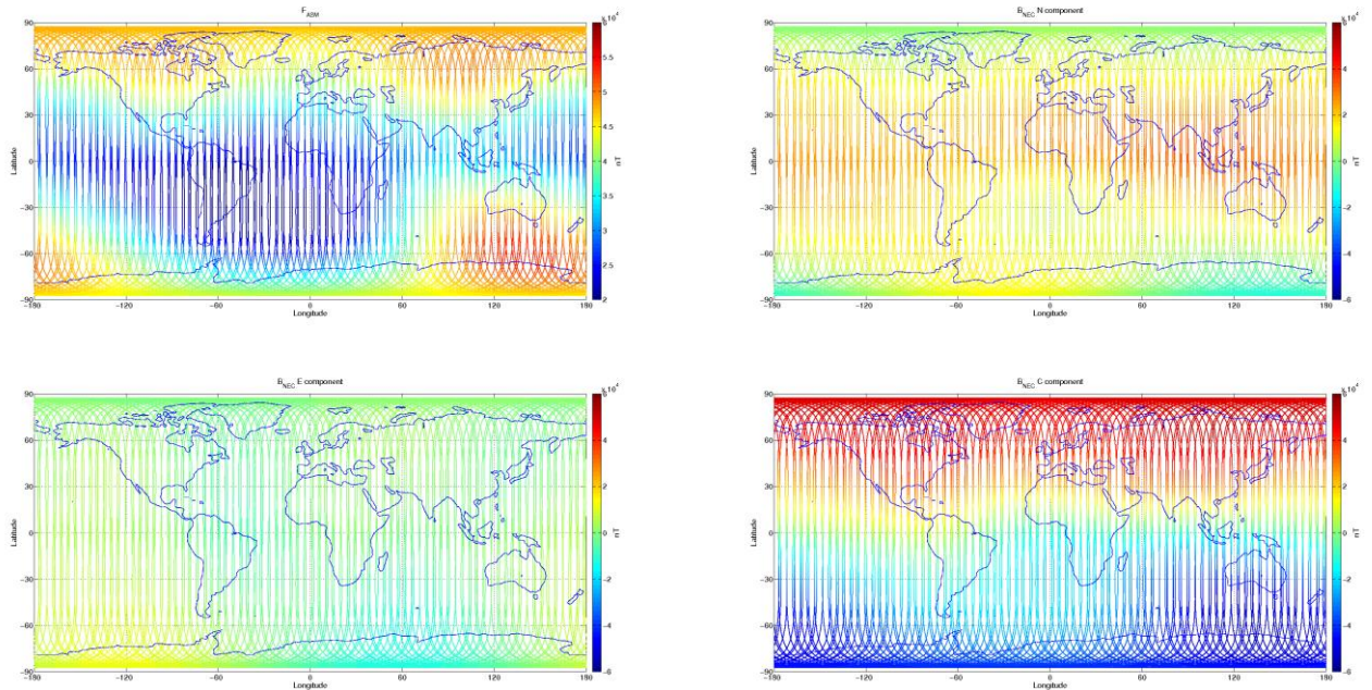
Figure 3-7: S/C A, world map plots of the geomagnetic field and components measured during monitoring period 12/07-18/07. From top to bottom: F-magnetic field from ASM measurement, B_{NEC} components (North, East, and Centre) of magnetic field from VFM measurement.
