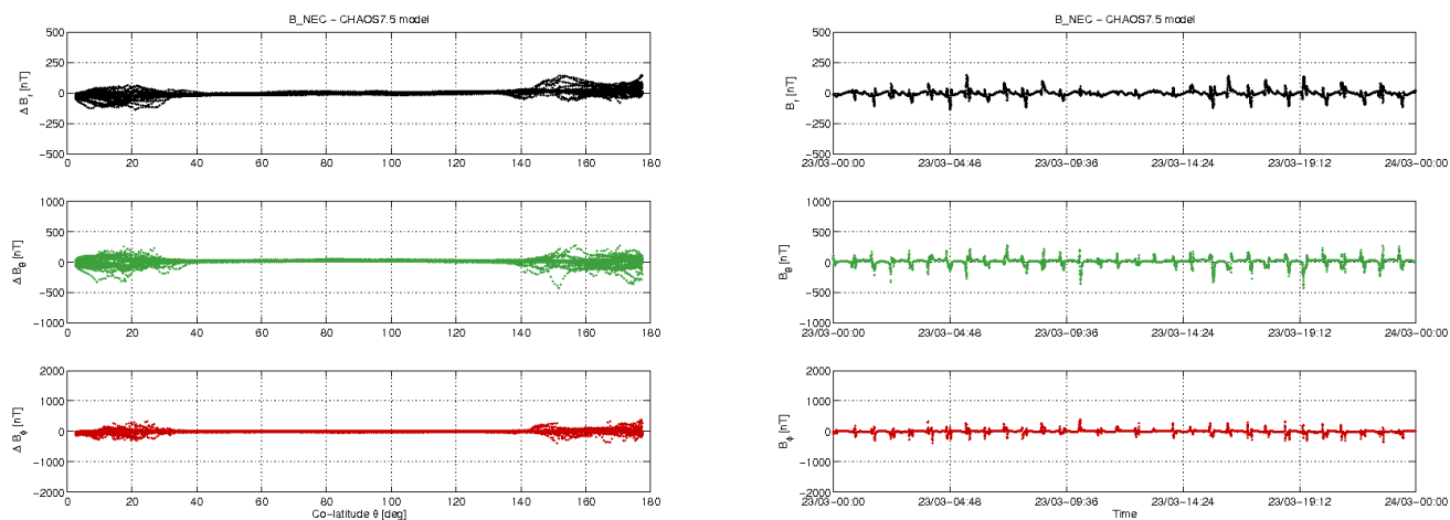
Figure 3-12: S/C C day 23.03: time series of B_{NEC} - B_{Chaos} residuals (right) and B_{NEC} - B_{Chaos} vs colatitude (left)
