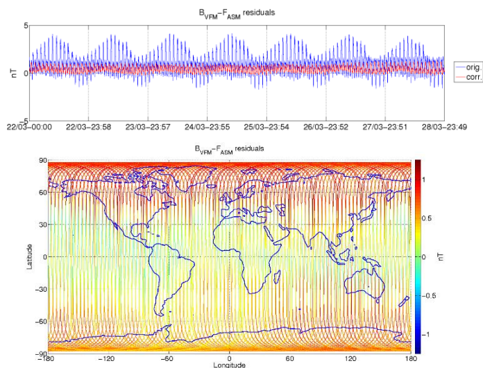
Figure 3-6: ASM-VFM residuals for S/C B, during monitoring period 22/03-28/03. In top figure are plotted: difference between |B_{VFM}| and F_{ASM} (without dB_{Sun} correction) (blue colour), and the residuals with dB_{Sun} corrections (red colour). In bottom figure residuals are presented on the world map.
