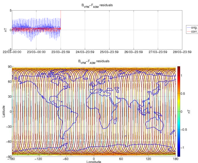
Figure 3-5: ASM-VFM residuals for S/C A, during monitoring period 22/03-28/03. In top figure are plotted: difference between |B_{VFM}| and F_{ASM} (without dB_{Sun} correction) (blue colour), and the residuals with dB_{Sun} corrections (red colour). In bottom figure residuals are presented on the world map.
