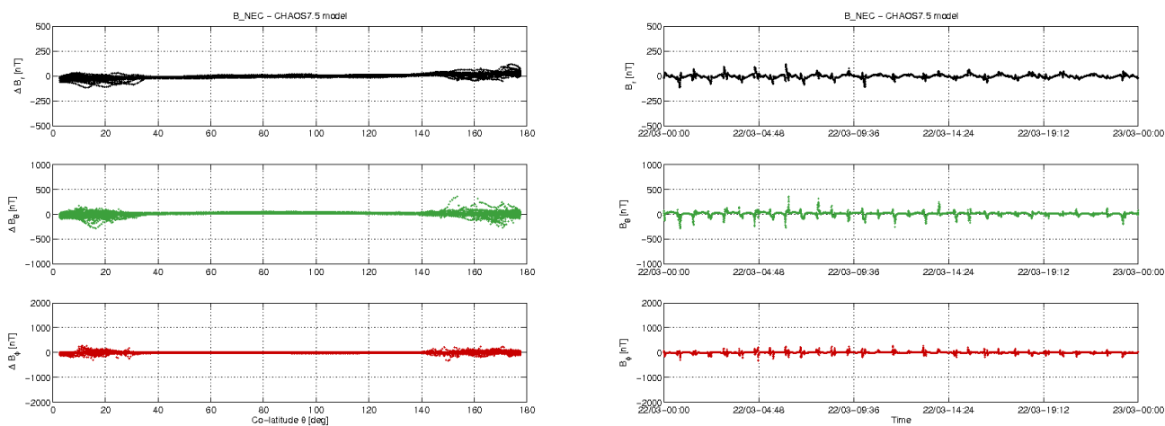
Figure 3-10: S/C A day 22.03: time series of B_{NEC} - B_{Chaos} residuals (right) and B_{NEC} - B_{Chaos} vs colatitude (left).
