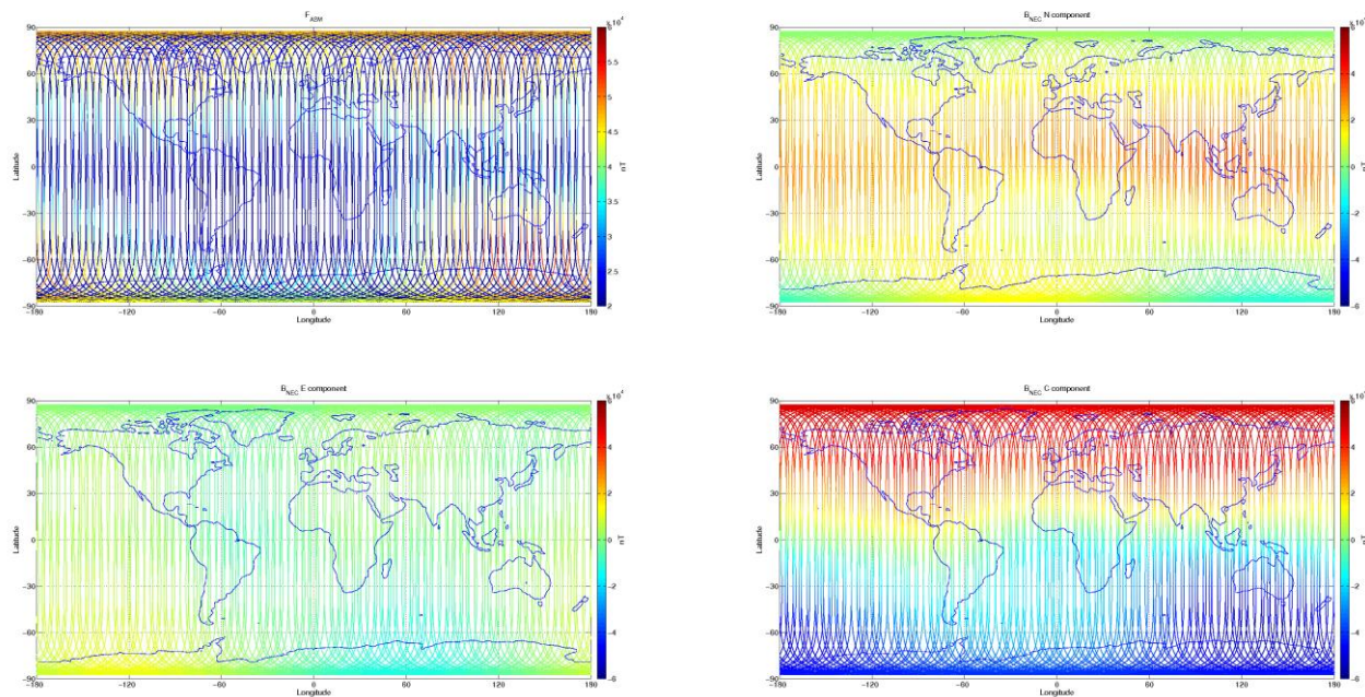
Figure 3-7: S/C A, world map plots of the geomagnetic field and components measured during monitoring period 22/03-28/03. From top to bottom: F-magnetic field from ASM measurement, B_{NEC} components (North, East, and Centre) of magnetic field from VFM measurement.
