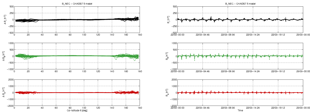
Figure 3-11: S/C B day 22.03 S/C: time series of B_{NEC} - B_{Chaos} residuals (right) and B_{NEC} - B_{Chaos} vs colatitude (left).
