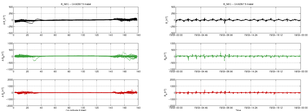
Figure 3-11: S/C B day 15.03: time series of B_{NEC} - B_{Chaos} residuals (right) and B_{NEC} - B_{Chaos} vs colatitude (left).
