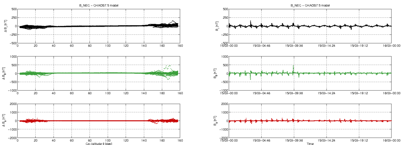
Figure 3-10: S/C A day 15.03: time series of B_{NEC} - B_{Chaos} residuals (right) and B_{NEC} - B_{Chaos} vs colatitude (left).
