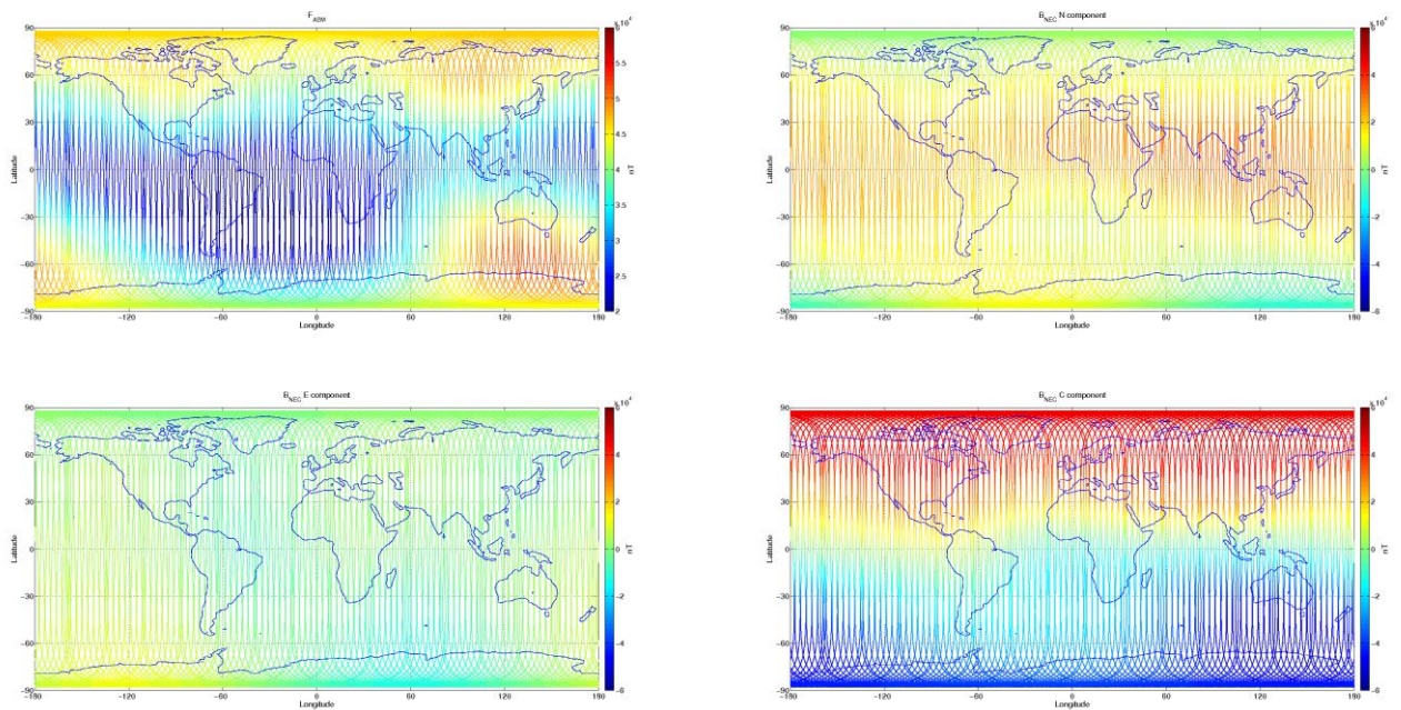
Figure 3-8: S/C B, world map plots of the geomagnetic field and components measured during monitoring period 15/03-21/03. From top to bottom: F-magnetic field from ASM measurement, B_{NEC} components (North, East, and Centre) of magnetic field from VFM measurement.
