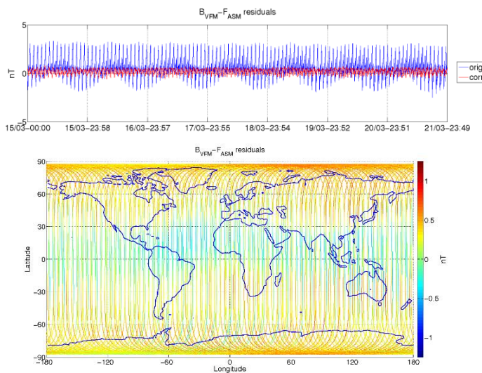
Figure 3-5: ASM-VFM residuals for S/C A, during monitoring period 15/03-21/03. In top figure are plotted: difference between |B_{VFM}| and F_{ASM} (without dB_{Sun} correction) (blue colour), and the residuals with dB_{Sun} corrections (red colour). In bottom figure residuals are presented on the world map.
