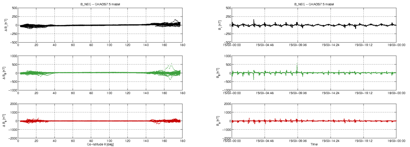
Figure 3-12: S/C C day 1503: time series of B_{NEC} - B_{Chaos} residuals (right) and B_{NEC} - B_{Chaos} vs colatitude (left)
