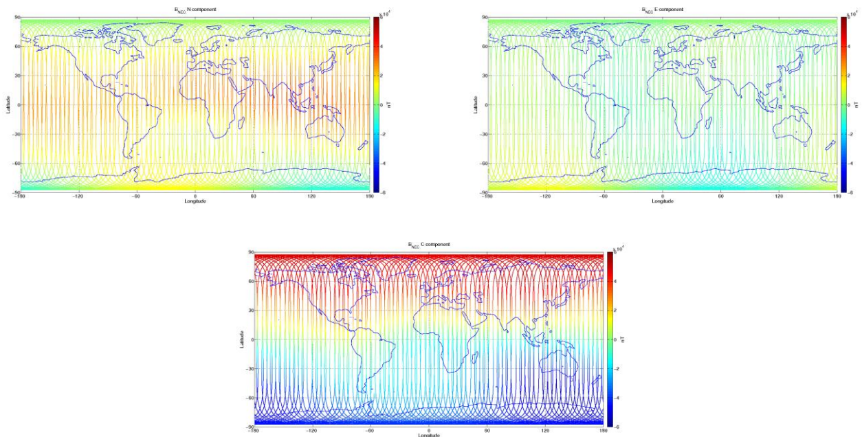
Figure 3-9: S/C C, world map plots of the geomagnetic field and components measured during monitoring period 15/03-21/03. From top to bottom: B_{NEC} components (North, East, and Centre) of magnetic field from VFM measurement.
