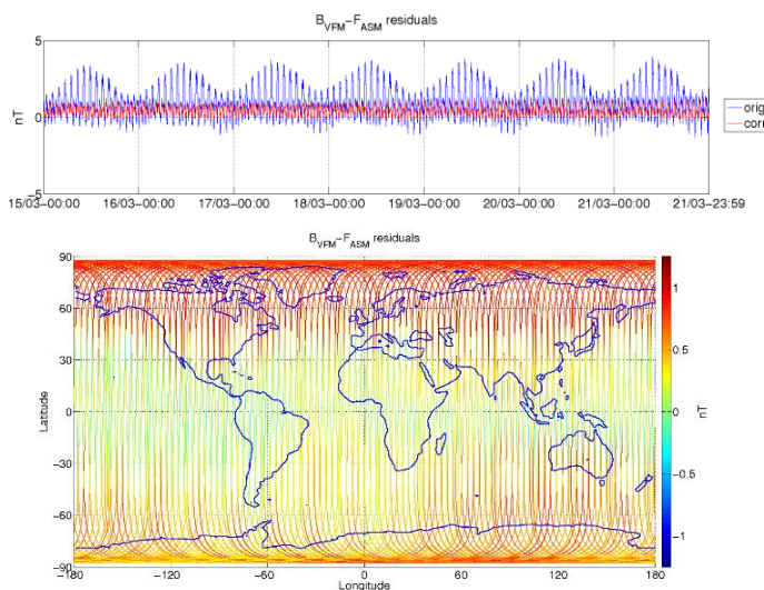
Figure 3-6: ASM-VFM residuals for S/C B, during monitoring period 15/03-21/03. In top figure are plotted: difference between |B_{VFM}| and F_{ASM} (without dB_{Sun} correction) (blue colour), and the residuals with dB_{Sun} corrections (red colour). In bottom figure residuals are presented on the world map.
