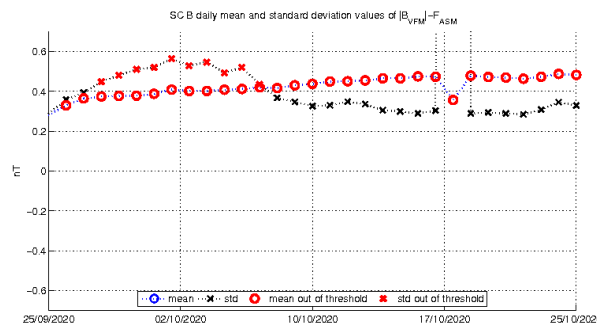
Figure 3-3: Daily mean and standard deviation values of ASM-VFM residuals (defined as dF = |B_{VFM}| - F_{ASM} ) for S/C B.
