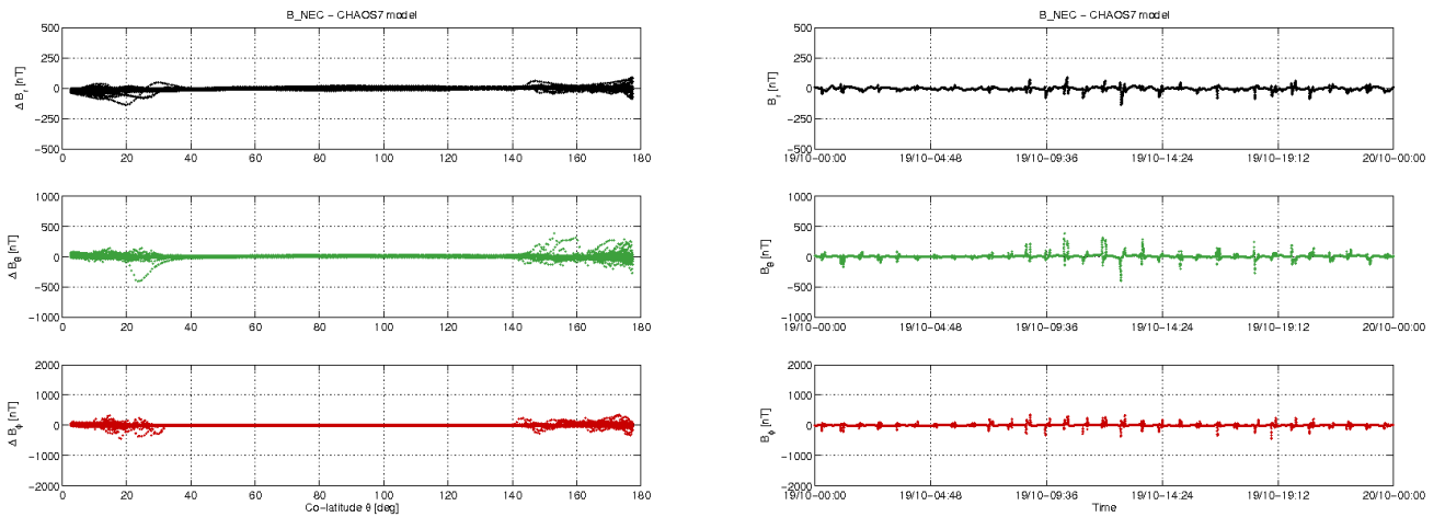
Figure 3-8: S/C C day 19.10: time series of B_{NEC} - B_{Chaos} residuals (right) and B_{NEC} - B_{Chaos} vs colatitude (left).
