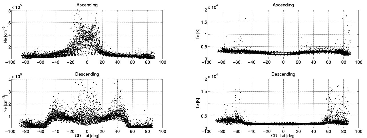
Figure 3-11: The panels shown the electron density (left) and temperature (right) profile as a function of QD Latitudes for the last week of operation. The analysis is made separately for ascending (upper panels) and descending (bottom panels) orbits.
