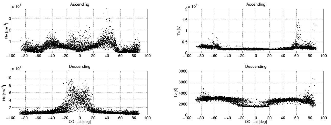
Figure 3-12: The panels shown the electron density (left) and temperature (right) profile as a function of QD Latitudes for the last week of operation. The analysis is made separately for ascending (upper panels) and descending (bottom panels) orbits.
