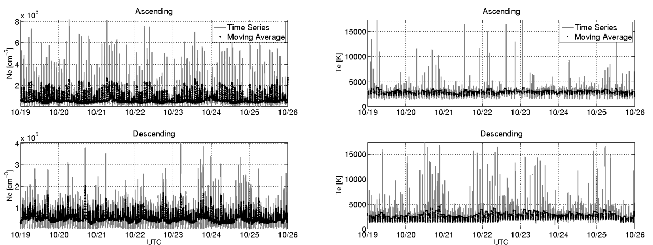
Figure 3-9: The panels show the electron density (left) and temperature (right) weekly time series (grey lines) together with the 20 min moving windows average (black lines). The analysis is made separately for ascending (upper panels) and descending (bottom panels) orbits. The average magnetic local time during the week is 2 a.m. for descending phase and 2 p.m. for ascending phase.
