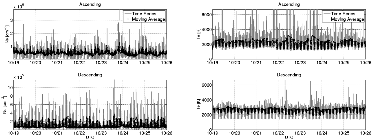
Figure 3-10: The panels show the electron density (left) and temperature (right) weekly time series (grey lines) together with the 20 min moving windows average (black lines). The analysis is made separately for ascending (upper panels) and descending (bottom panels) orbits. The average magnetic local time during the week is 4 a.m. for ascending phase and 4 p.m. for descending phase.
