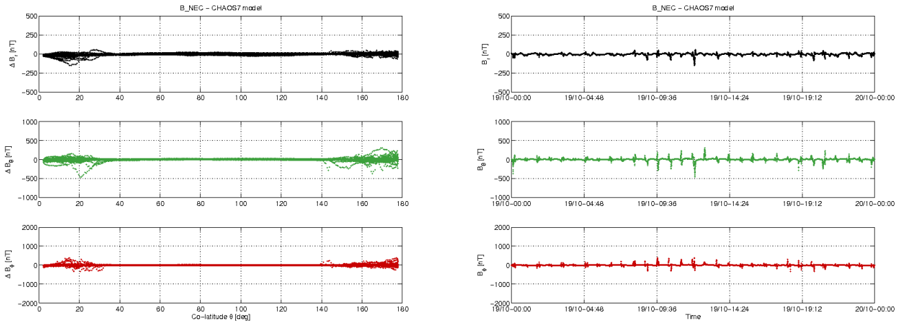
Figure 3-7: S/C B day 19.10: time series of B_{NEC} - B_{Chaos} residuals (right) and B_{NEC} - B_{Chaos} vs colatitude (left).
