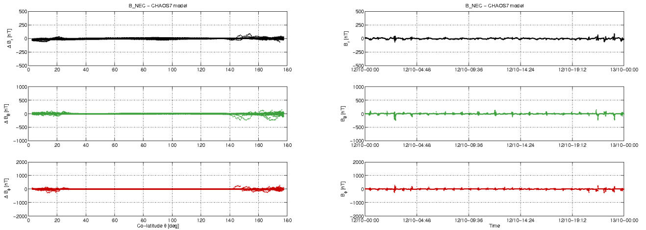
Figure 3-12: S/C C day 12.10: time series of B_{NEC} - B_{Chaos} residuals (right) and B_{NEC} - B_{Chaos} vs colatitude (left).
