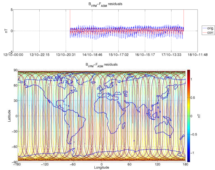
Figure 3-5: ASM-VFM residuals for S/C A, during monitoring period 12/10-18/10. In top figure are plotted: difference between |B_{VFM}| and F_{ASM} (without dB_{Sun} correction) (blue colour), and the residuals with dB_{Sun} corrections (red colour). In bottom figure residuals are presented on the world map.
