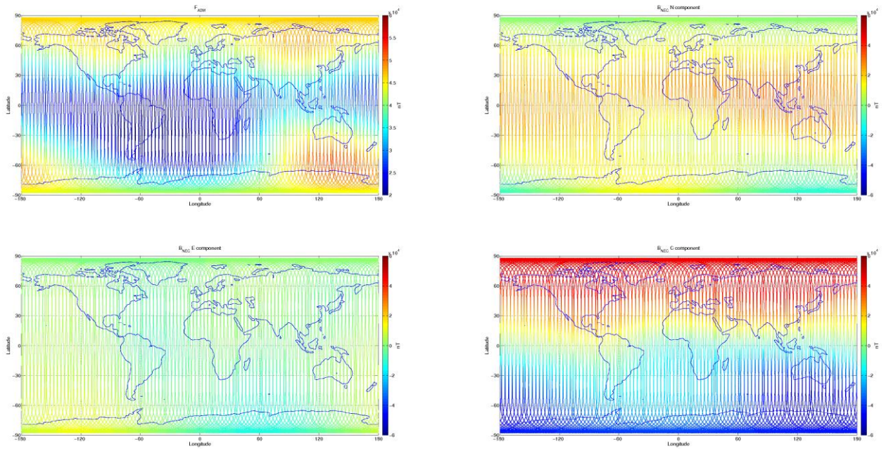
Figure 3-8: S/C B, world map plots of the geomagnetic field and components measured during monitoring period 12/10-18/10. From top to bottom: F-magnetic field from ASM measurement, B_{NEC} components (North, East, and Centre) of magnetic field from VFM measurement.
