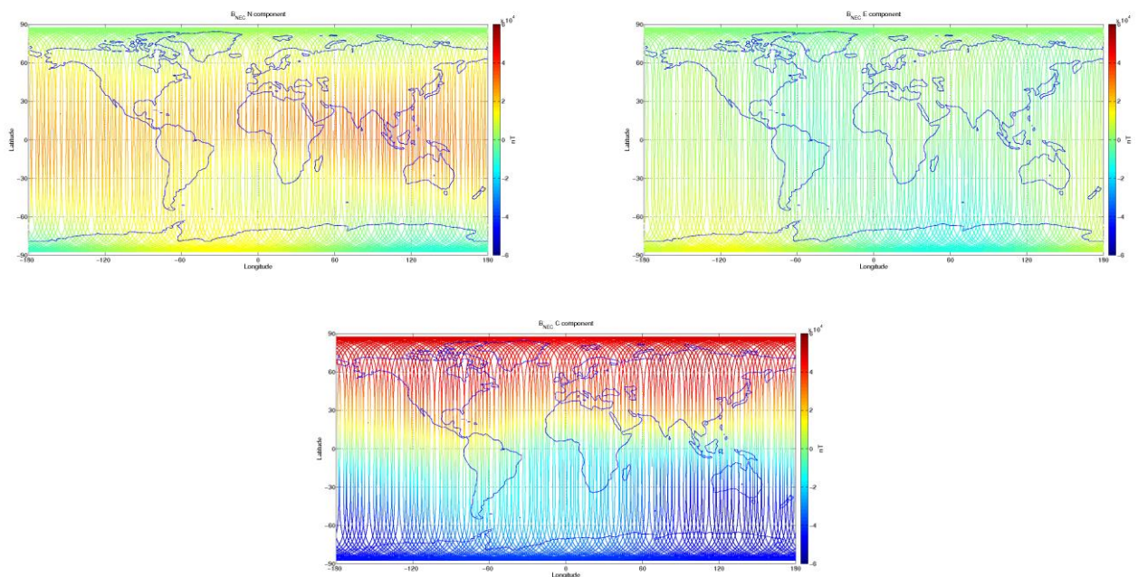
Figure 3-9: S/C C, world map plots of the geomagnetic field and components measured during monitoring period 12/10-18/10. From top to bottom: B_{NEC} components (North, East, and Centre) of magnetic field from VFM measurement.
