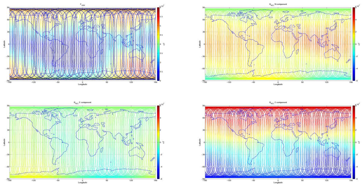
Figure 3-7: S/C A, world map plots of the geomagnetic field and components measured during monitoring period 12/10-18/10. From top to bottom: F-magnetic field from ASM measurement, B_{NEC} components (North, East, and Centre) of magnetic field from VFM measurement.
