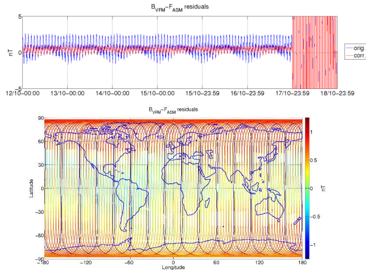
Figure 3-6: ASM-VFM residuals for S/C B, during monitoring period 12/10-18/10. In top figure are plotted: difference between |B_{VFM}| and F_{ASM} (without dB_{Sun} correction) (blue colour), and the residuals with dB_{Sun} corrections (red colour). In bottom figure residuals are presented on the world map.
