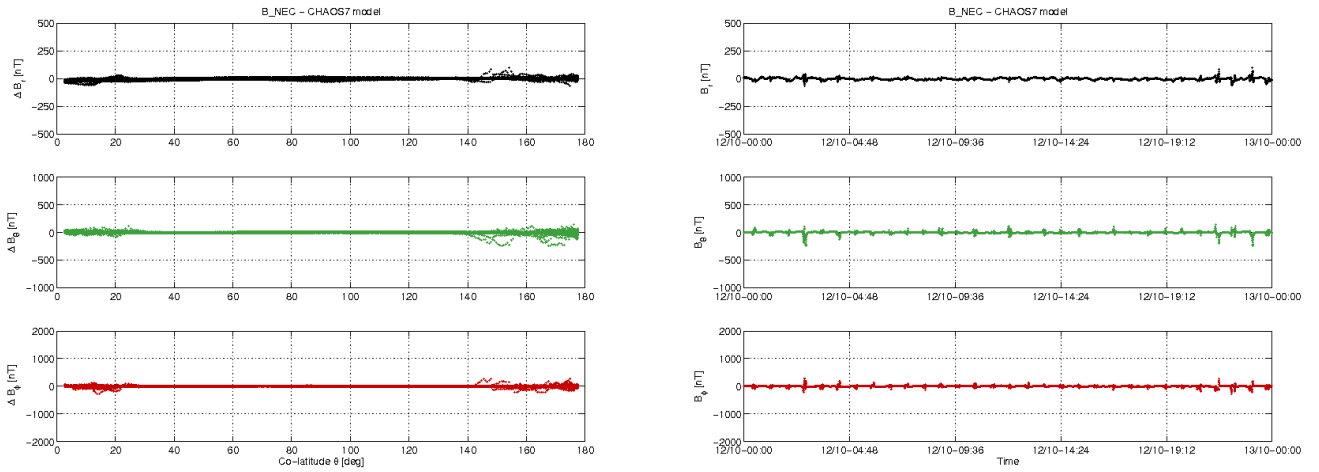
Figure 3-10: S/C A day 12.10: time series of B_{NEC} - B_{Chaos} residuals (right) and B_{NEC} - B_{Chaos} vs colatitude (left).
