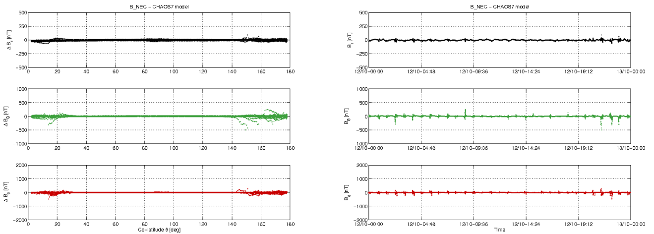
Figure 3-11: S/C B day 12.10: time series of B_{NEC} - B_{Chaos} residuals (right) and B_{NEC} - B_{Chaos} vs colatitude (left).
