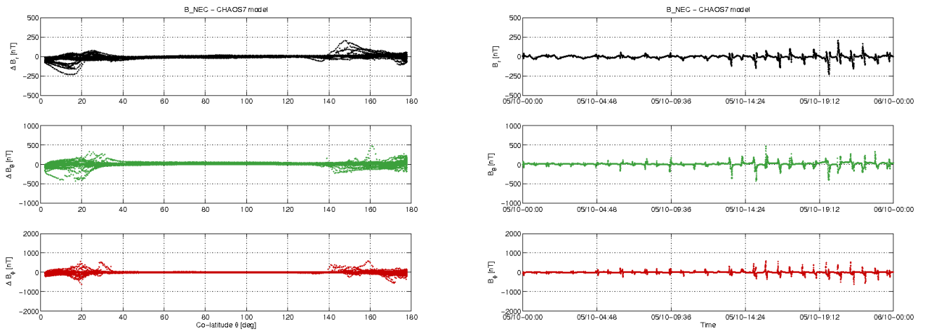
Figure 3-11: S/C B day 05.10: time series of B_{NEC} - B_{Chaos} residuals (right) and B_{NEC} - B_{Chaos} vs colatitude (left).
