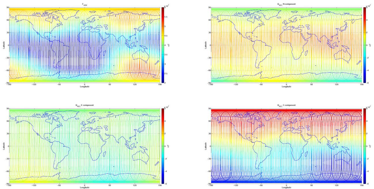
Figure 3-8: S/C B, world map plots of the geomagnetic field and components measured during monitoring period 05/10-11/10. From top to bottom: F-magnetic field from ASM measurement, B_{NEC} components (North, East, and Centre) of magnetic field from VFM measurement.
