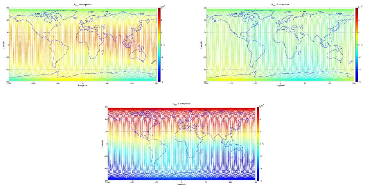
Figure 3-9: S/C C, world map plots of the geomagnetic field and components measured during monitoring period 05/10-11/10. From top to bottom: B_{NEC} components (North, East, and Centre) of magnetic field from VFM measurement.
