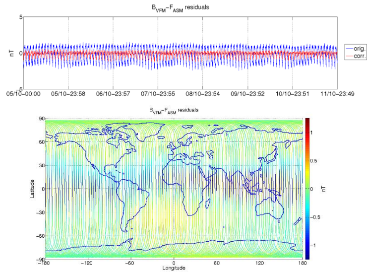
Figure 3-5: ASM-VFM residuals for S/C A, during monitoring period 05/10-11/10. In top figure are plotted: difference between |B_{VFM}| and F_{ASM} (without dB_{Sun} correction) (blue colour), and the residuals with dB_{Sun} corrections (red colour). In bottom figure residuals are presented on the world map.
