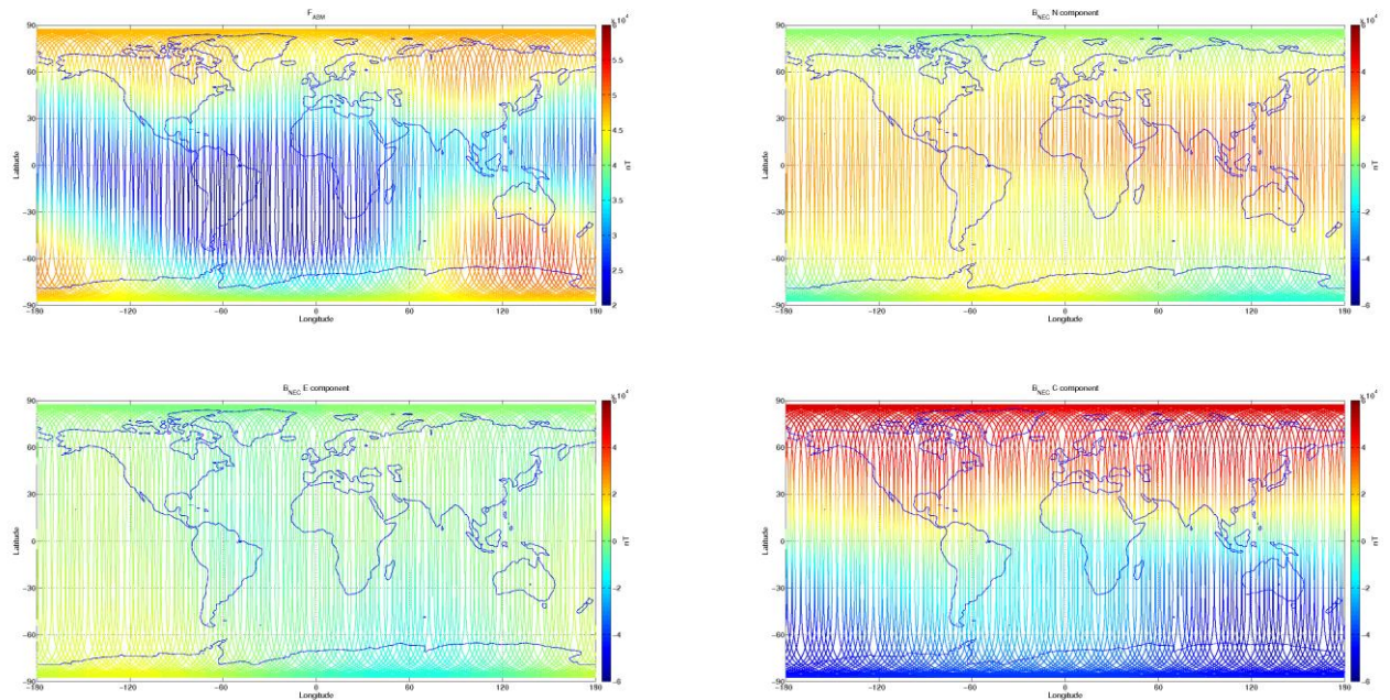
Figure 3-7: S/C A, world map plots of the geomagnetic field and components measured during monitoring period 05/10-11/10. From top to bottom: F-magnetic field from ASM measurement, B_{NEC} components (North, East, and Centre) of magnetic field from VFM measurement.
