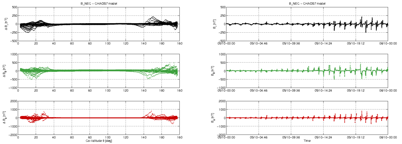
Figure 3-10: S/C A day 05.10: time series of B_{NEC} - B_{Chaos} residuals (right) and B_{NEC} - B_{Chaos} vs colatitude (left).
