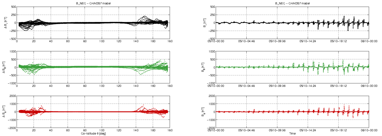
Figure 3-12: S/C C day 05.10: time series of B_{NEC} - B_{Chaos} residuals (right) and B_{NEC} - B_{Chaos} vs colatitude (left).
