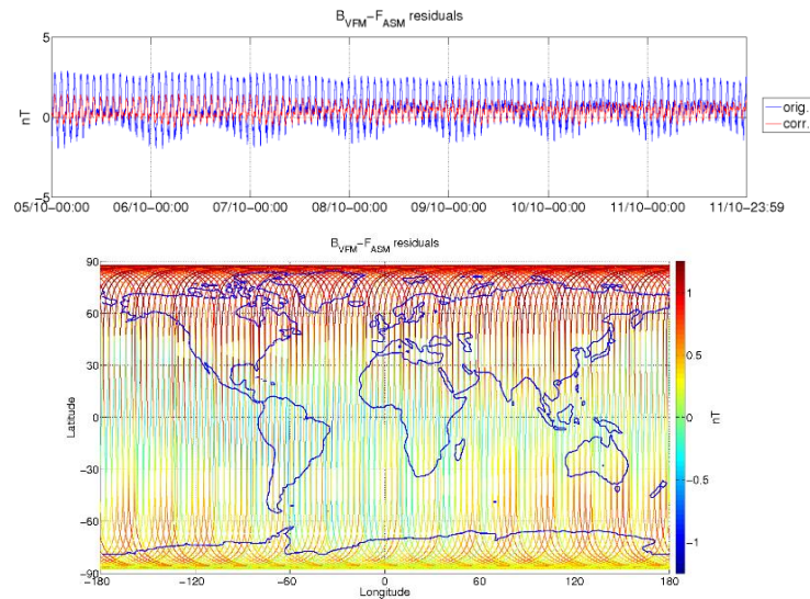
Figure 3-6: ASM-VFM residuals for S/C B, during monitoring period 05/10-11/10. In top figure are plotted: difference between |B_{VFM}| and F_{ASM} (without dB_{Sun} correction) (blue colour), and the residuals with dB_{Sun} corrections (red colour). In bottom figure residuals are presented on the world map.
