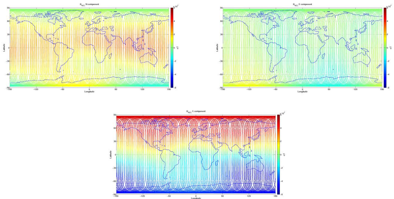
Figure 3-9: S/C C, world map plots of the geomagnetic field and components measured during monitoring period 28/09-04/10. From top to bottom: B_{NEC} components (North, East, and Centre) of magnetic field from VFM measurement.
