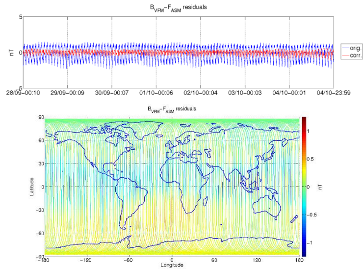
Figure 3-5: ASM-VFM residuals for S/C A, during monitoring period 28/09-04/10. In top figure are plotted: difference between |B_{VFM}| and F_{ASM} (without dB_{Sun} correction) (blue colour), and the residuals with dB_{Sun} corrections (red colour). In bottom figure residuals are presented on the world map.
