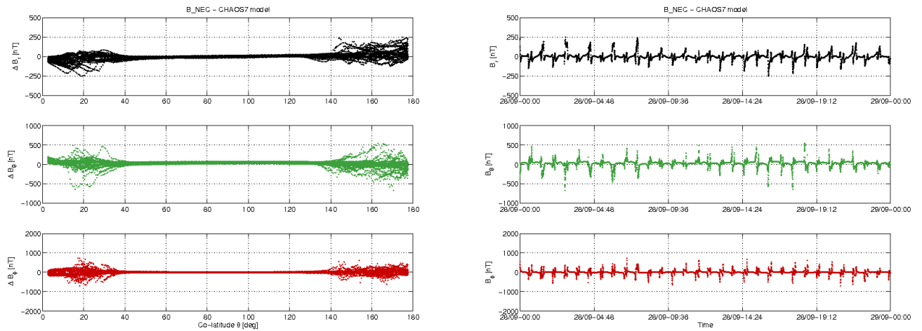
Figure 3-10: S/C A day 28.09: time series of B_{NEC} - B_{Chaos} residuals (right) and B_{NEC} - B_{Chaos} vs colatitude (left).
