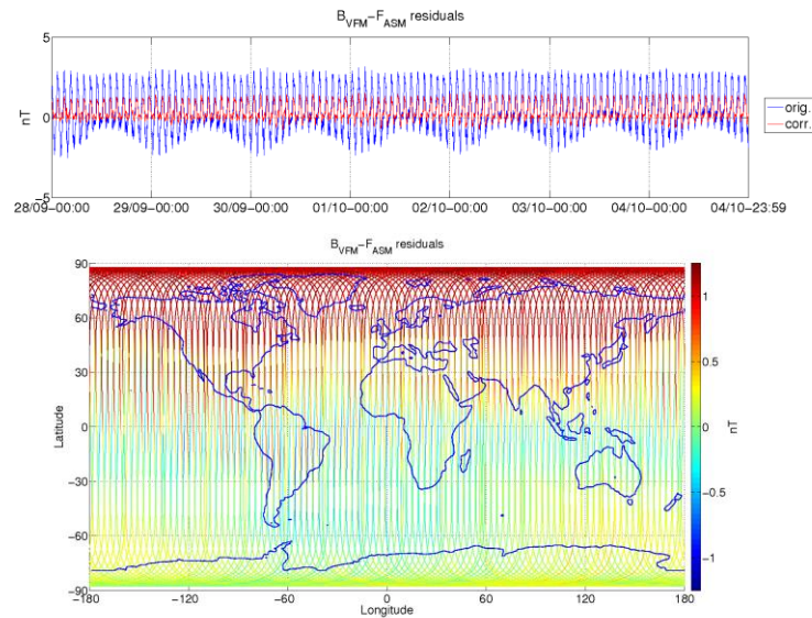
Figure 3-6: ASM-VFM residuals for S/C B, during monitoring period 28/09-04/10. In top figure are plotted: difference between |B_{VFM}| and F_{ASM} (without dB_{Sun} correction) (blue colour), and the residuals with dB_{Sun} corrections (red colour). In bottom figure residuals are presented on the world map.
