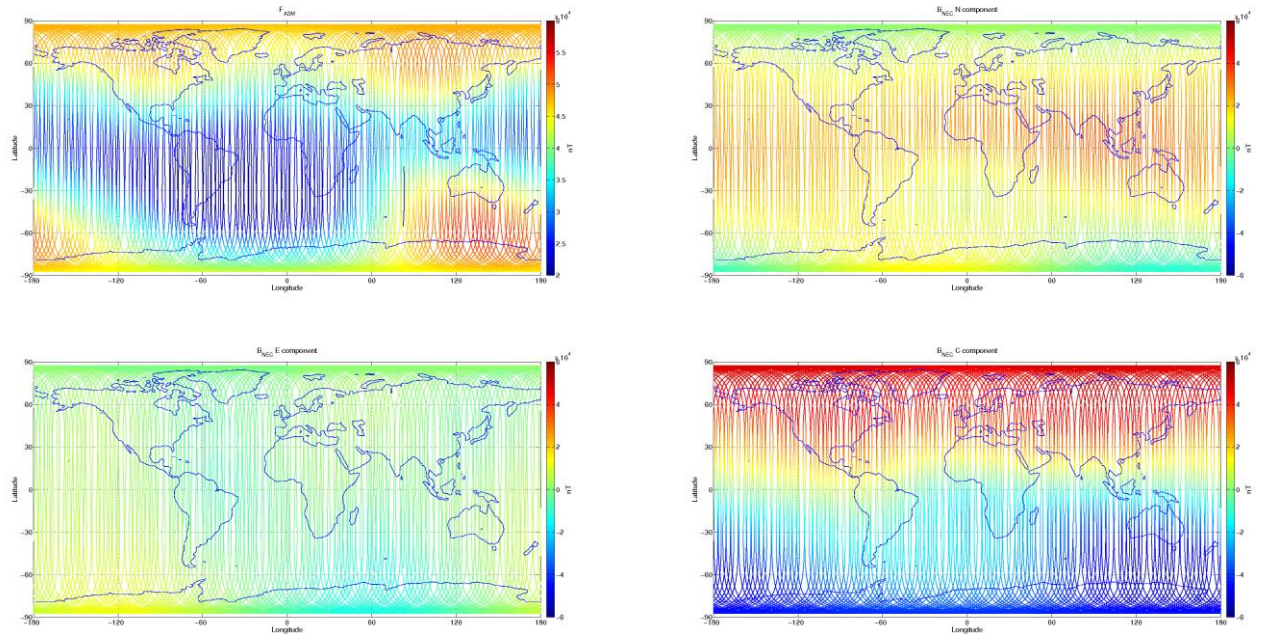
Figure 3-7: S/C A, world map plots of the geomagnetic field and components measured during monitoring period 28/09-04/10. From top to bottom: F-magnetic field from ASM measurement, B_{NEC} components (North, East, and Centre) of magnetic field from VFM measurement.
