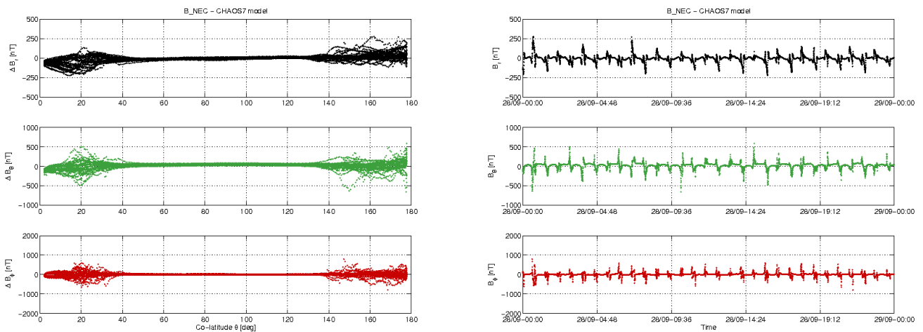
Figure 3-11: S/C B day 28.09: time series of B_{NEC} - B_{Chaos} residuals (right) and B_{NEC} - B_{Chaos} vs colatitude (left).
