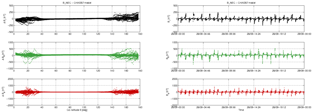
Figure 3-12: S/C C day 28.09: time series of B_{NEC} - B_{Chaos} residuals (right) and B_{NEC} - B_{Chaos} vs colatitude (left).
