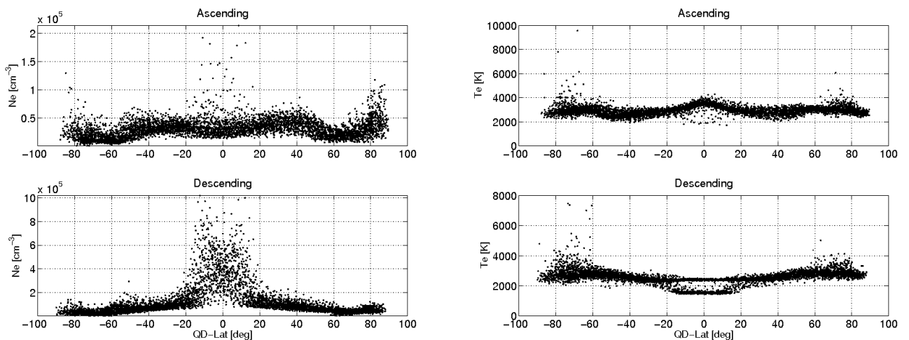
Figure 3-15: The panels shown the electron density (left) and temperature (right) profile as a function of QD Latitudes for the last week of operation. The analysis is made separately for ascending (upper panels) and descending (bottom panels) orbits.
