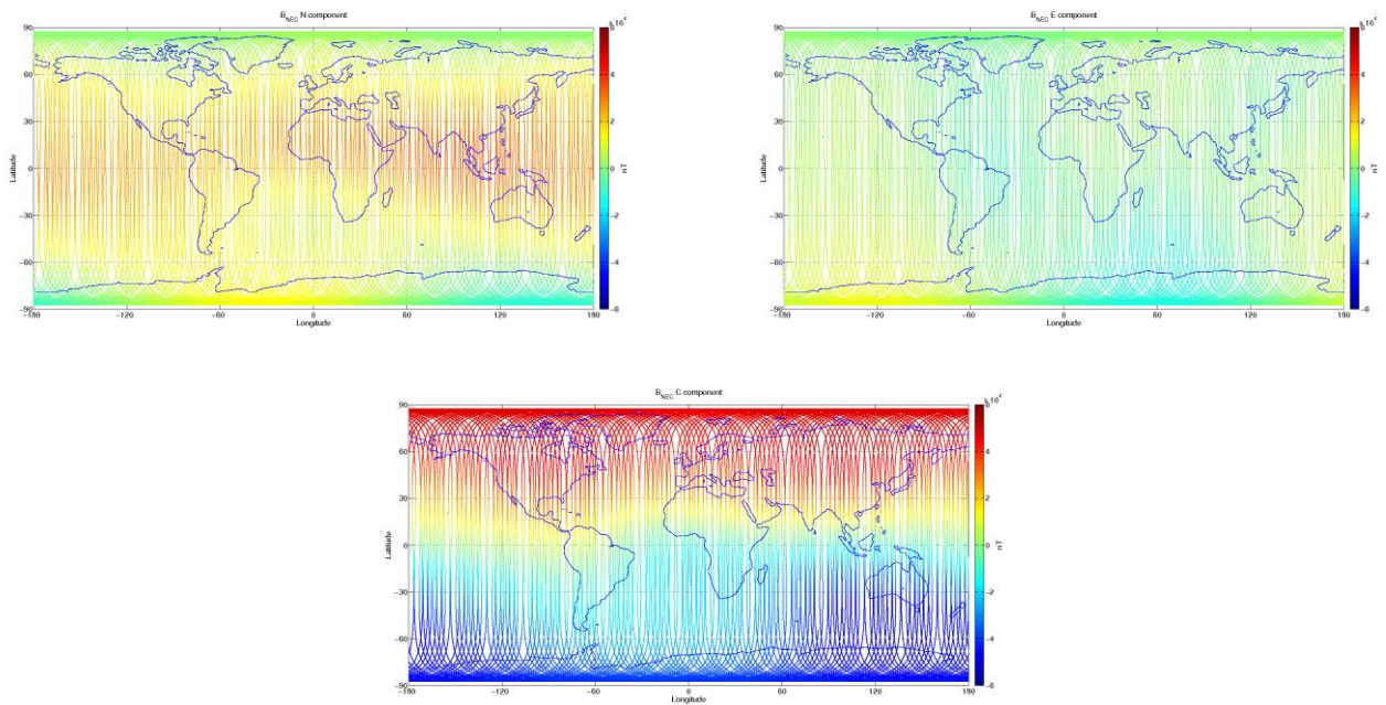
Figure 3-8: S/C C, world map plots of the geomagnetic field and components measured during monitoring period 21/09-27/09. From top to bottom: B_{NEC} components (North, East, and Centre) of magnetic field from VFM measurement.
