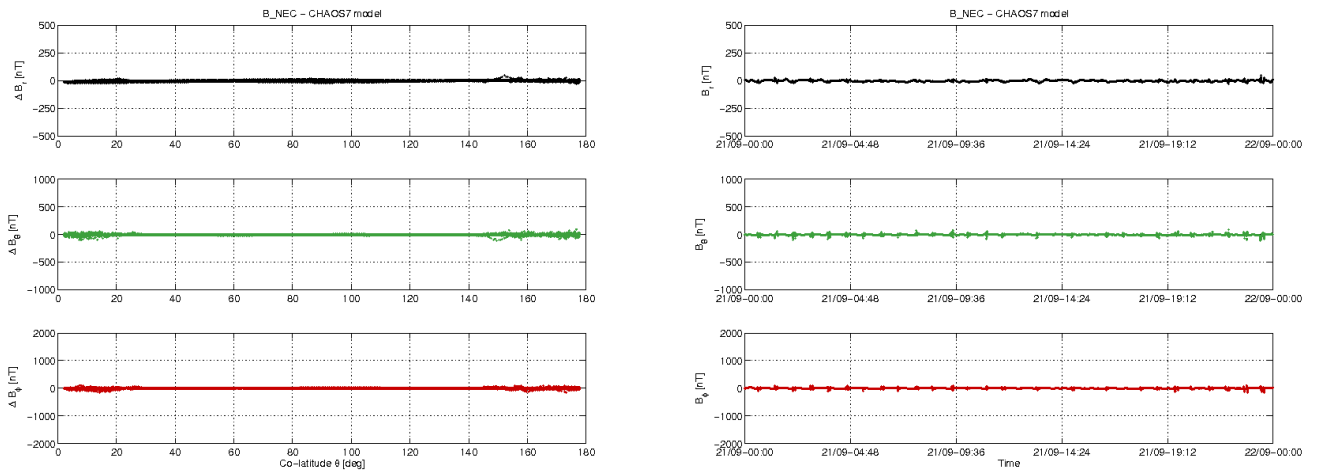
Figure 3-10: S/C B day 21.09: time series of B_{NEC} - B_{Chaos} residuals (right) and B_{NEC} - B_{Chaos} vs colatitude (left).
