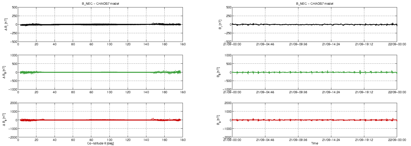
Figure 3-11: S/C C day 21.09: time series of B_{NEC} - B_{Chaos} residuals (right) and B_{NEC} - B_{Chaos} vs colatitude (left).
