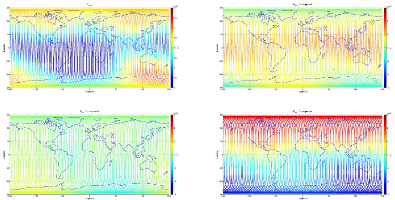
Figure 3-7: S/C B, world map plots of the geomagnetic field and components measured during monitoring period 21/09-27/09. From top to bottom: F-magnetic field from ASM measurement, B_{NEC} components (North, East, and Centre) of magnetic field from VFM measurement.
