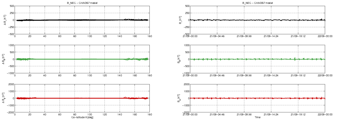
Figure 3-9: S/C A day 21.09: time series of B_{NEC} - B_{Chaos} residuals (right) and B_{NEC} - B_{Chaos} vs colatitude (left).
