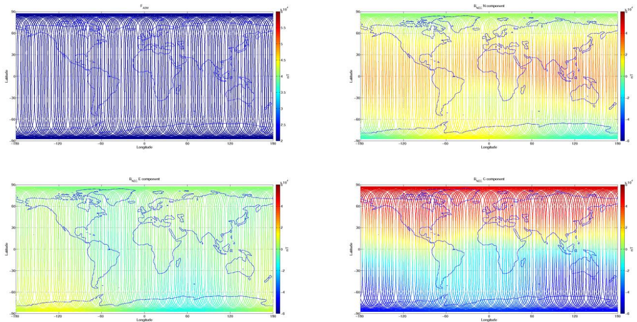
Figure 3-6: S/C A, world map plots of the geomagnetic field and components measured during monitoring period 21/09-27/09. From top to bottom: F-magnetic field from ASM measurement, B_{NEC} components (North, East, and Centre) of magnetic field from VFM measurement.
