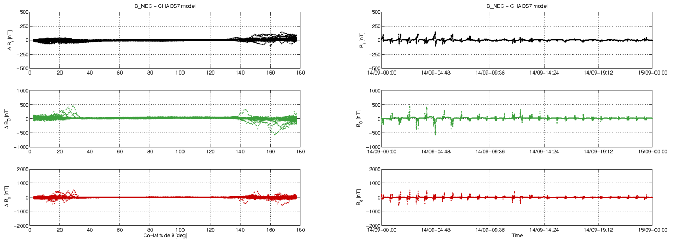
Figure 3-12: S/C C day 14.09: time series of B_{NEC} - B_{Chaos} residuals (right) and B_{NEC} - B_{Chaos} vs colatitude (left).
