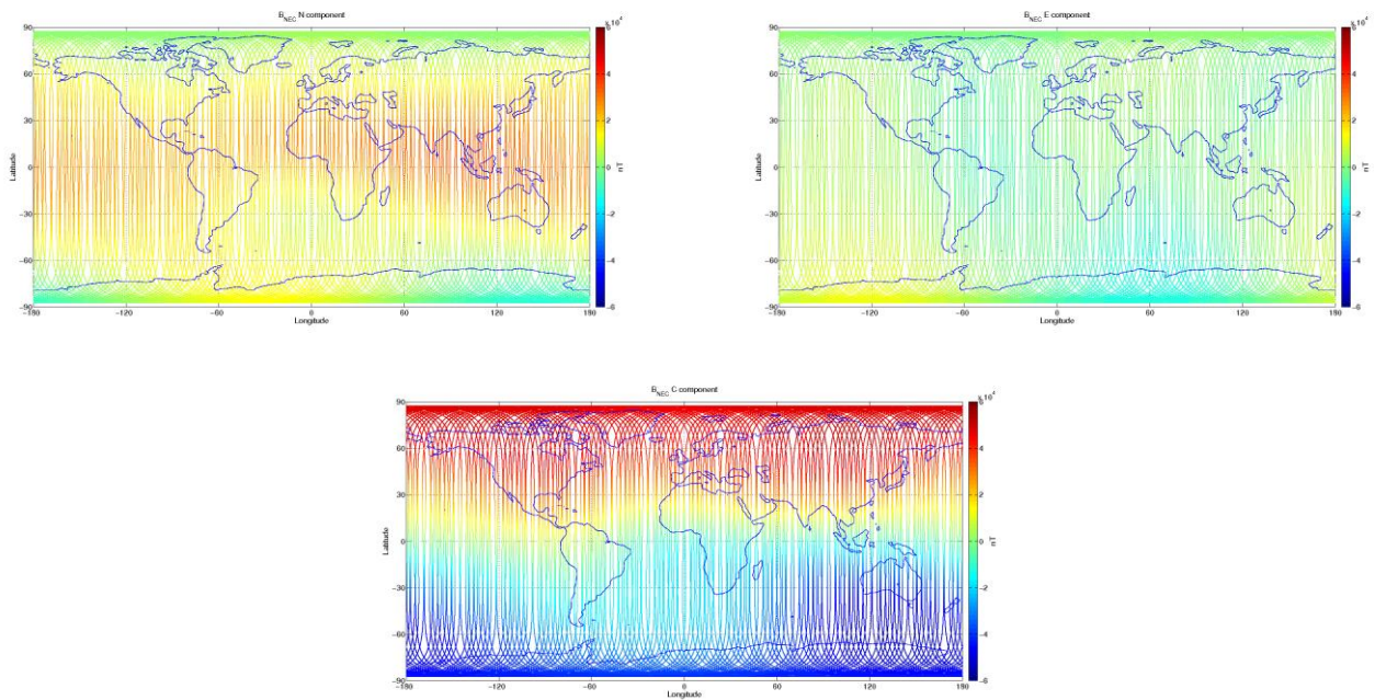
Figure 3-9: S/C C, world map plots of the geomagnetic field and components measured during monitoring period 14/09-20/09. From top to bottom: B_{NEC} components (North, East, and Centre) of magnetic field from VFM measurement.
