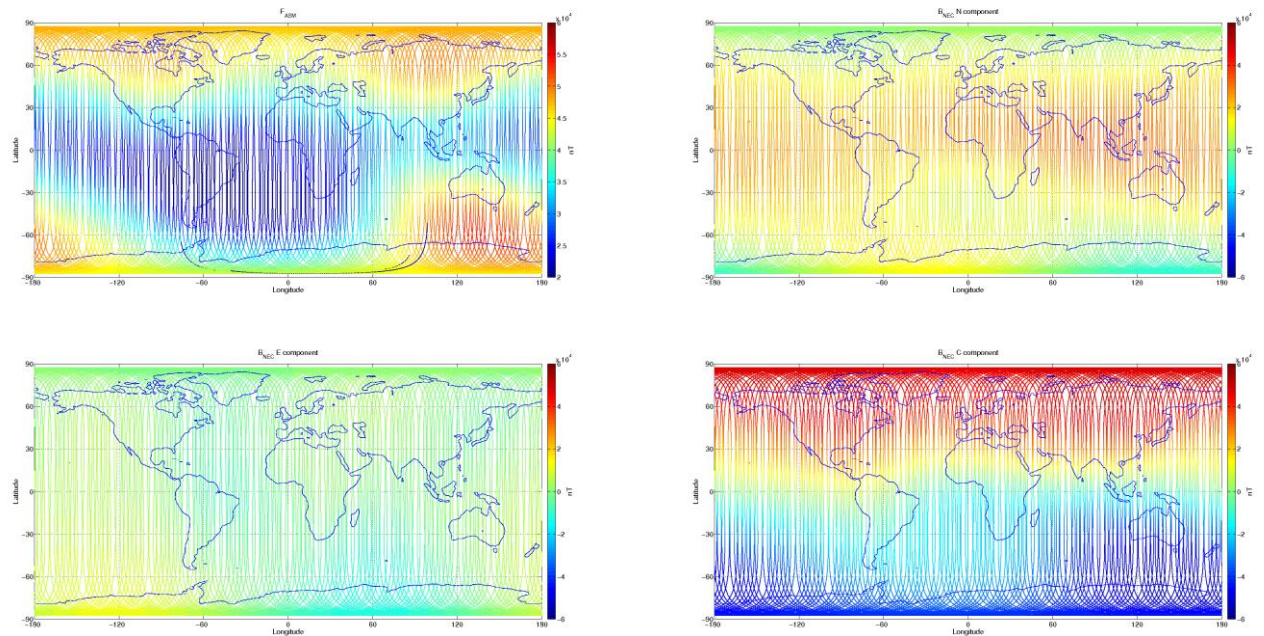
Figure 3-7: S/C A, world map plots of the geomagnetic field and components measured during monitoring period 14/09-20/09. From top to bottom: F-magnetic field from ASM measurement, B_{NEC} components (North, East, and Centre) of magnetic field from VFM measurement.
