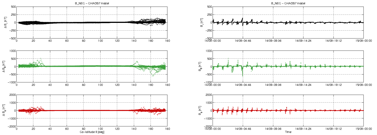
Figure 3-10: S/C A day 14.09: time series of B_{\text{NEC}} - B_{\text{ChaoS}} residuals (right) and B_{\text{NEC}} - B_{\text{ChaoS}} vs colatitude (left).
