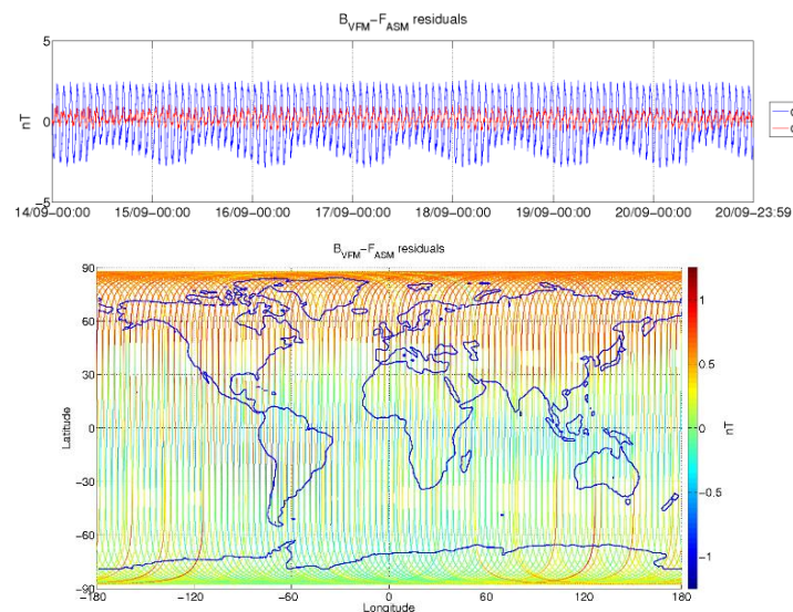
Figure 3-6: ASM-VFM residuals for S/C B, during monitoring period 14/09-20/09. In top figure are plotted: difference between |B_{VFM}| and F_{ASM} (without dB_{Sun} correction) (blue colour), and the residuals with dB_{Sun} corrections (red colour). In bottom figure residuals are presented on the world map.
