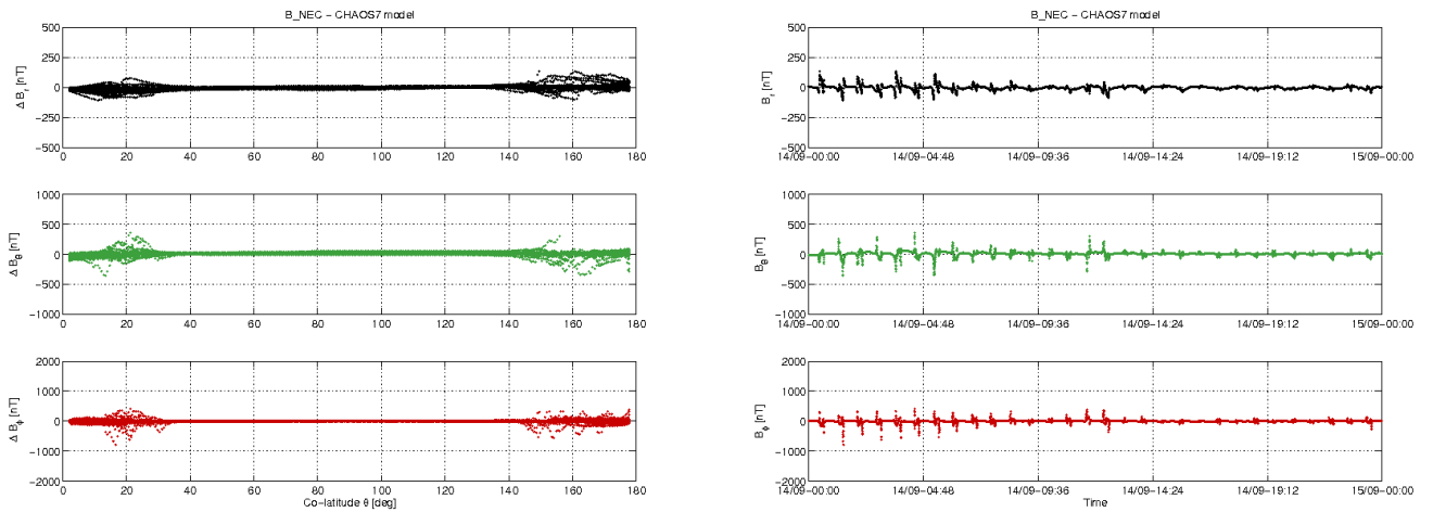
Figure 3-11: S/C B day 14.09: time series of B_{\text{NEC}} - B_{\text{ChaoS}} residuals (right) and B_{\text{NEC}} - B_{\text{ChaoS}} vs colatitude (left).
