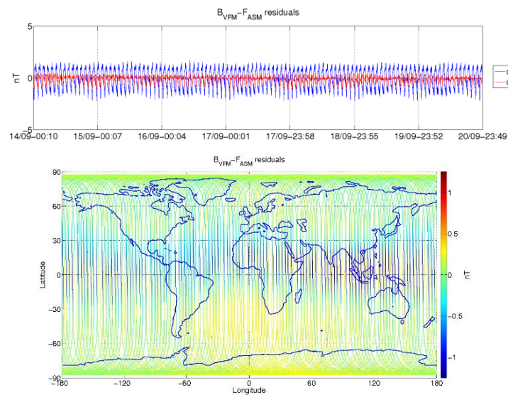
Figure 3-5: ASM-VFM residuals for S/C A, during monitoring period 14/09-20/09. In top figure are plotted: difference between |B_{VFM}| and F_{ASM} (without dB_{Sun} correction) (blue colour), and the residuals with dB_{Sun} corrections (red colour). In bottom figure residuals are presented on the world map.
