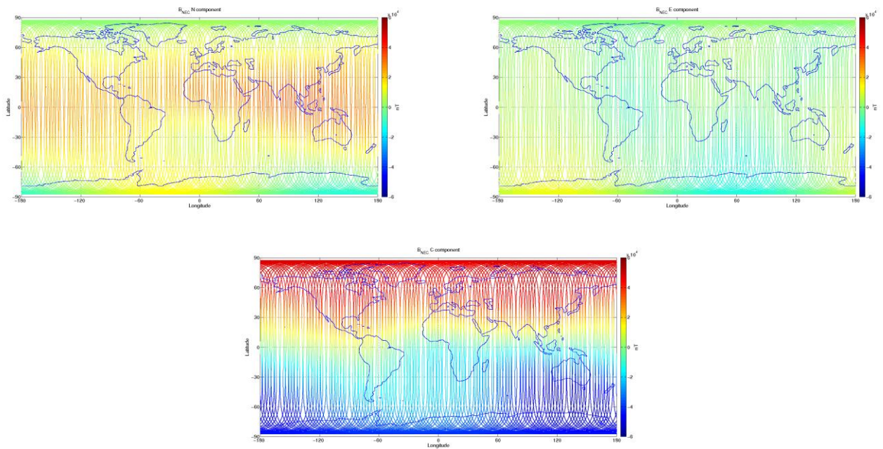
Figure 3-9: S/C C, world map plots of the geomagnetic field and components measured during monitoring period 07/09-13/09. From top to bottom: B_{NEC} components (North, East, and Centre) of magnetic field from VFM measurement.
