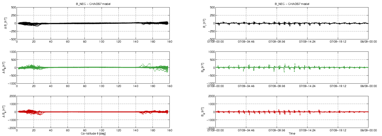
Figure 3-11: S/C B day 07.09: time series of B_{\text{NEC}} - B_{\text{ChaoS}} residuals (right) and B_{\text{NEC}} - B_{\text{ChaoS}} vs colatitude (left).
