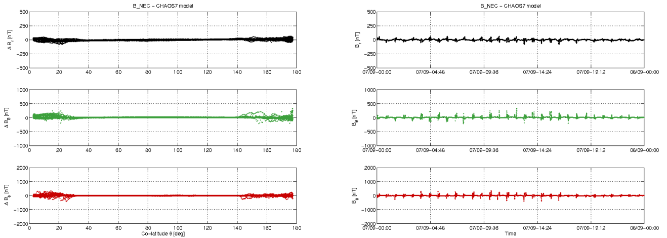
Figure 3-12: S/C C day 07.09: time series of B_{NEC} - B_{Chaos} residuals (right) and B_{NEC} - B_{Chaos} vs colatitude (left).
