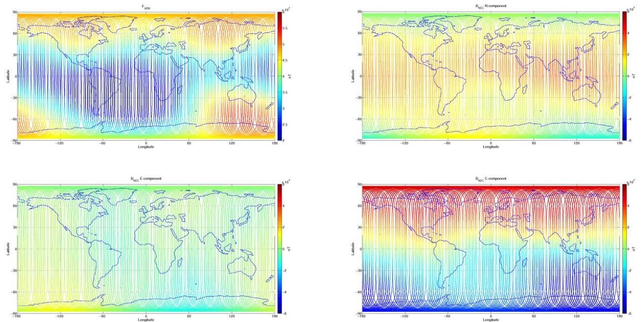
Figure 3-7: S/C A, world map plots of the geomagnetic field and components measured during monitoring period 07/09-13/09. From top to bottom: F-magnetic field from ASM measurement, B_{NEC} components (North, East, and Centre) of magnetic field from VFM measurement.
