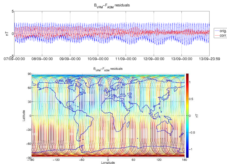
Figure 3-6: ASM-VFM residuals for S/C B, during monitoring period 07/09-13/09. In top figure are plotted: difference between |B_{VFM}| and F_{ASM} (without dB_{Sun} correction) (blue colour), and the residuals with dB_{Sun} corrections (red colour). In bottom figure residuals are presented on the world map.
