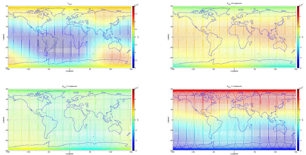
Figure 3-8: S/C B, world map plots of the geomagnetic field and components measured during monitoring period 07/09-13/09. From top to bottom: F-magnetic field from ASM measurement, B_{NEC} components (North, East, and Centre) of magnetic field from VFM measurement.
