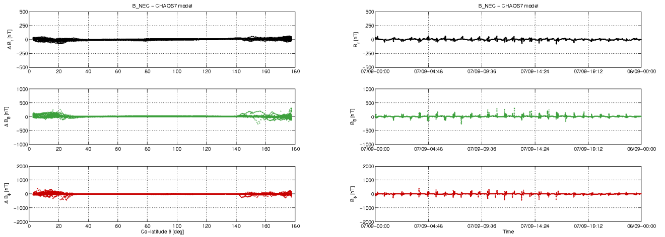
Figure 3-10: S/C A day 07.09: time series of B_{\text{NEC}} - B_{\text{ChaoS}} residuals (right) and B_{\text{NEC}} - B_{\text{ChaoS}} vs colatitude (left).
