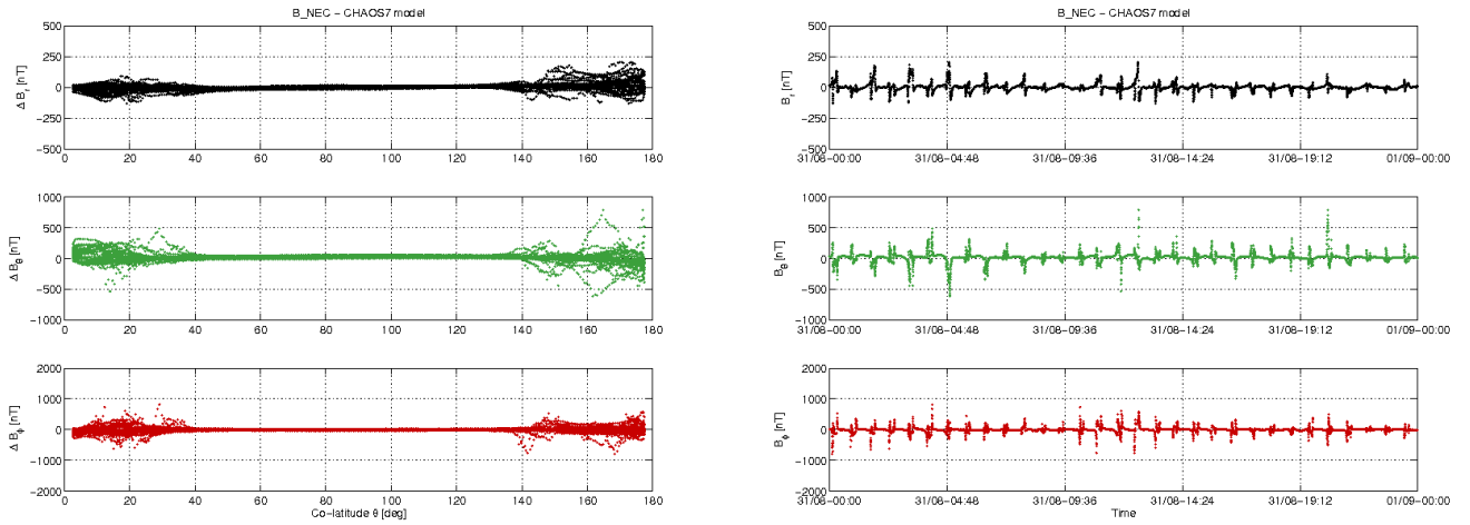
Figure 3-10: S/C A day 31.08: time series of B_{NEC} - B_{ChaoS} residuals (right) and B_{NEC} - B_{ChaoS} vs colatitude (left).
