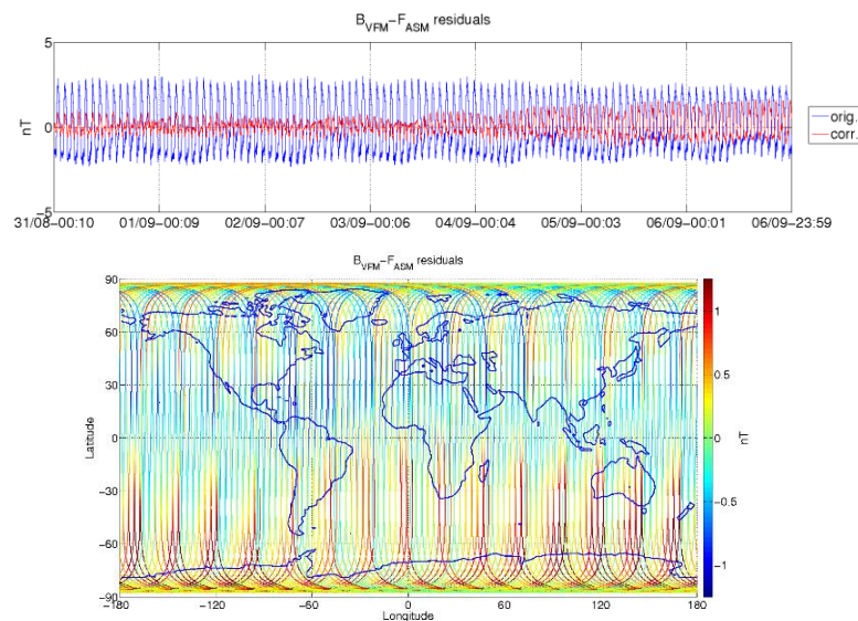
Figure 3-6: ASM-VFM residuals for S/C B, during monitoring period 31/08-06/09. In top figure are plotted: difference between |B_{VFM}| and F_{ASM} (without dB_{Sun} correction) (blue colour), and the residuals with dB_{Sun} corrections (red colour). In bottom figure residuals are presented on the world map.
