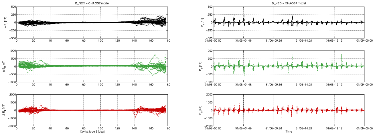
Figure 3-12: S/C C day 31.08: time series of B_{NEC} - B_{Chaos} residuals (right) and B_{NEC} - B_{Chaos} vs colatitude (left).
