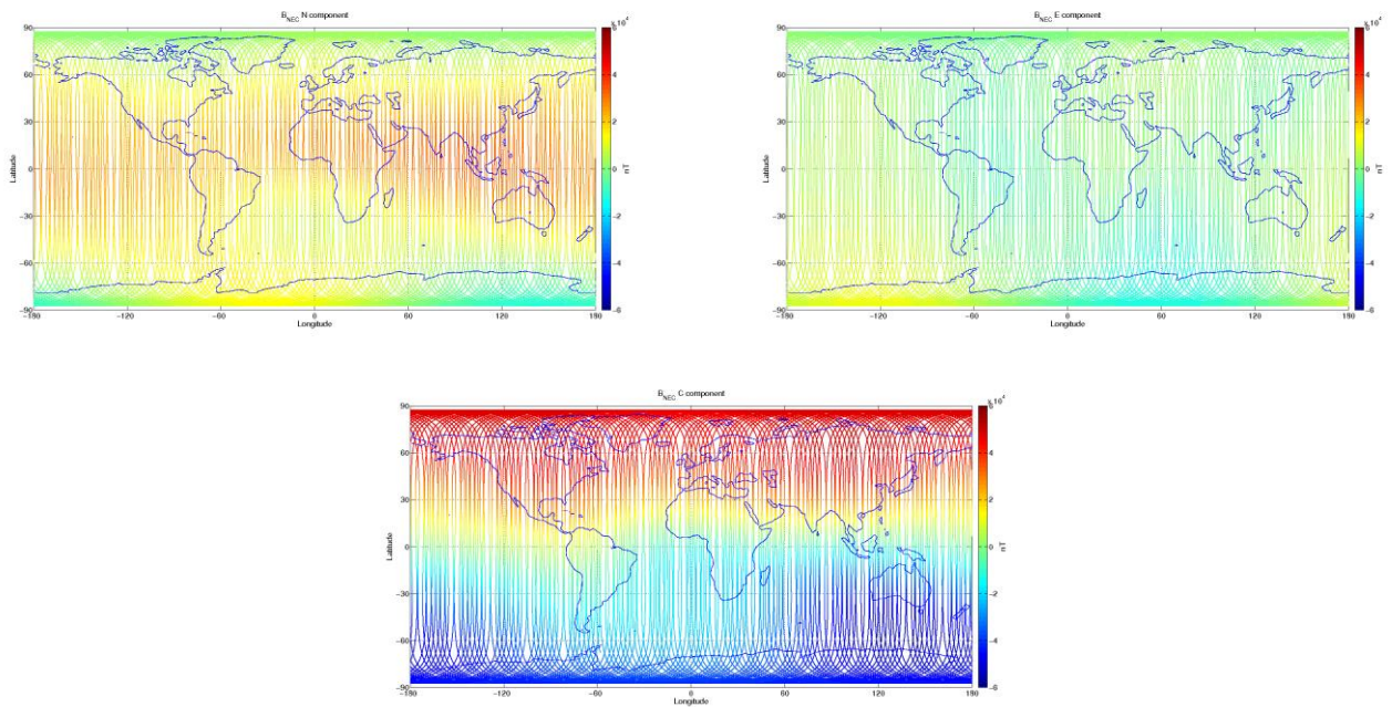
Figure 3-9: S/C C, world map plots of the geomagnetic field and components measured during monitoring period 31/08-06/09. From top to bottom: B_{NEC} components (North, East, and Centre) of magnetic field from VFM measurement.
