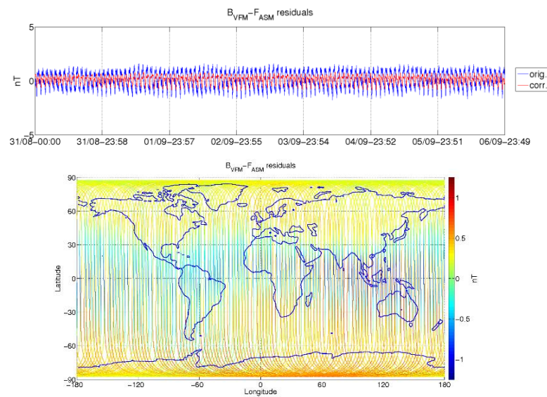
Figure 3-5: ASM-VFM residuals for S/C A, during monitoring period 31/08-06/09. In top figure are plotted: difference between |B_{VFM}| and F_{ASM} (without dB_Sun correction) (blue colour), and the residuals with dB_Sun corrections (red colour). In bottom figure residuals are presented on the world map.
