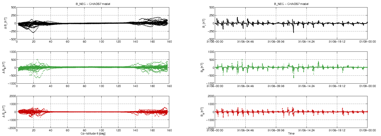
Figure 3-11: S/C B day 31.08: time series of B_{NEC} - B_{ChaoS} residuals (right) and B_{NEC} - B_{ChaoS} vs colatitude (left).
