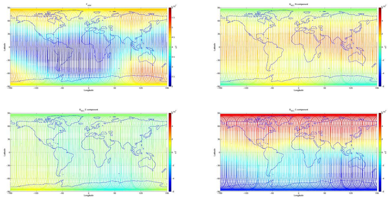
Figure 3-8: S/C B, world map plots of the geomagnetic field and components measured during monitoring period 31/08-06/09. From top to bottom: F-magnetic field from ASM measurement, B_{NEC} components (North, East, and Centre) of magnetic field from VFM measurement.
