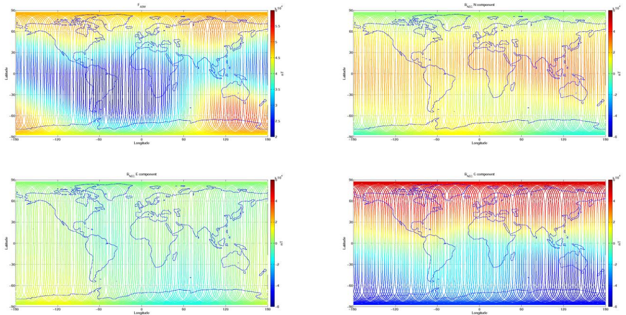
Figure 3-6: S/C A, world map plots of the geomagnetic field and components measured during monitoring period 24/08-30/08. From top to bottom: F-magnetic field from ASM measurement, B_{NEC} components (North, East, and Centre) of magnetic field from VFM measurement.
