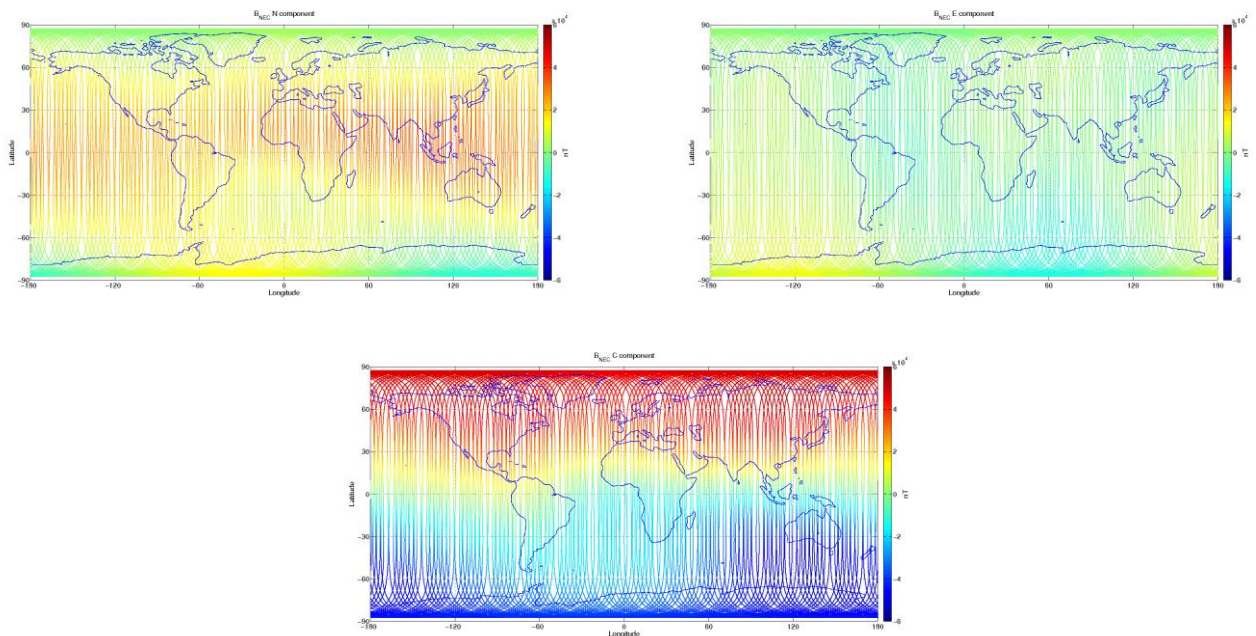
Figure 3-8: S/C C, world map plots of the geomagnetic field and components measured during monitoring period 24/08-30/08. From top to bottom: B_{NEC} components (North, East, and Centre) of magnetic field from VFM measurement.
