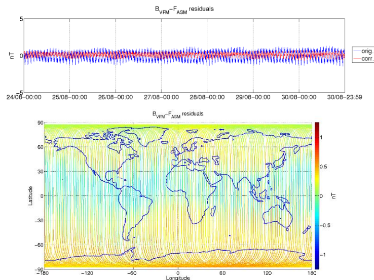
Figure 3-5: ASM-VFM residuals for S/C A, during monitoring period 24/08-30/08. In top figure are plotted: difference between |B_{VFM}| and F_{ASM} (without dB_{Sun} correction) (blue colour), and the residuals with dB_{Sun} corrections (red colour). In bottom figure residuals are presented on the world map.
