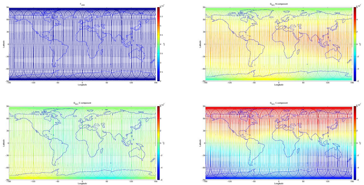
Figure 3-7: S/C B, world map plots of the geomagnetic field and components measured during monitoring period 24/08-30/08. From top to bottom: F-magnetic field from ASM measurement, B_{NEC} components (North, East, and Centre) of magnetic field from VFM measurement.
