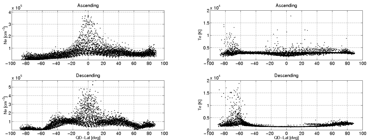
Figure 3-15: The panels shown the electron density (left) and temperature (right) profile as a function of QD Latitudes for the last week of operation. The analysis is made separately for ascending (upper panels) and descending (bottom panels) orbits.
