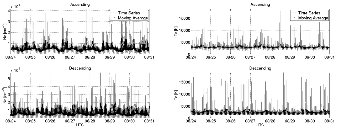
Figure 3-12: The panels show the electron density (left) and temperature (right) weekly time series (grey lines) together with the 20 min moving windows average (black lines). The analysis is made separately for ascending (upper panels) and descending (bottom panels) orbits. The average magnetic local time during the week is 8 p.m. for ascending phase and 8 a.m. for descending phase.
