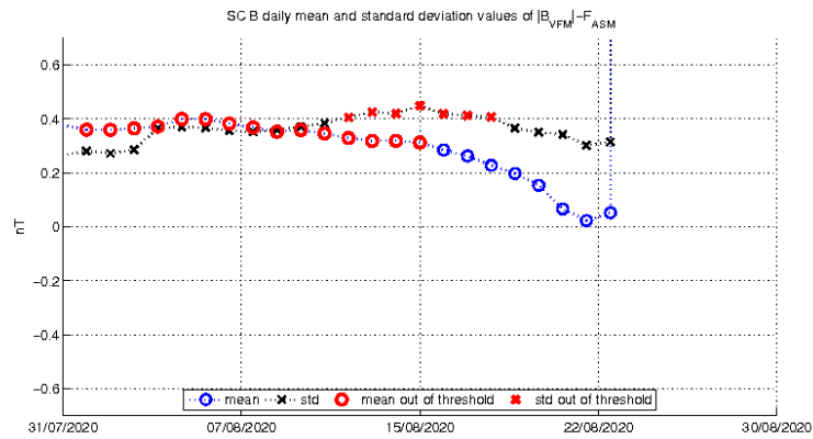
Figure 3-4: Daily mean and standard deviation values of ASM-VFM residuals (defined as dF=|B_{VFM}|-F_{ASM} ) for S/C B. The jump on the graph is due to ASM burst mode data processing failure.
