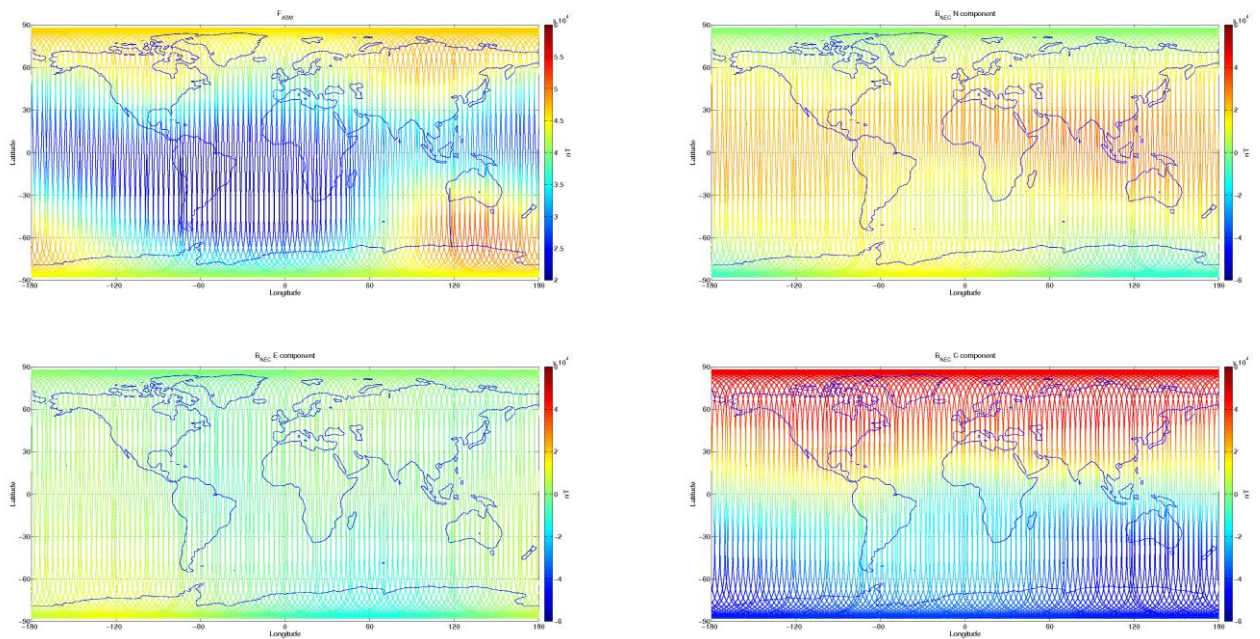
Figure 3-8: S/C B, world map plots of the geomagnetic field and components measured during monitoring period 17/08-23/08. From top to bottom: F-magnetic field from ASM measurement, B_{NEC} components (North, East, and Centre) of magnetic field from VFM measurement.
