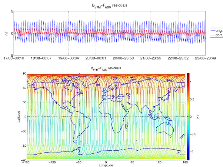
Figure 3-6: ASM-VFM residuals for S/C B, during monitoring period 17/08-23/08. In top figure are plotted: difference between |B_{VFM}| and F_{ASM} (without dB_{Sun} correction) (blue colour), and the residuals with dB_{Sun} corrections (red colour). In bottom figure residuals are presented on the world map.
