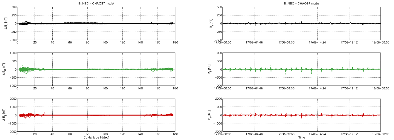
Figure 3-12: S/C C day 17.08: time series of B_{NEC} - B_{Chaos} residuals (right) and B_{NEC} - B_{Chaos} vs colatitude (left).
