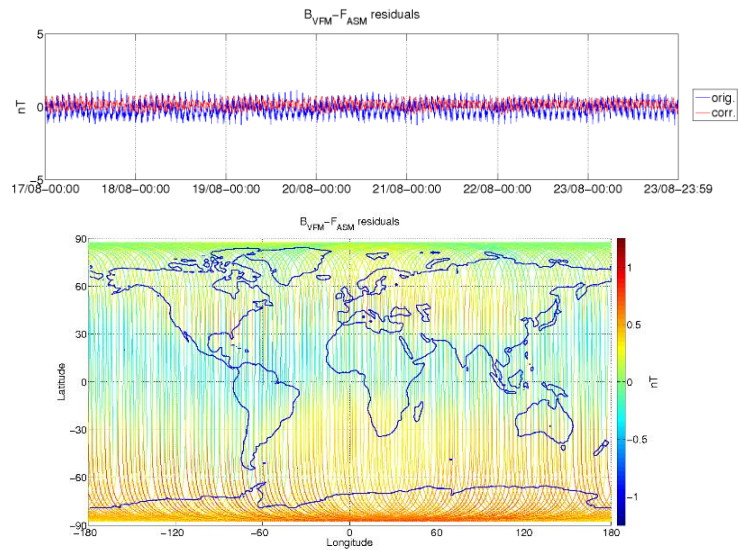
Figure 3-5: ASM-VFM residuals for S/C A, during monitoring period 17/08-23/08. In top figure are plotted: difference between |B_{VFM}| and F_{ASM} (without dB_{Sun} correction) (blue colour), and the residuals with dB_{Sun} corrections (red colour). In bottom figure residuals are presented on the world map.
