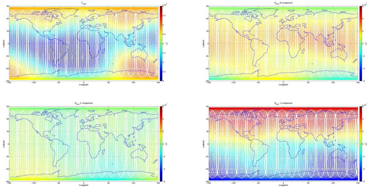
Figure 3-7: S/C A, world map plots of the geomagnetic field and components measured during monitoring period 17/08-23/08. From top to bottom: F_{msm} magnetic field from ASM measurement, B_{NEC} components (North, East, and Centre) of magnetic field from VFM measurement.
