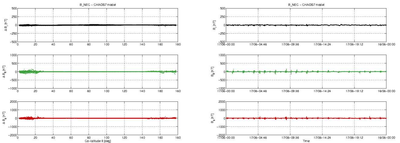
Figure 3-11: S/C B day 17.08: time series of B_{NEC} - B_{Chaos} residuals (right) and B_{NEC} - B_{Chaos} vs colatitude (left).
