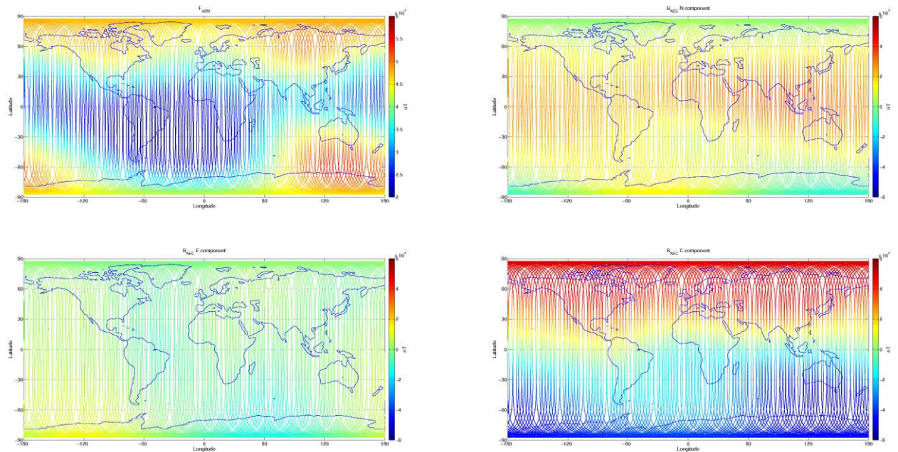
Figure 3-7: S/C A, world map plots of the geomagnetic field and components measured during monitoring period 10/08-16/08. From top to bottom: F-magnetic field from ASM measurement, B_{NEC} components (North, East, and Centre) of magnetic field from VFM measurement.
