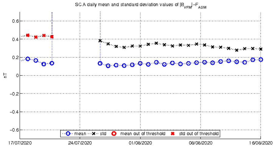
Figure 3-3: Daily mean and standard deviation values of ASM-VFM residuals (defined as dF = |B_{VFM}| - F_{ASM} ) for S/C A. Gap on the graph is caused by an error in processing of ASM BURST mode data
