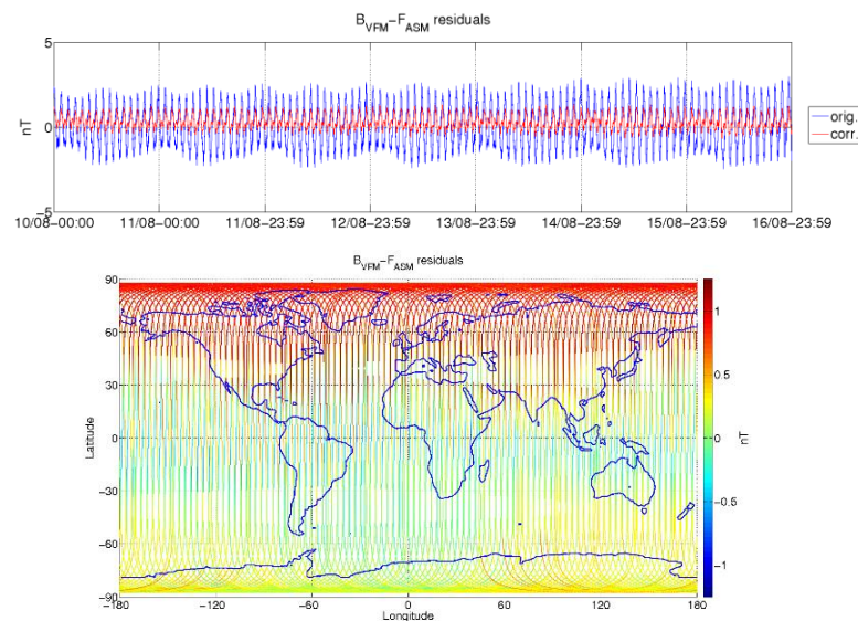
Figure 3-6: ASM-VFM residuals for S/C B, during monitoring period 10/08-16/08. In top figure are plotted: difference between |B_{VFM}| and F_{ASM} (without dB_{Sun} correction) (blue colour), and the residuals with dB_{Sun} corrections (red colour). In bottom figure residuals are presented on the world map.
