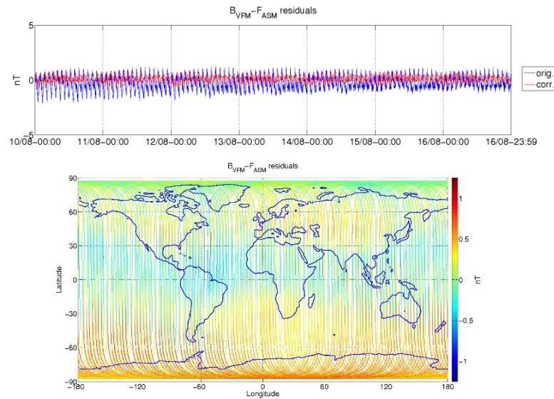
Figure 3-5: ASM-VFM residuals for S/C A, during monitoring period 10/08-16/08. In top figure are plotted: difference between |B_{VFM}| and F_{ASM} (without dB_{Sun} correction) (blue colour), and the residuals with dB_{Sun} corrections (red colour). In bottom figure residuals are presented on the world map.
