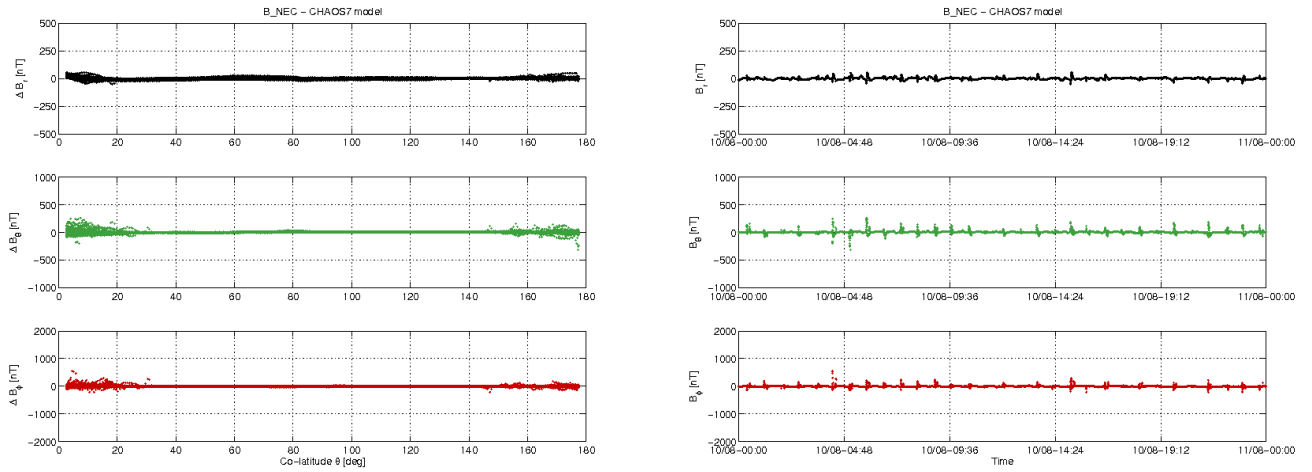
Figure 3-10: S/C A day 10.08: time series of B_{NEC} - B_{Chaos} residuals (right) and B_{NEC} - B_{Chaos} vs colatitude (left).
