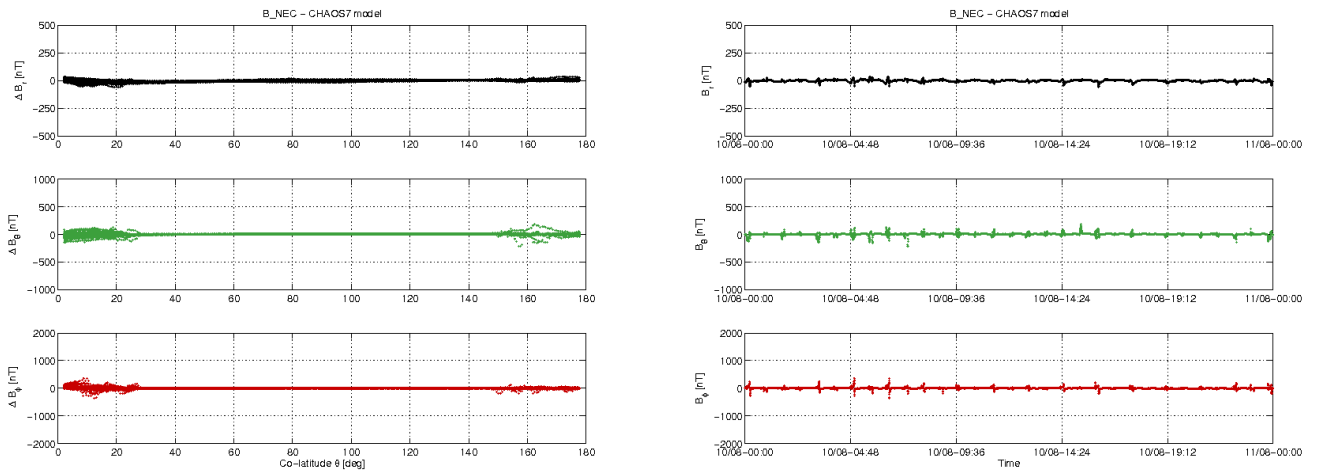
Figure 3-11: S/C B day 10.08: time series of B_{NEC} - B_{Chaos} residuals (right) and B_{NEC} - B_{Chaos} vs colatitude (left).
