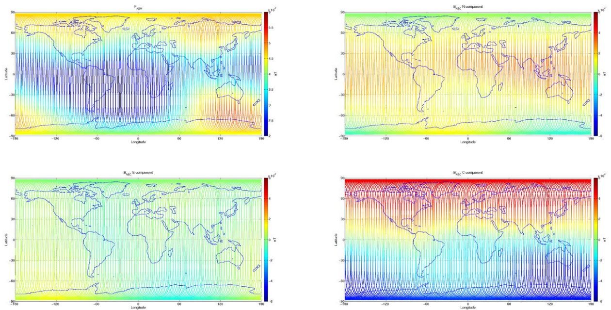
Figure 3-8: S/C B, world map plots of the geomagnetic field and components measured during monitoring period 10/08-16/08. From top to bottom: F-magnetic field from ASM measurement, B_{NEC} components (North, East, and Centre) of magnetic field from VFM measurement.
