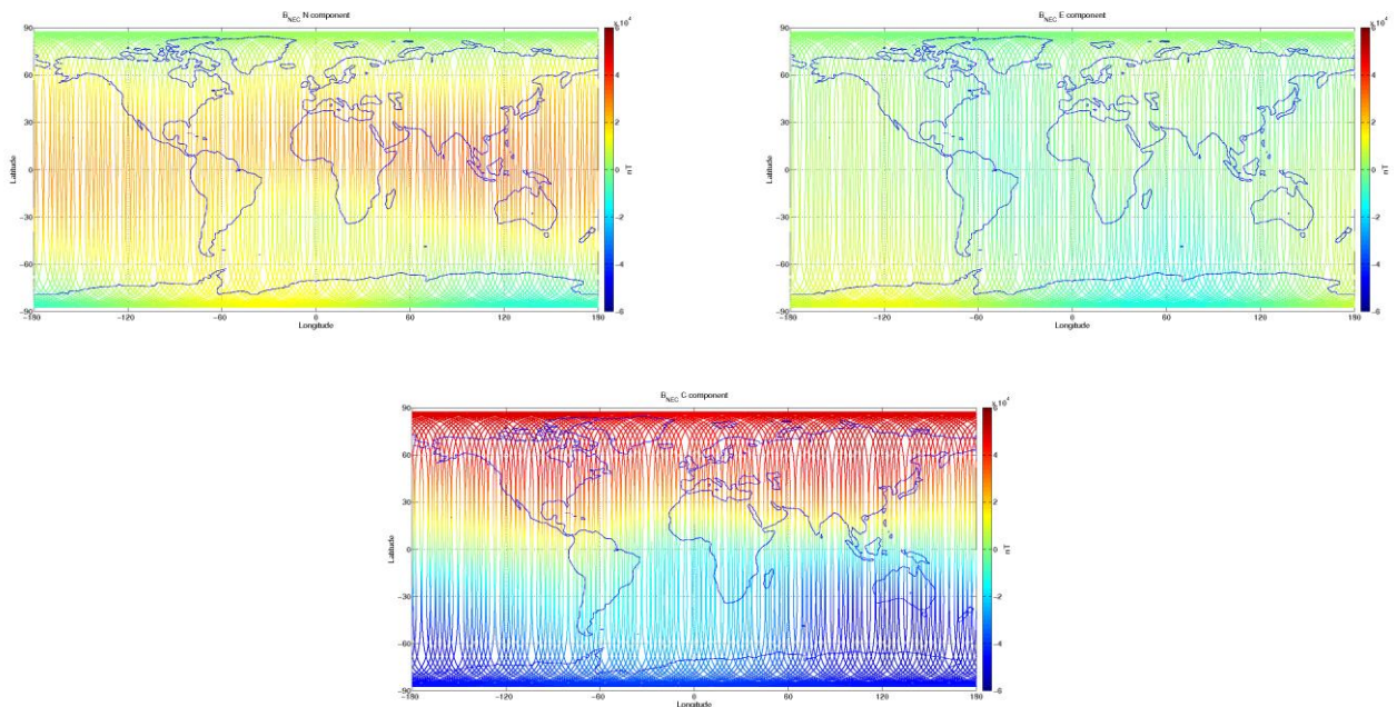
Figure 3-9: S/C C, world map plots of the geomagnetic field and components measured during monitoring period 10/08-16/08. From top to bottom: B_{NEC} components (North, East, and Centre) of magnetic field from VFM measurement.
