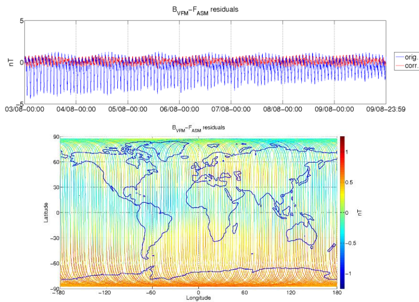
Figure 3-5: ASM-VFM residuals for S/C A, during monitoring period 03/08-09/08. In top figure are plotted: difference between |B_{VFM}| and F_{ASM} (without dB_{Sun} correction) (blue colour), and the residuals with dB_{Sun} corrections (red colour). In bottom figure residuals are presented on the world map.
