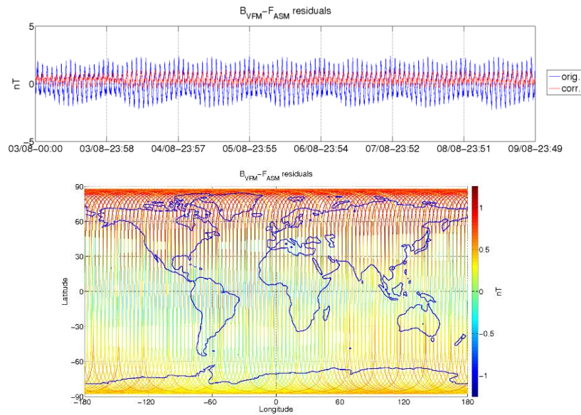
Figure 3-6: ASM-VFM residuals for S/C B, during monitoring period 03/08-09/08. In top figure are plotted: difference between |B_{VFM}| and F_{ASM} (without dB_{Sun} correction) (blue colour), and the residuals with dB_{Sun} corrections (red colour). In bottom figure residuals are presented on the world map.
