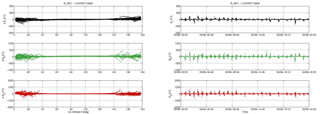
Figure 3-11: S/C B day 03.08: time series of B_{NEC} - B_{Chaos} residuals (right) and B_{NEC} - B_{Chaos} vs colatitude (left).
