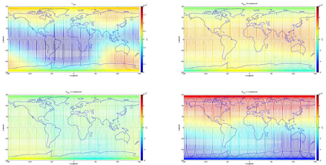
Figure 3-8: S/C B, world map plots of the geomagnetic field and components measured during monitoring period 03/08-09/08. From top to bottom: F-magnetic field from ASM measurement, B_{NEC} components (North, East, and Centre) of magnetic field from VFM measurement.
