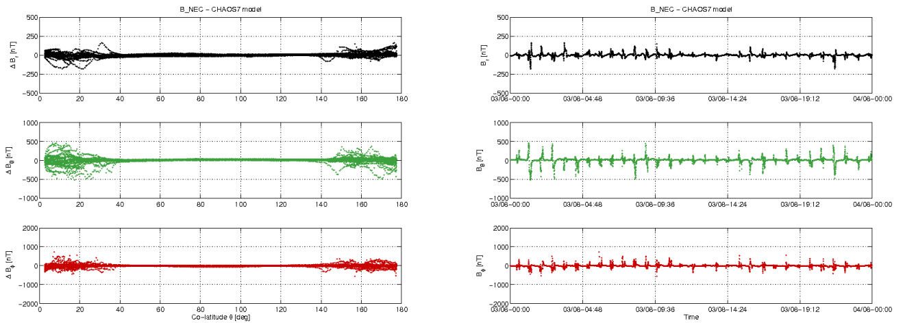
Figure 3-12: S/C C day 03.08: time series of B_{NEC} - B_{Chaos} residuals (right) and B_{NEC} - B_{Chaos} vs colatitude (left).
