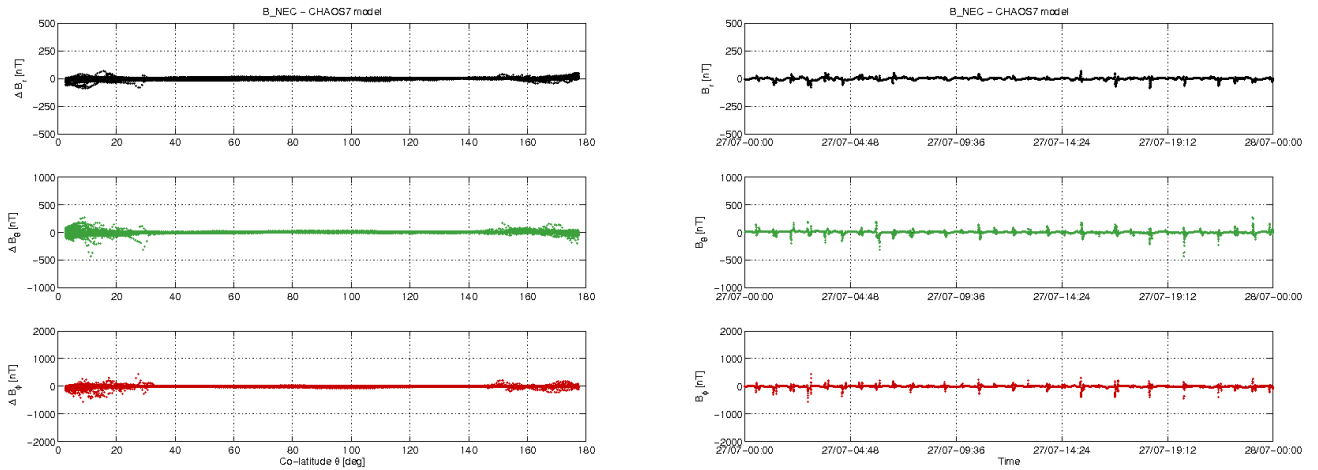
Figure 3-12: S/C C day 27.07: time series of B_{NEC} - B_{Chaos} residuals (right) and B_{NEC} - B_{Chaos} vs colatitude (left).
