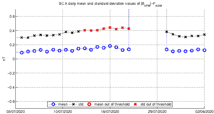
Figure 3-3: Daily mean and standard deviation values of ASM-VFM residuals (defined as dF = |B_{VFM}| - F_{ASM} ) for S/C A. The jump in the graph is caused by ASM BURST data processing.
