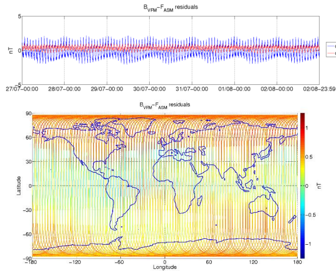
Figure 3-6: ASM-VFM residuals for S/C B, during monitoring period 27/07-02/08. In top figure are plotted: difference between |B_{VFM}| and F_{ASM} (without dB_{Sun} correction) (blue colour), and the residuals with dB_{Sun} corrections (red colour). In bottom figure residuals are presented on the world map.
