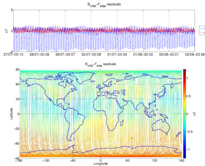
Figure 3-5: ASM-VFM residuals for S/C A, during monitoring period 27/07-02/08. In top figure are plotted: difference between |B_{VFM}| and F_{ASM} (without dB_{Sun} correction) (blue colour), and the residuals with dB_{Sun} corrections (red colour). In bottom figure residuals are presented on the world map.
