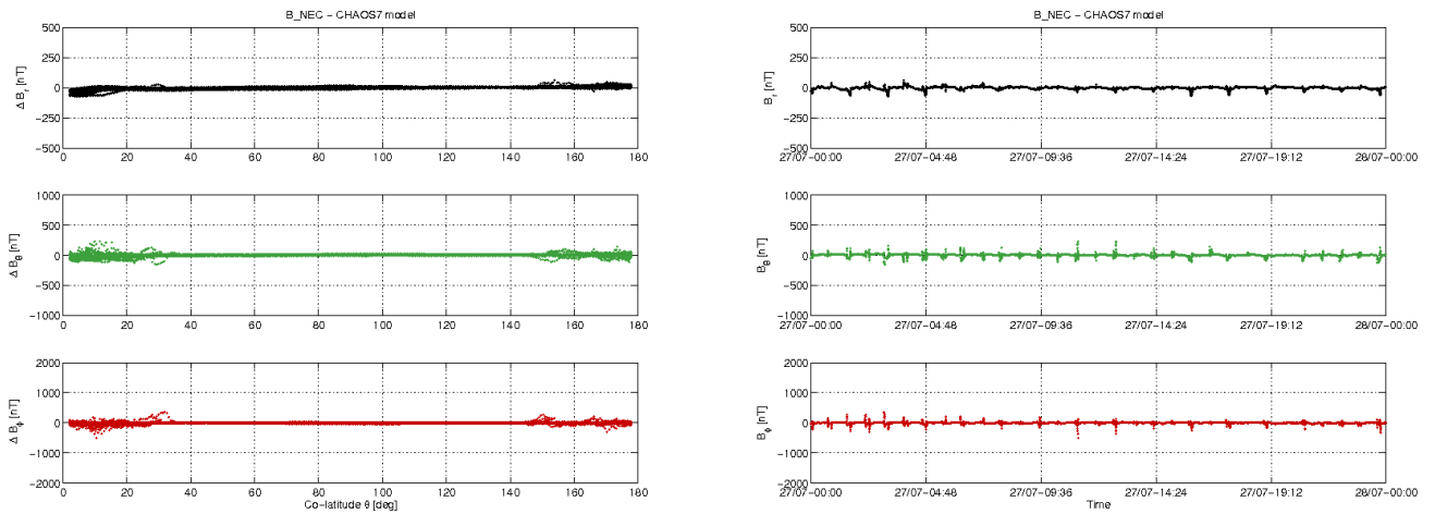
Figure 3-11: S/C B day 27.07: time series of B_{NEC} - B_{Chaos} residuals (right) and B_{NEC} - B_{Chaos} vs colatitude (left).
