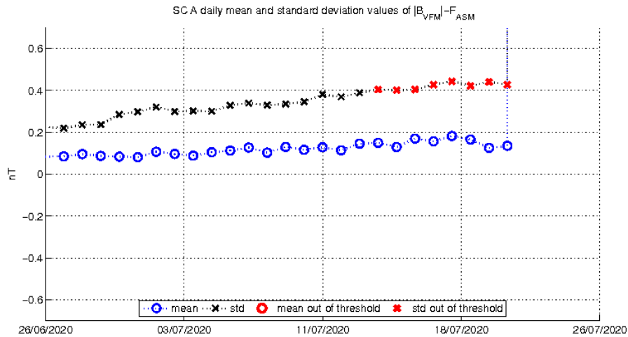
Figure 3-3: Daily mean and standard deviation values of ASM-VFM residuals (defined as dF = |B_{VFM}| - F_{ASM} ) for S/C A. Due to data gap in Burst mode further calculations failed.
