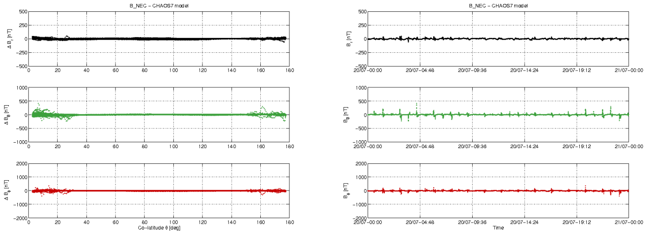
Figure 3-12: S/C C day 20.07: time series of B_{NEC} - B_{Chaos} residuals (right) and B_{NEC} - B_{Chaos} vs colatitude (left).
