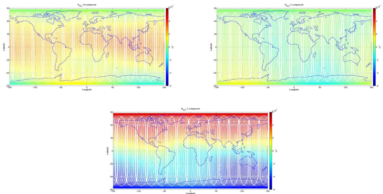
Figure 3-9: S/C C, world map plots of the geomagnetic field and components measured during monitoring period 20/07-26/07. From top to bottom: B_{NEC} components (North, East, and Centre) of magnetic field from VFM measurement.
