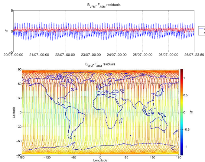
Figure 3-6: ASM-VFM residuals for S/C B, during monitoring period 20/07-26/07. In top figure are plotted: difference between |B_{VFM}| and F_{ASM} (without dB_{Sun} correction) (blue colour), and the residuals with dB_{Sun} corrections (red colour). In bottom figure residuals are presented on the world map.
