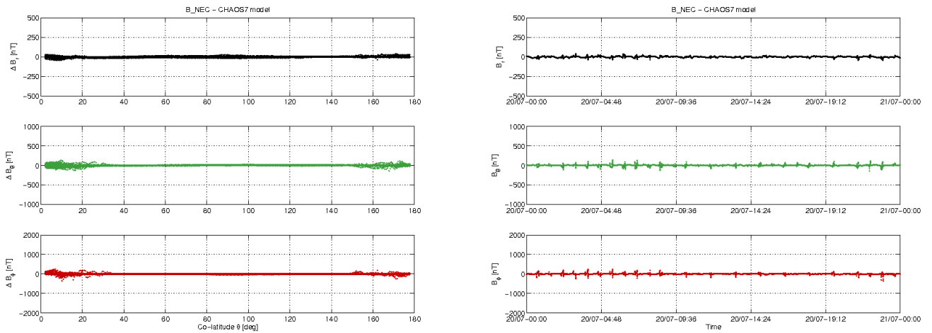
Figure 3-11: S/C B day 20.07: time series of B_{NEC} - B_{Chaos} residuals (right) and B_{NEC} - B_{Chaos} vs colatitude (left).
