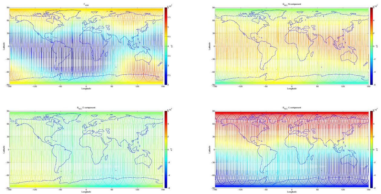
Figure 3-8: S/C B, world map plots of the geomagnetic field and components measured during monitoring period 20/07-26/07. From top to bottom: F-magnetic field from ASM measurement, B_{NEC} components (North, East, and Centre) of magnetic field from VFM measurement.
