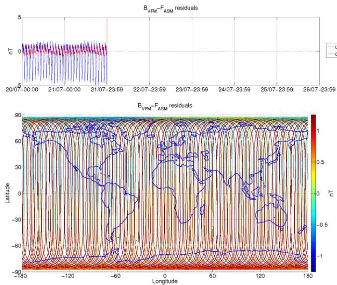
Figure 3-5: ASM-VFM residuals for S/C A, during monitoring period 20/07-26/07. In top figure are plotted: difference between |B_{VFM}| and F_{ASM} (without dB_{Sun} correction) (blue colour), and the residuals with dB_{Sun} corrections (red colour). In bottom figure residuals are presented on the world map.
