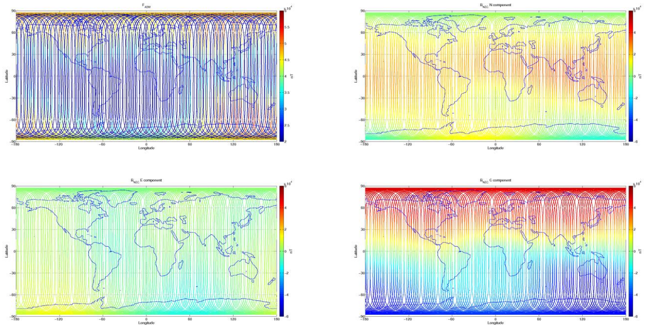
Figure 3-7: S/C A, world map plots of the geomagnetic field and components measured during monitoring period 20/07-26/07. From top to bottom: F-magnetic field from ASM measurement, B_{NEC} components (North, East, and Centre) of magnetic field from VFM measurement.
