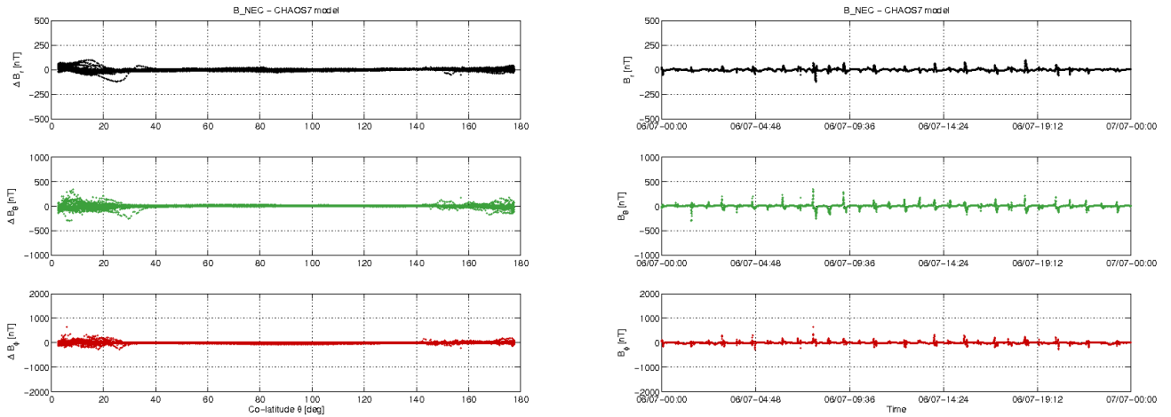
Figure 3-12: S/C C day 06/07: time series of B_{NEC} - B_{Chaos} residuals (right) and B_{NEC} - B_{Chaos} vs colatitude (left).
