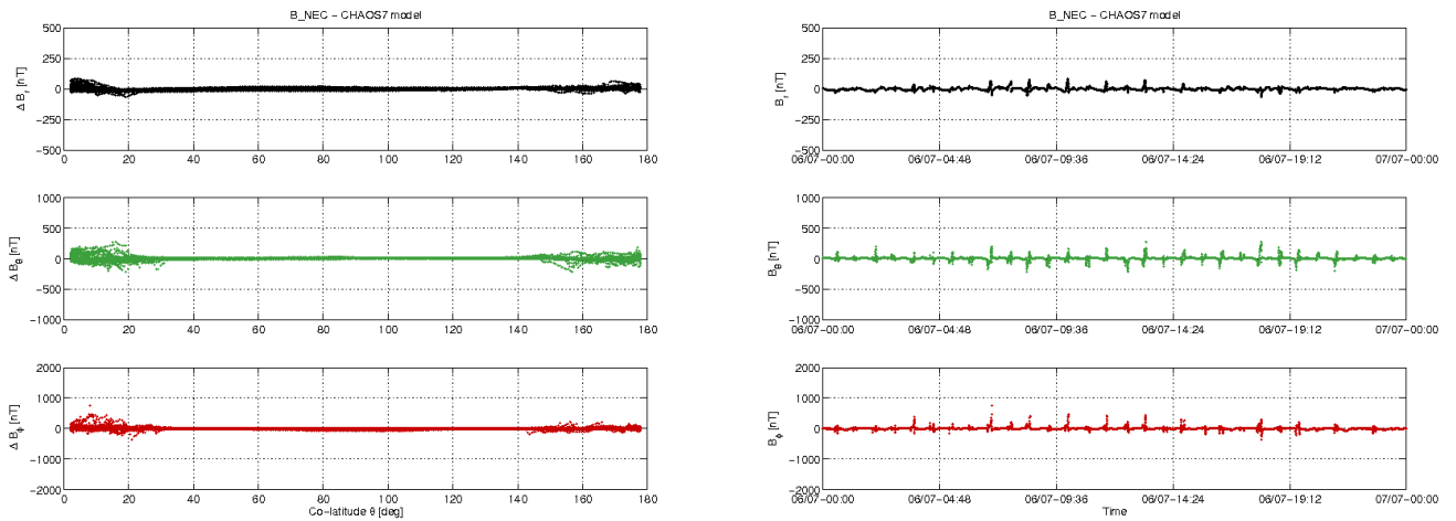
Figure 3-11: S/C B day 06.07: time series of B_{NEC} - B_{Chaos} residuals (right) and B_{NEC} - B_{Chaos} vs colatitude (left).
