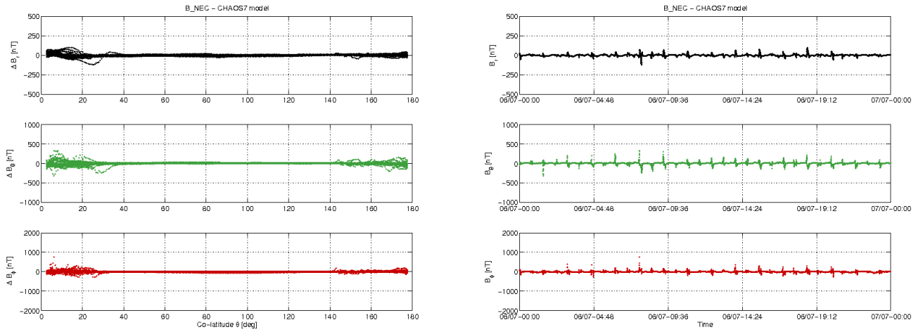
Figure 3-10: S/C A day 06.07: time series of B_{NEC} - B_{Chaos} residuals (right) and B_{NEC} - B_{Chaos} vs colatitude (left).
