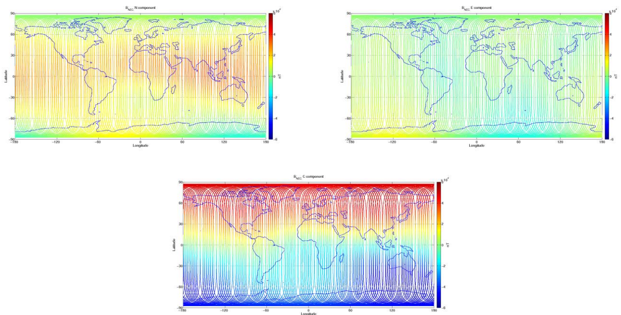
Figure 3-9: S/C C, world map plots of the geomagnetic field and components measured during monitoring period 06/07-12/07. From top to bottom: B_{NEC} components (North, East, and Centre) of magnetic field from VFM measurement.
