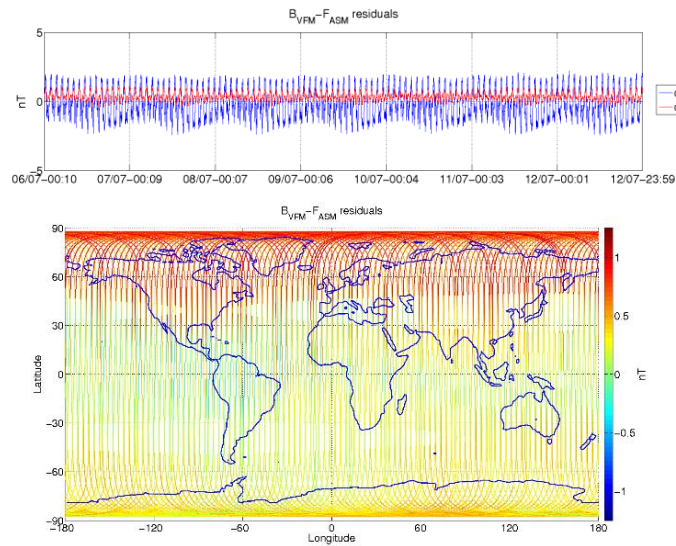
Figure 3-6: ASM-VFM residuals for S/C B, during monitoring period 06/07-12/07. In top figure are plotted: difference between |B_{VFM}| and F_{ASM} (without dB_{Sun} correction) (blue colour), and the residuals with dB_{Sun} corrections (red colour). In bottom figure residuals are presented on the world map.
