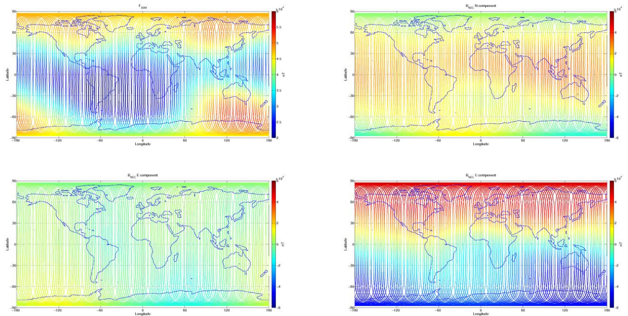
Figure 3-7: S/C A, world map plots of the geomagnetic field and components measured during monitoring period 06/07-12/07. From top to bottom: F-magnetic field from ASM measurement, B_{NEC} components (North, East, and Centre) of magnetic field from VFM measurement.
