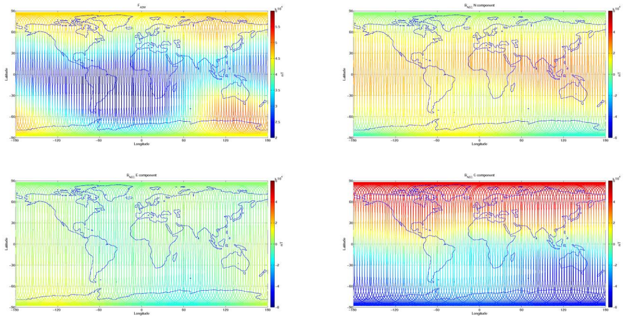
Figure 3-8: S/C B, world map plots of the geomagnetic field and components measured during monitoring period 06/07-12/07. From top to bottom: F-magnetic field from ASM measurement, B_{NEC} components (North, East, and Centre) of magnetic field from VFM measurement.
