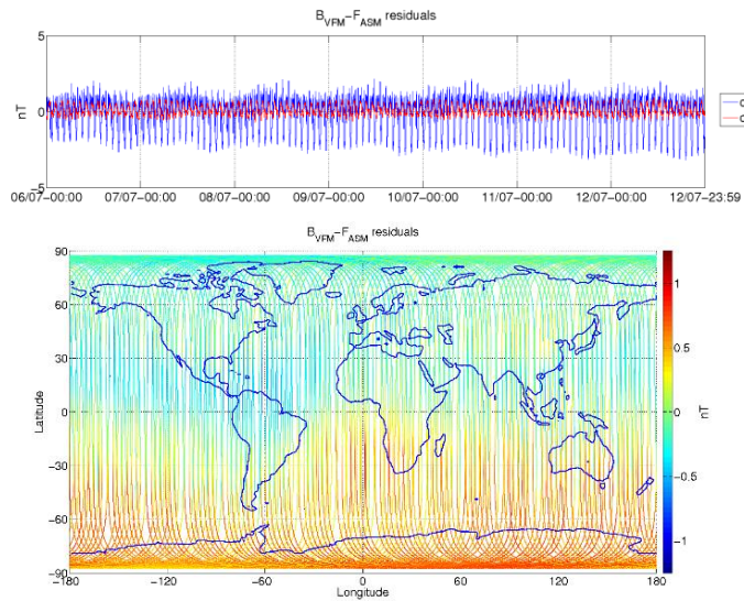
Figure 3-5: ASM-VFM residuals for S/C A, during monitoring period 06/07-12/07. In top figure are plotted: difference between |B_{VFM}| and F_{ASM} (without dB_{Sun} correction) (blue colour), and the residuals with dB_{Sun} corrections (red colour). In bottom figure residuals are presented on the world map.
