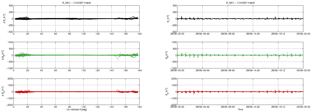
Figure 0-10: S/C A day 29.06: time series of B_{NEC} - B_{Chaos} residuals (right) and B_{NEC} - B_{Chaos} vs colatitude (left).
