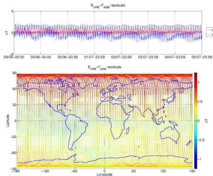
Figure 0-6: ASM-VFM residuals for S/C B, during monitoring period 29/06-05/07. In top figure are plotted: difference between |B_{VFM}| and F_{ASM} (without dB_{Sun} correction) (blue colour), and the residuals with dB_{Sun} corrections (red colour). In bottom figure residuals are presented on the world map.
