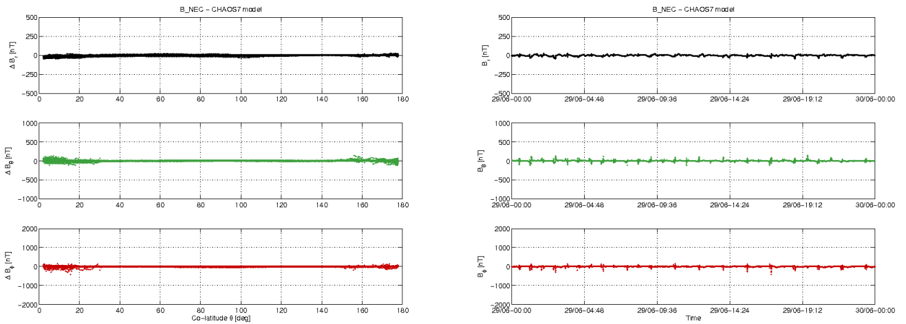
Figure 0-11: S/C B day 29.06: time series of B_{NEC} - B_{Chaos} residuals(right) and B_{NEC} - B_{Chaos} vs colatitude (left).
