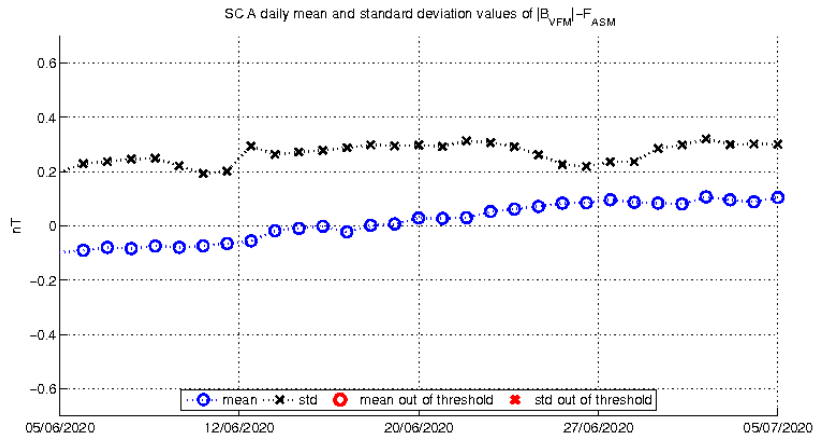
Figure 0-3: Daily mean and standard deviation values of ASM-VFM residuals (defined as dF = |B_{VFM}| - F_{ASM} ) for S/C A.
