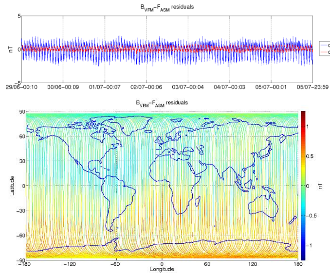
Figure 0-5: ASM-VFM residuals for S/C A, during monitoring period 29/06-05/07. In top figure are plotted: difference between |B_{VFM}| and F_{ASM} (without dB_Sun correction) (blue colour), and the residuals with dB_Sun corrections (red colour). In bottom figure residuals are presented on the world map.
