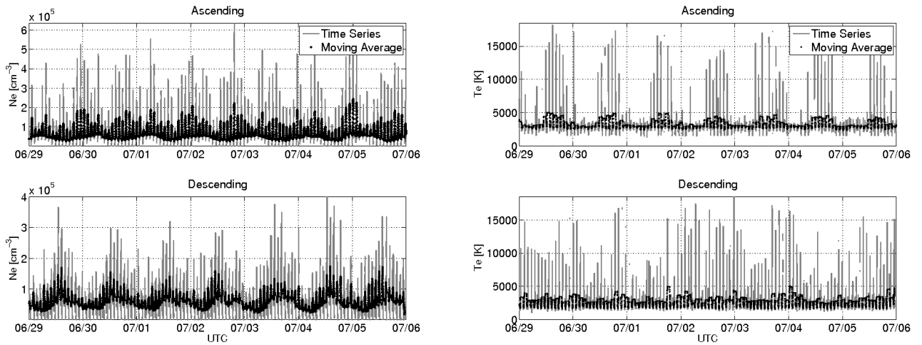
Figure 0-15: The panels show the electron density (left) and temperature (right) weekly time series (grey lines) together with the 20 min moving windows average (black lines). The analysis is made separately for ascending (upper panels) and descending (bottom panels) orbits. The average magnetic local time during the week is 2 p.m. for ascending phase and 2 a.m. for descending phase.
