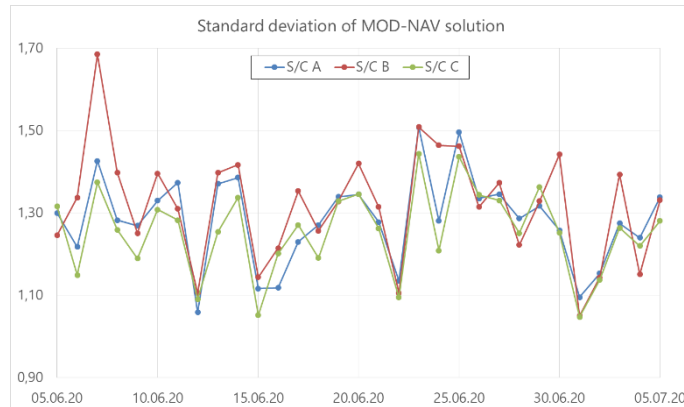
Figure 0-1: Plot of the standard deviation of the difference between MOD and NAV solutions for all satellites. Plot covers last month of operation.
