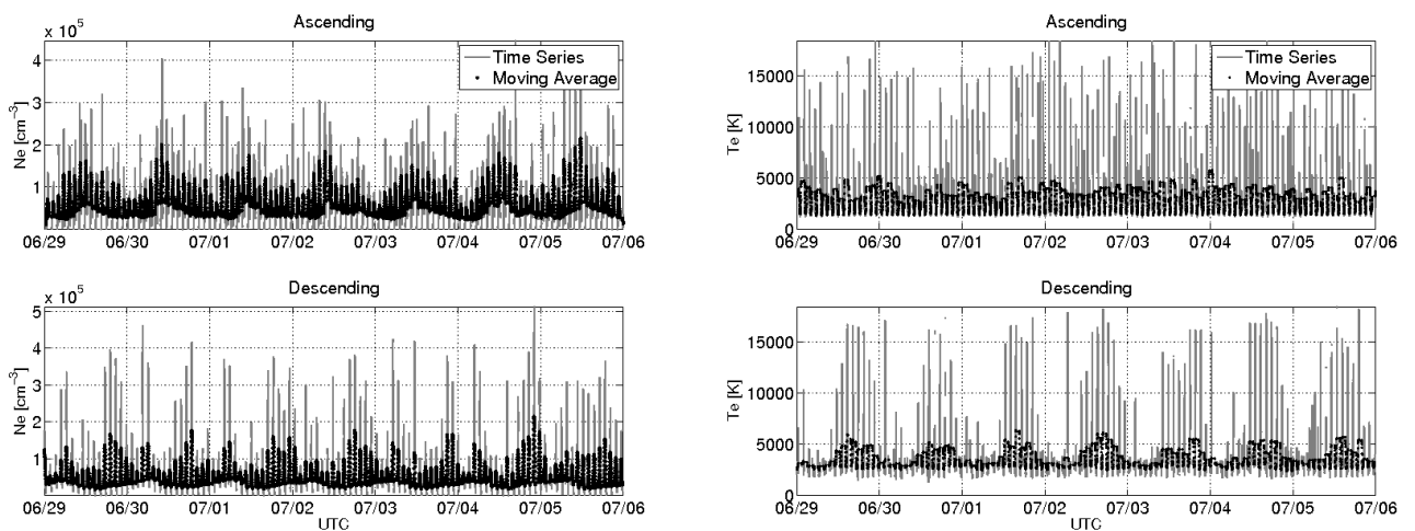
Figure 0-14: The panels show the electron density (left) and temperature (right) weekly time series (grey lines) together with the 20 min moving windows average (black lines). The analysis is made separately for ascending (upper panels) and descending (bottom panels) orbits. The average magnetic local time during the week is 11 p.m. for descending phase and 11 a.m. for ascending phase.
