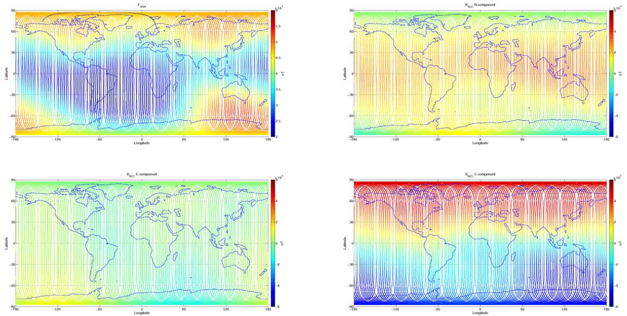
Figure 0-7: S/C A, world map plots of the geomagnetic field and components measured during monitoring period 29/06-05/07. From top to bottom: F-magnetic field from ASM measurement, B_{NEC} components (North, East, and Centre) of magnetic field from VFM measurement.
