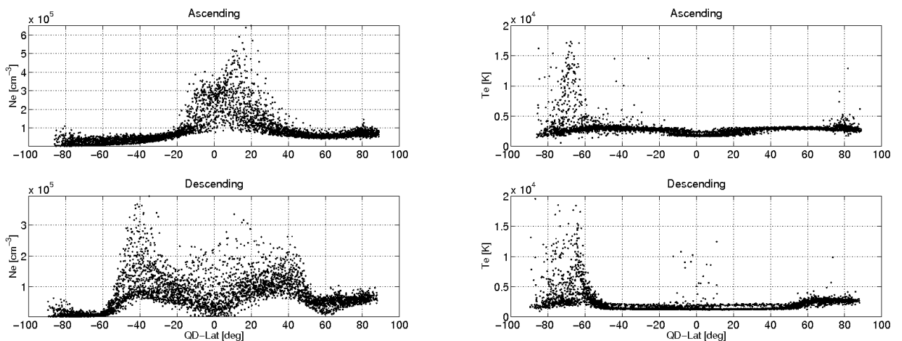
Figure 0-16: The panels shown the electron density (left) and temperature (right) profile as a function of QD Latitudes for the last week of operation. The analysis is made separately for ascending (upper panels) and descending (bottom panels) orbits.
