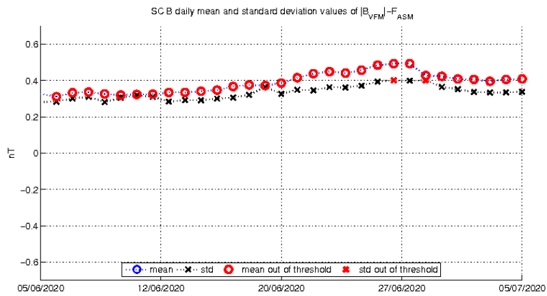
Figure 0-4: Daily mean and standard deviation values of ASM-VFM residuals (defined as dF = |B_{VFM}| - F_{ASM} ) for S/C B.
