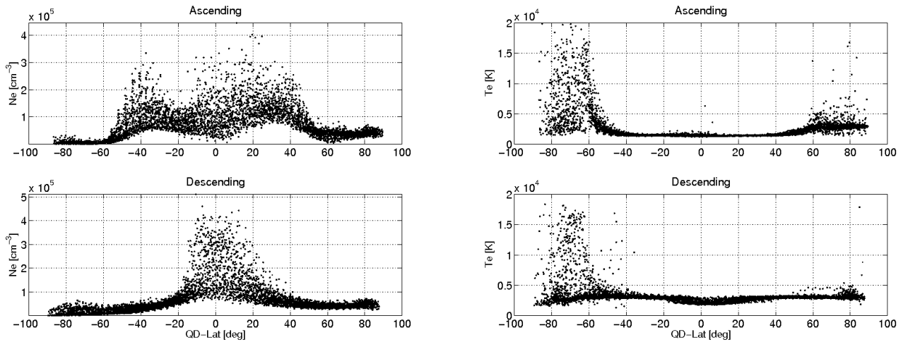
Figure 0-17: The panels shown the electron density (left) and temperature (right) profile as a function of QD Latitudes for the last week of operation. The analysis is made separately for ascending (upper panels) and descending (bottom panels) orbits.
