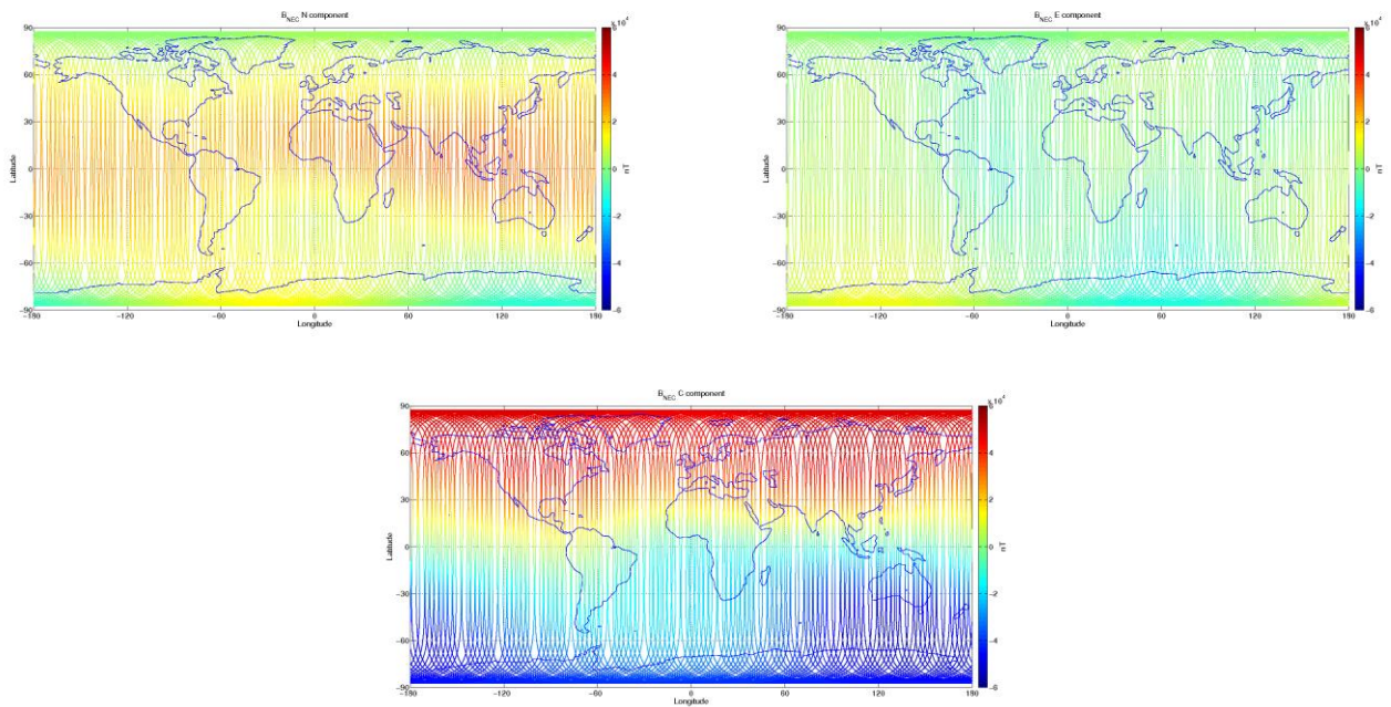
Figure 0-9: S/C C, world map plots of the geomagnetic field and components measured during monitoring period 29/06-05/07. From top to bottom: B_{NEC} components (North, East, and Centre) of magnetic field from VFM measurement.
