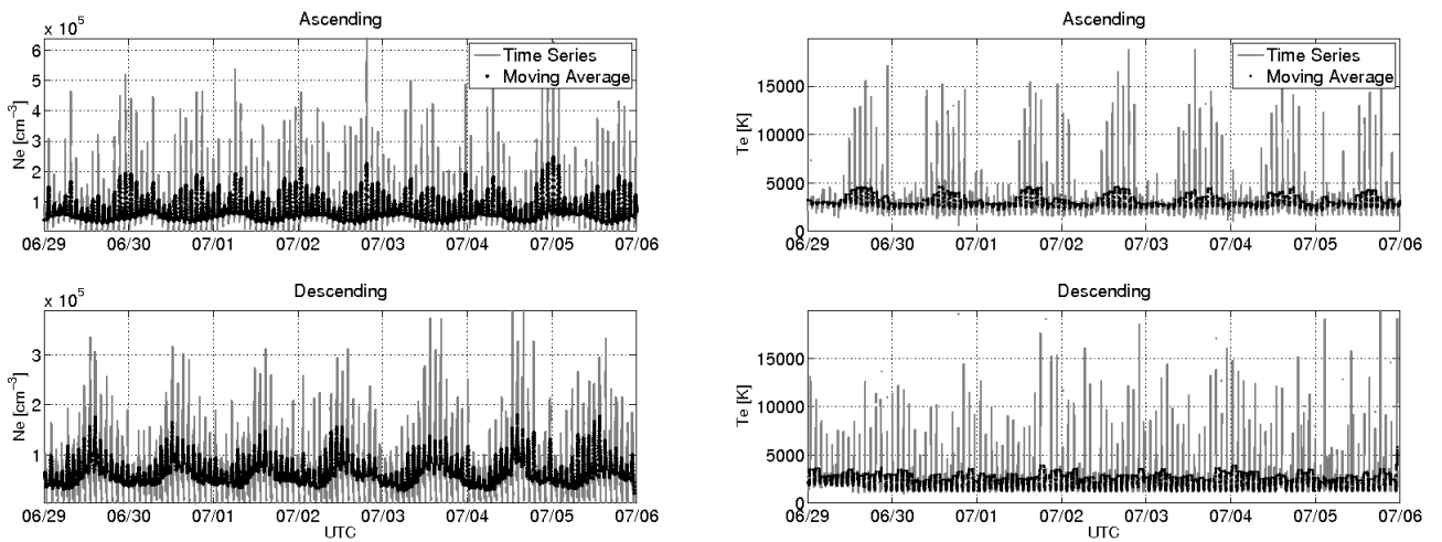
Figure 0-13: The panels show the electron density (left) and temperature (right) weekly time series (grey lines) together with the 20 min moving windows average (black lines). The analysis is made separately for ascending (upper panels) and descending (bottom panels) orbits. The average magnetic local time during the week is 2 p.m. for ascending phase and 2 a.m. for descending phase.
