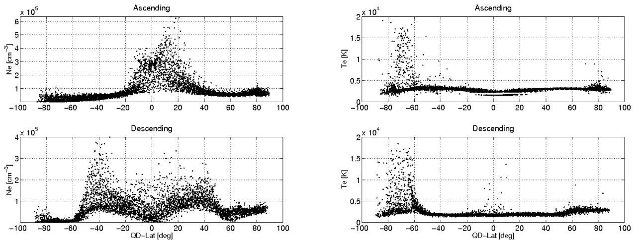
Figure 0-18: The panels shown the electron density (left) and temperature (right) profile as a function of QD Latitudes for the last week of operation. The analysis is made separately for ascending (upper panels) and descending (bottom panels) orbits.
