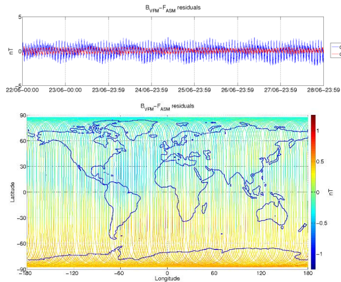
Figure 3-5: ASM-VFM residuals for S/C A, during monitoring period 22/06-28/06. In top figure are plotted: difference between |B_{VFM}| and F_{ASM} (without dB_{Sun} correction) (blue colour), and the residuals with dB_{Sun} corrections (red colour). In bottom figure residuals are presented on the world map.
