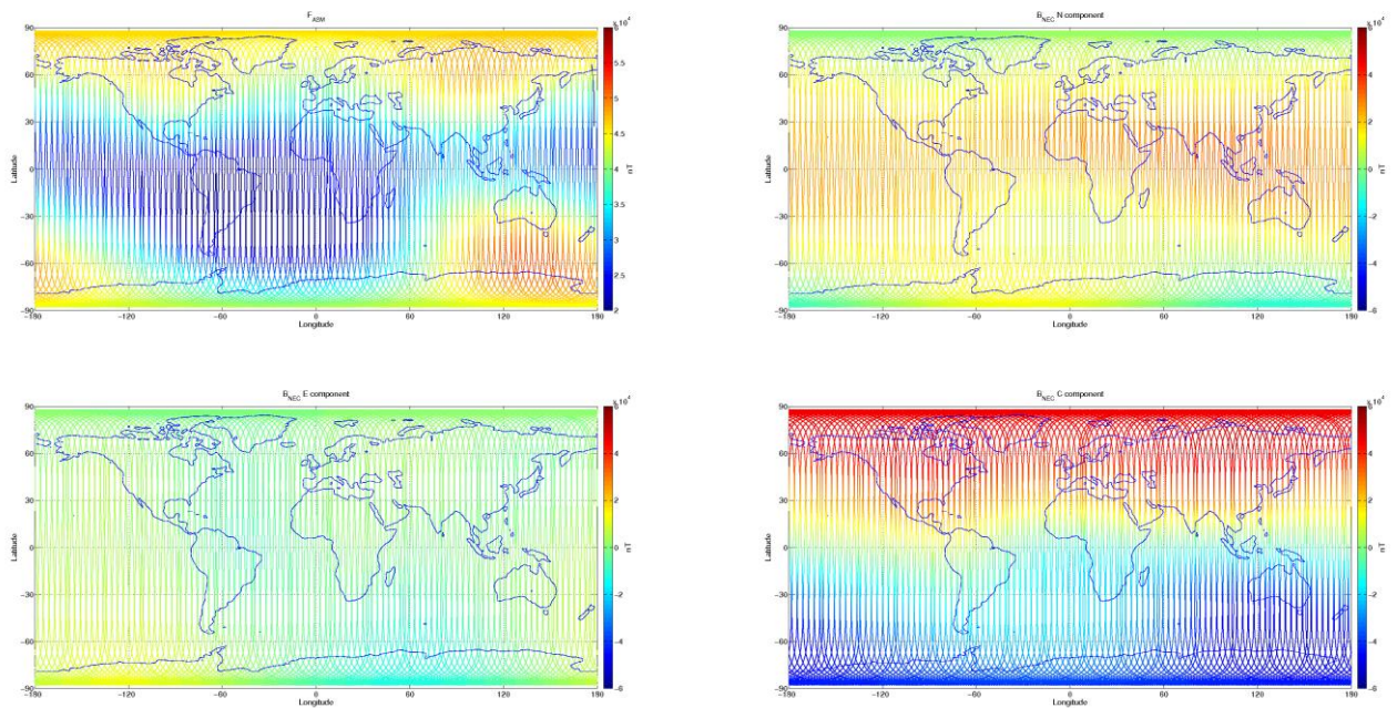
Figure 3-8: S/C B, world map plots of the geomagnetic field and components measured during monitoring period 22/06-28/06. From top to bottom: F-magnetic field from ASM measurement, B_{NEC} components (North, East, and Centre) of magnetic field from VFM measurement.
