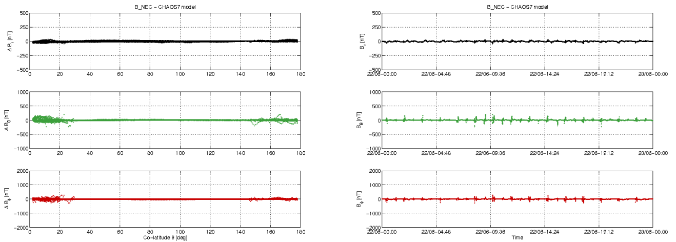
Figure 3-11: S/C B day 22.06: time series of B_{NEC} - B_{Chaos} residuals (right) and B_{NEC} - B_{Chaos} vs colatitude (left).
