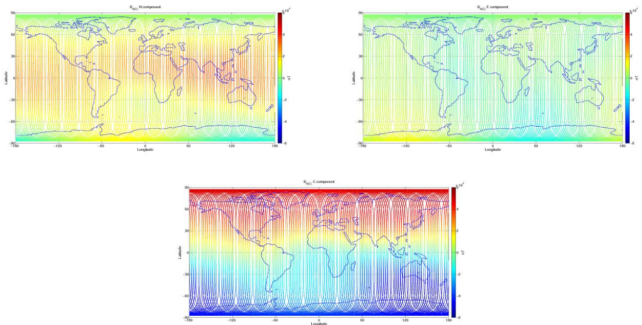
Figure 3-9: S/C C, world map plots of the geomagnetic field and components measured during monitoring period 22/06-28/06. From top to bottom: B_{NEC} components (North, East, and Centre) of magnetic field from VFM measurement.
