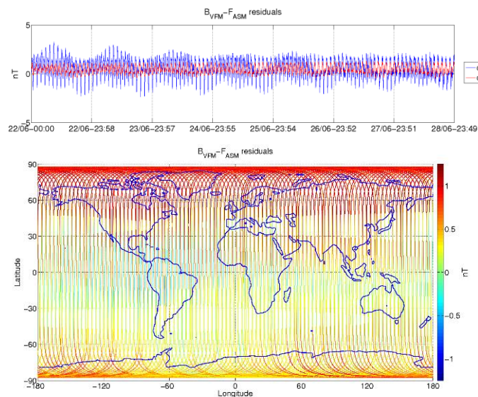
Figure 3-6: ASM-VFM residuals for S/C B, during monitoring period 22/06-28/06. In top figure are plotted: difference between |B_{VFM}| and F_{ASM} (without dB_{Sun} correction) (blue colour), and the residuals with dB_{Sun} corrections (red colour). In bottom figure residuals are presented on the world map.
