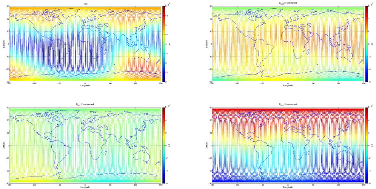
Figure 3-7: S/C A, world map plots of the geomagnetic field and components measured during monitoring period 22/06-28/06. From top to bottom: F-magnetic field from ASM measurement, B_{NEC} components (North, East, and Centre) of magnetic field from VFM measurement.
