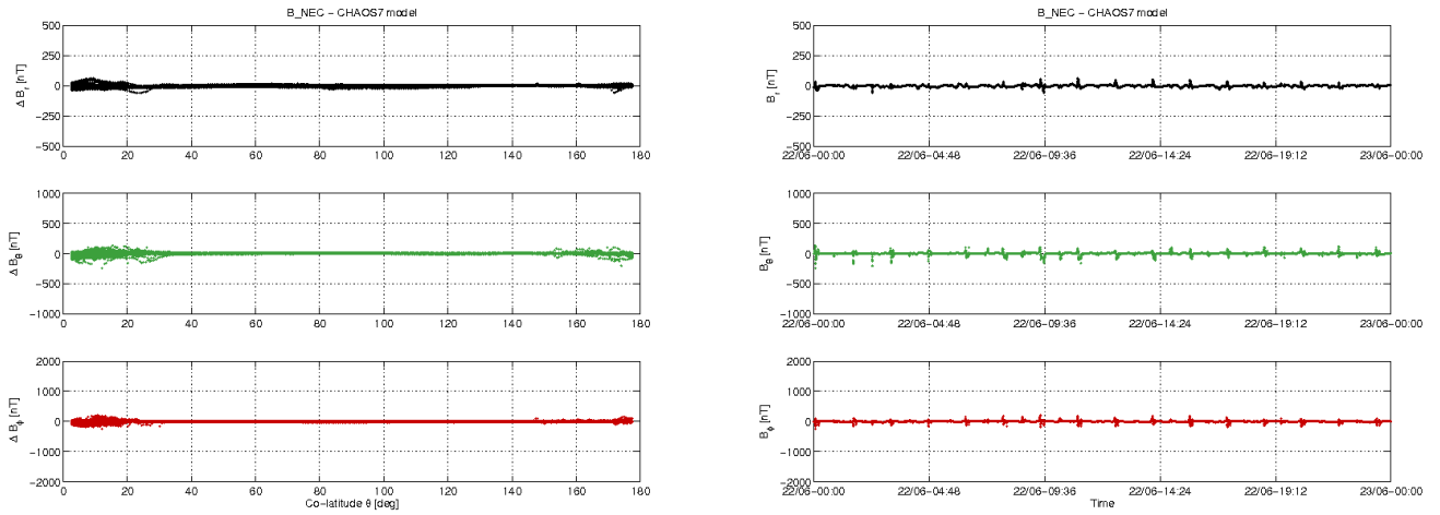
Figure 3-10: S/C A day 22.06: time series of B_{NEC} - B_{Chaos} residuals (right) and B_{NEC} - B_{Chaos} vs colatitude (left).
