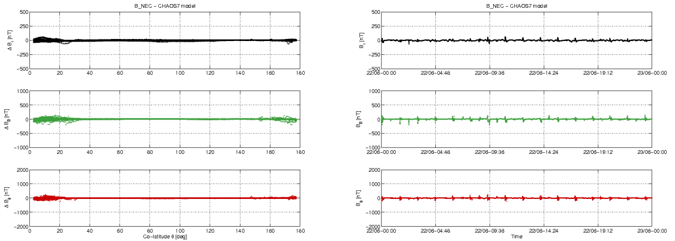
Figure 3-12: S/C C day 22.06: time series of B_{NEC} - B_{Chaos} residuals (right) and B_{NEC} - B_{Chaos} vs colatitude (left).
