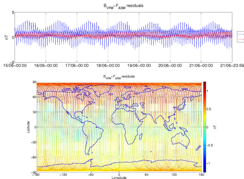
Figure 3-6: ASM-VFM residuals for S/C B, during monitoring period 15/06-21/06. In top figure are plotted: difference between |B_{VFM}| and F_{ASM} (without dB_{Sun} correction) (blue colour), and the residuals with dB_{Sun} corrections (red colour). In bottom figure residuals are presented on the world map.
