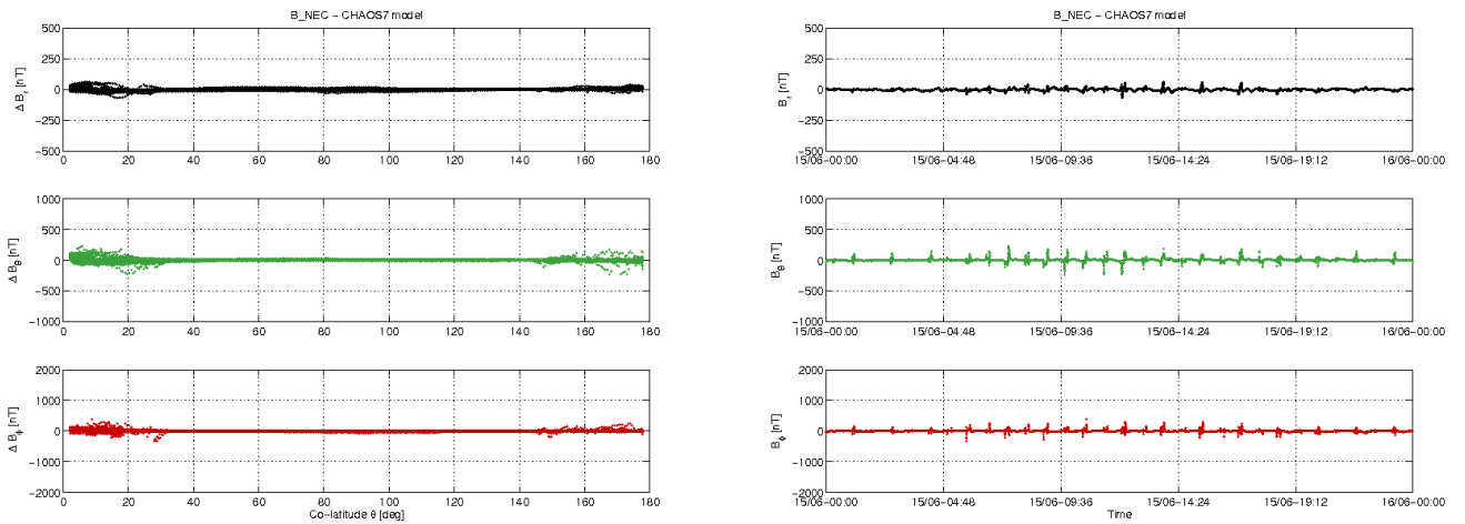
Figure 3-11: S/C B day 15.06: time series of B_{NEC} - B_{Chaos} residuals (right) and B_{NEC} - B_{Chaos} vs colatitude (left).
