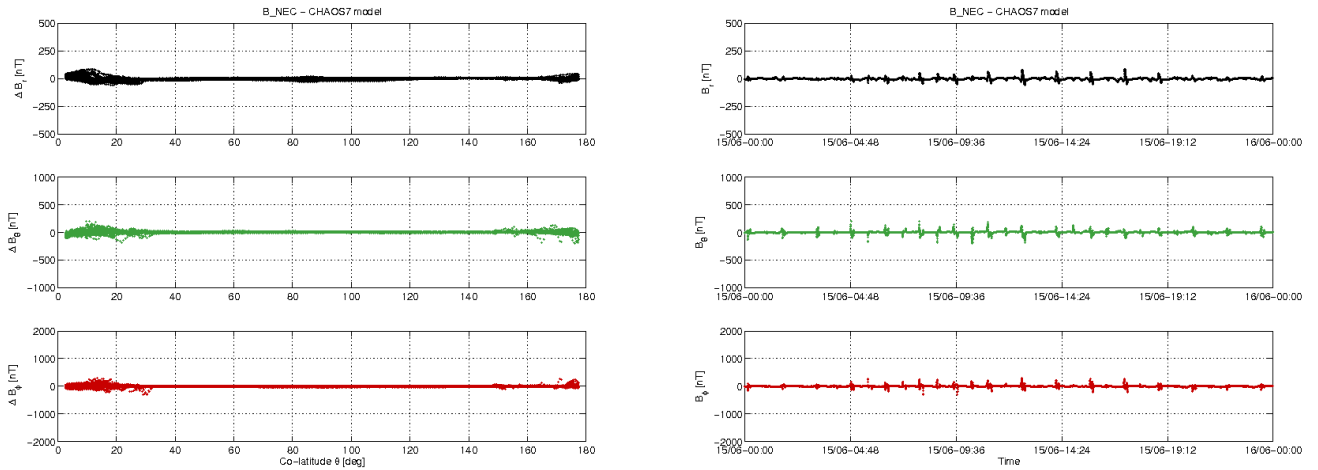
Figure 3-12: S/C C day 15.06: time series of B_{NEC} - B_{Chaos} residuals (right) and B_{NEC} - B_{Chaos} vs colatitude (left).
