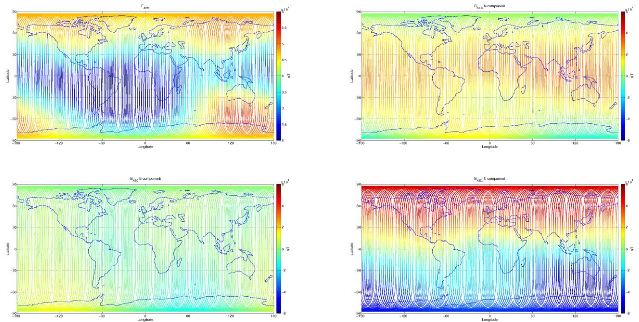
Figure 3-7: S/C A, world map plots of the geomagnetic field and components measured during monitoring period 15/06-21/06. From top to bottom: F-magnetic field from ASM measurement, B_{NEC} components (North, East, and Centre) of magnetic field from VFM measurement.
