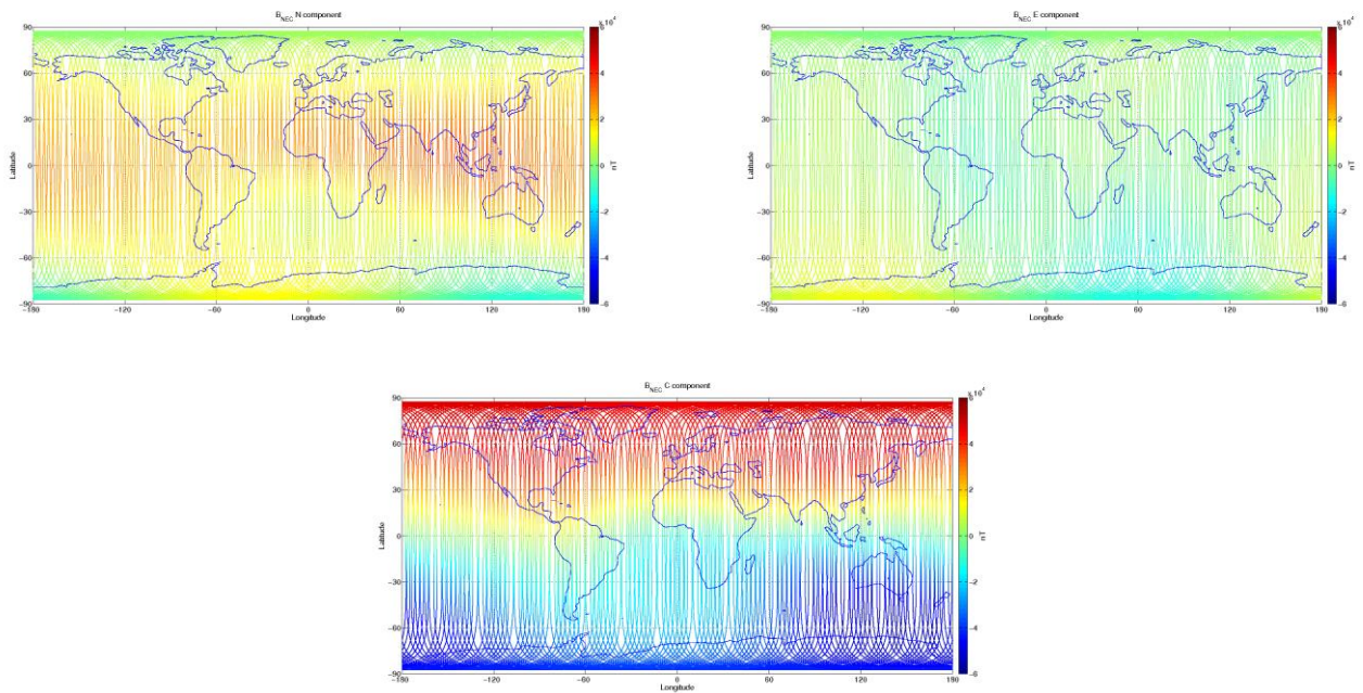
Figure 3-9: S/C C, world map plots of the geomagnetic field and components measured during monitoring period 15/06-21/06. From top to bottom: B_{NEC} components (North, East, and Centre) of magnetic field from VFM measurement.
