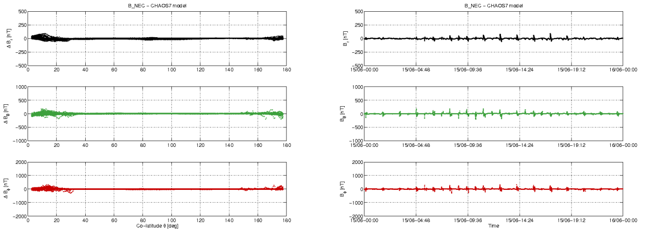
Figure 3-10: S/C A day 15.06: time series of B_{NEC} - B_{Chaos} residuals (right) and B_{NEC} - B_{Chaos} vs colatitude (left).
