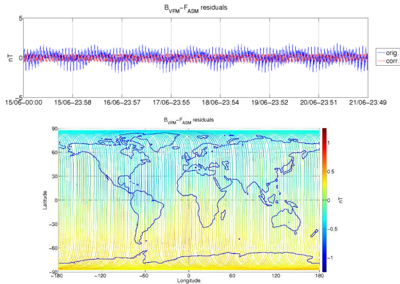
Figure 3-5: ASM-VFM residuals for S/C A, during monitoring period 15/06-21/06. In top figure are plotted: difference between |B_{VFM}| and F_{ASM} (without dB_{Sun} correction) (blue colour), and the residuals with dB_{Sun} corrections (red colour). In bottom figure residuals are presented on the world map.
