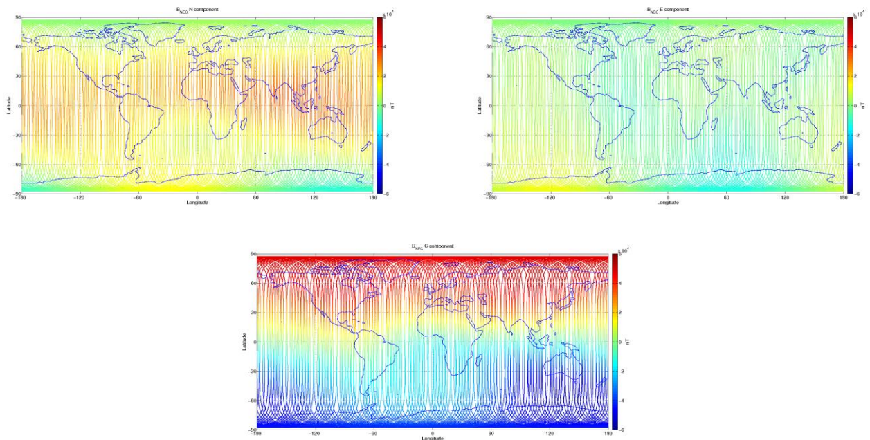
Figure 3-9: S/C C, world map plots of the geomagnetic field and components measured during monitoring period 08/06-14/06. From top to bottom: B_{NEC} components (North, East, and Centre) of magnetic field from VFM measurement.
