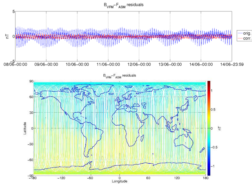
Figure 3-5: ASM-VFM residuals for S/C A, during monitoring period 08/06-14/06. In top figure are plotted: difference between |B_{VFM}| and F_{ASM} (without dB_{Sun} correction) (blue colour), and the residuals with dB_{Sun} corrections (red colour). In bottom figure residuals are presented on the world map.
