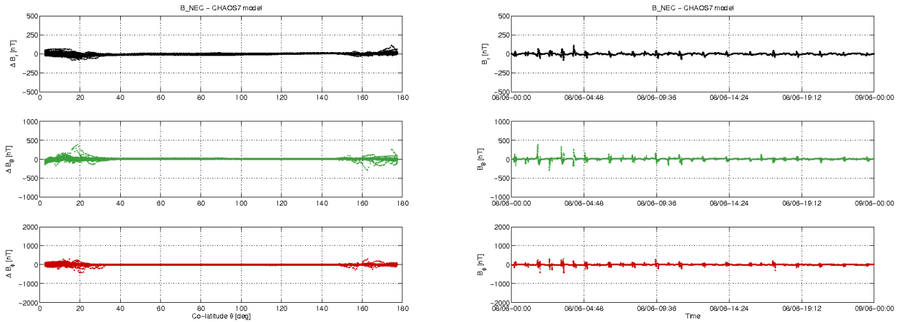
Figure 3-12: S/C C day 08.06: time series of B_{NEC} - B_{Chaos} residuals (right) and B_{NEC} - B_{Chaos} vs colatitude (left).
