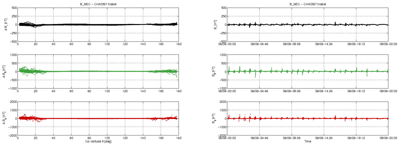
Figure 3-11: S/C B day 08.06: time series of B_{NEC} - B_{Chaos} residuals (right) and B_{NEC} - B_{Chaos} vs colatitude (left).
