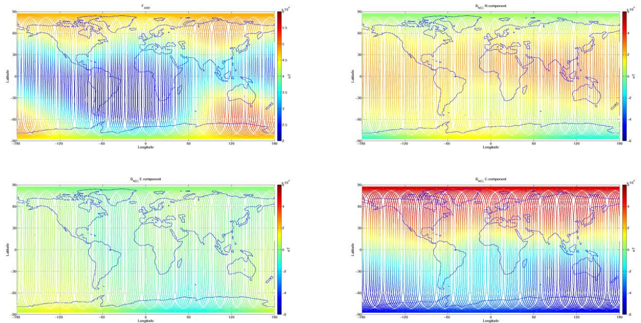
Figure 3-7: S/C A, world map plots of the geomagnetic field and components measured during monitoring period 08/06-14/06. From top to bottom: F-magnetic field from ASM measurement, B_{NEC} components (North, East, and Centre) of magnetic field from VFM measurement.
