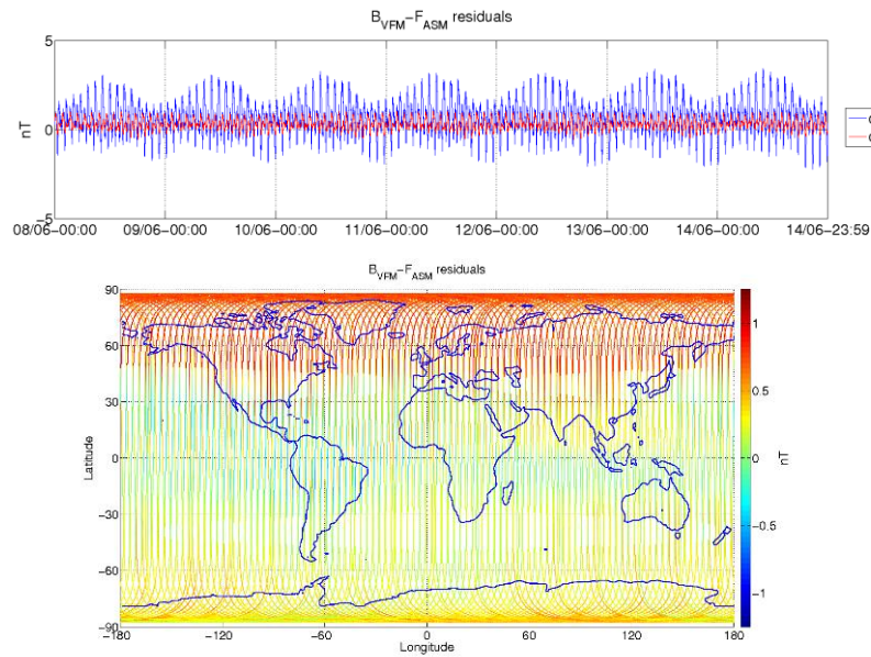
Figure 3-6: ASM-VFM residuals for S/C B, during monitoring period 08/06-14/06. In top figure are plotted: difference between |B_{VFM}| and F_{ASM} (without dB_{Sun} correction) (blue colour), and the residuals with dB_{Sun} corrections (red colour). In bottom figure residuals are presented on the world map.
