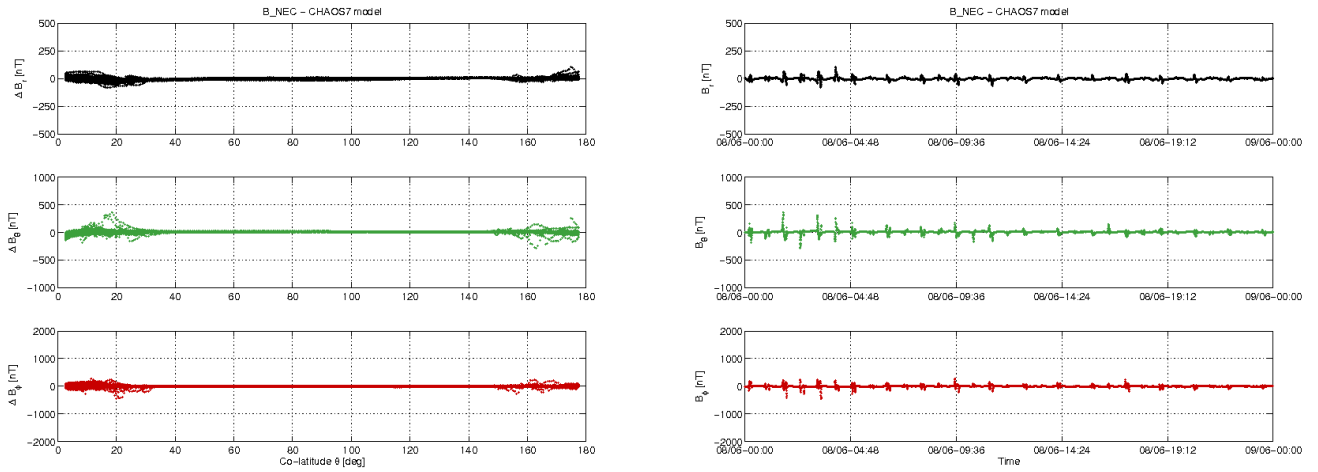
Figure 3-10: S/C A day 08.06: time series of B_{NEC} - B_{Chaos} residuals (right) and B_{NEC} - B_{Chaos} vs colatitude (left).
