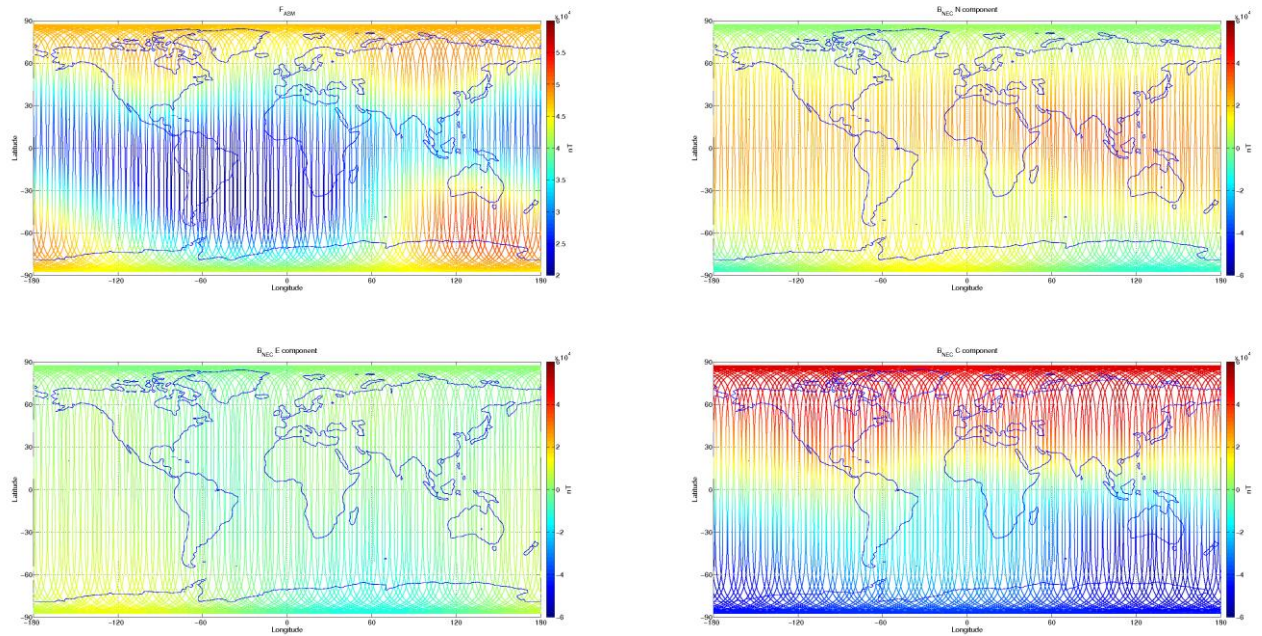
Figure 3-7: S/C A, world map plots of the geomagnetic field and components measured during monitoring period 01/06-07/06. From top to bottom: F-magnetic field from ASM measurement, B_{NEC} components (North, East, and Centre) of magnetic field from VFM measurement.
