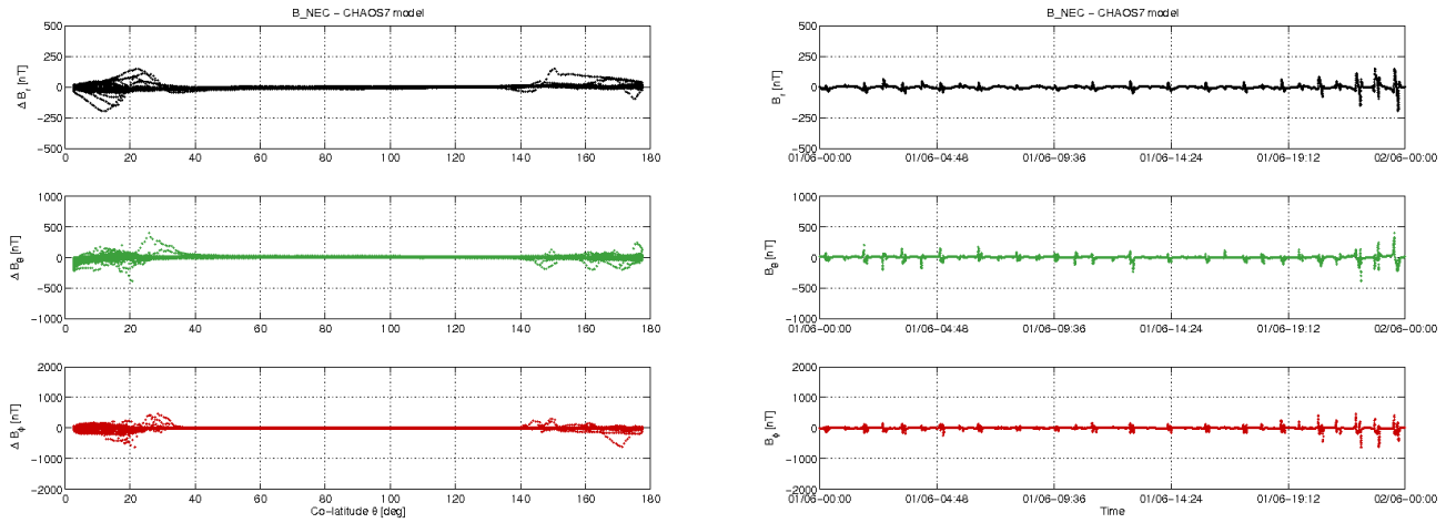
Figure 3-10: S/C A day 01.06: time series of B_{NEC} - B_{Chaos} residuals (right) and B_{NEC} - B_{Chaos} vs colatitude (left).
