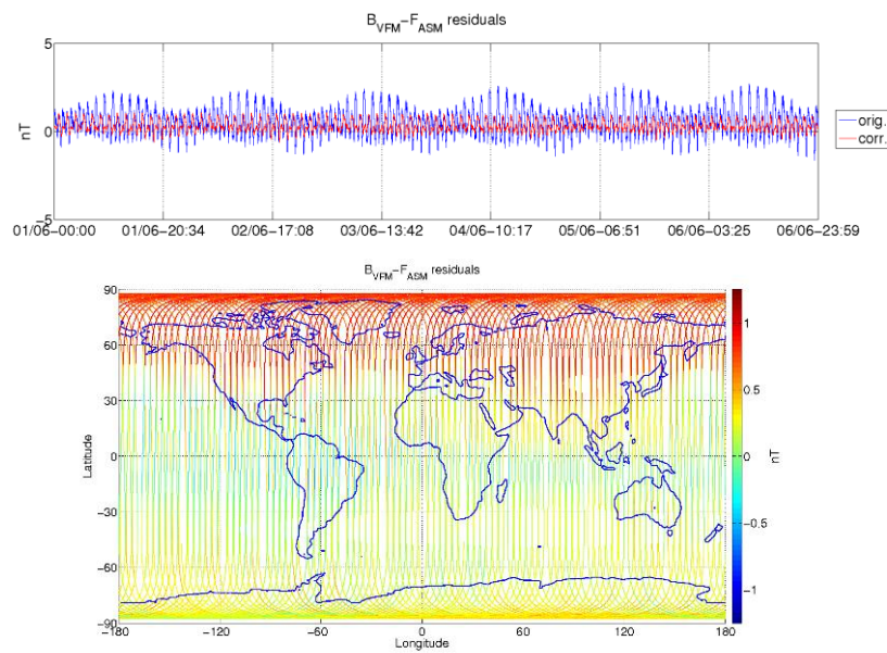
Figure 3-6: ASM-VFM residuals for S/C B, during monitoring period 01/06-07/06. In top figure are plotted: difference between |B_{VFM}| and F_{ASM} (without dB_{Sun} correction) (blue colour), and the residuals with dB_{Sun} corrections (red colour). In bottom figure residuals are presented on the world map.
