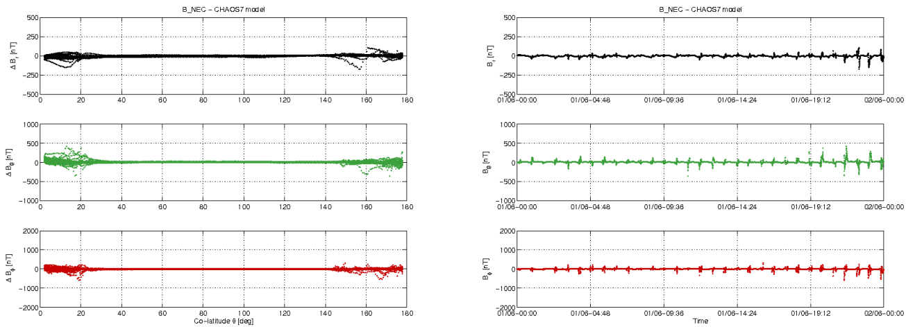
Figure 3-11: S/C B day 01.06: time series of B_{NEC} - B_{Chaos} residuals (right) and B_{NEC} - B_{Chaos} vs colatitude (left).
