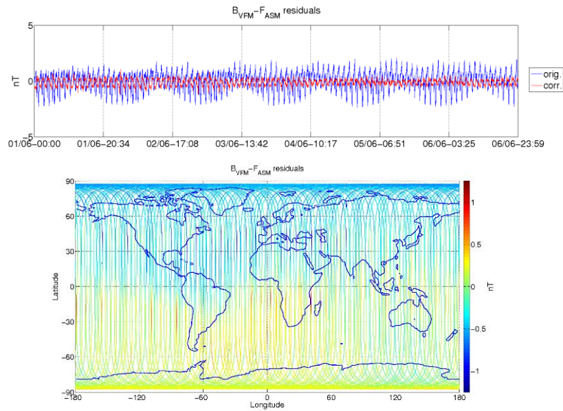
Figure 3-5: ASM-VFM residuals for S/C A, during monitoring period 01/06-07/06. In top figure are plotted: difference between |B_{VFM}| and F_{ASM} (without dB Sun correction) (blue colour), and the residuals with dB Sun corrections (red colour). In bottom figure residuals are presented on the world map.
