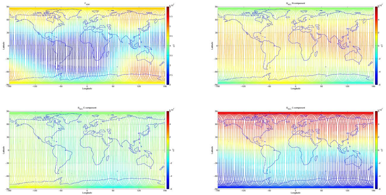
Figure 3-8: S/C B, world map plots of the geomagnetic field and components measured during monitoring period 01/06-07/06. From top to bottom: F-magnetic field from ASM measurement, B_{NEC} components (North, East, and Centre) of magnetic field from VFM measurement.
