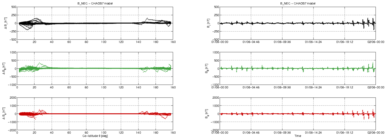
Figure 3-12: S/C C day 01.06: time series of B_{NEC} - B_{Chaos} residuals (right) and B_{NEC} - B_{Chaos} vs colatitude (left).
