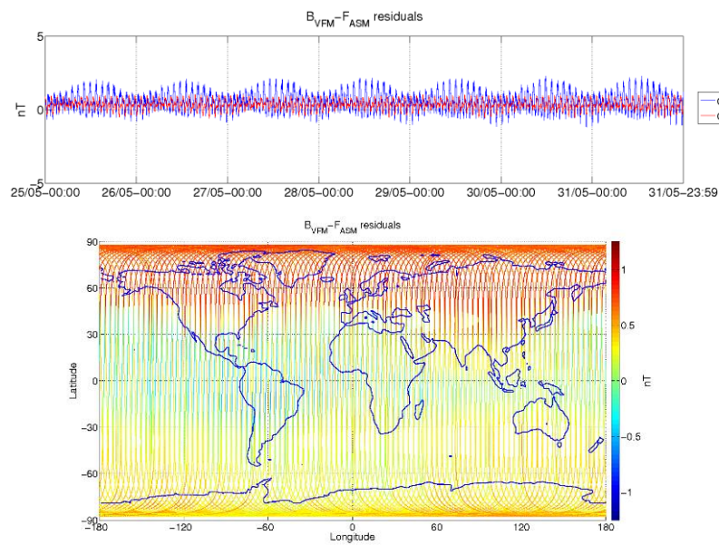
Figure 3-6: ASM-VFM residuals for S/C B, during monitoring period 25/05-31/05. In top figure are plotted: difference between |B_{VFM}| and F_{ASM} (without dB_{Sun} correction) (blue colour), and the residuals with dB_{Sun} corrections (red colour). In bottom figure residuals are presented on the world map.
