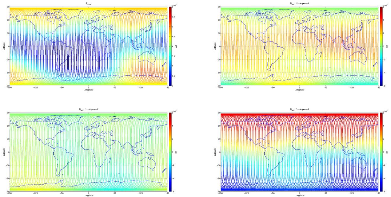
Figure 3-8: S/C B, world map plots of the geomagnetic field and components measured during monitoring period 25/05-31/05. From top to bottom: F-magnetic field from ASM measurement, B_{NEC} components (North, East, and Centre) of magnetic field from VFM measurement.
