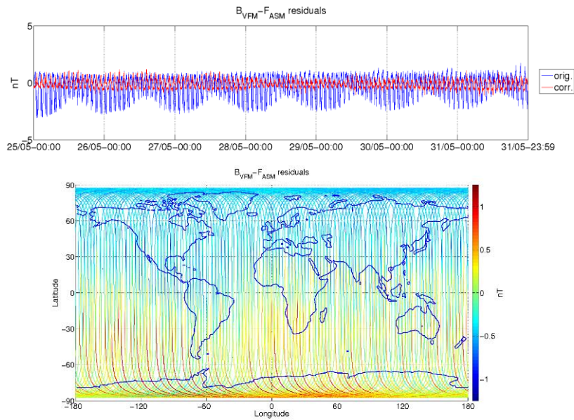
Figure 3-5: ASM-VFM residuals for S/C A, during monitoring period 25/05-31/05. In top figure are plotted: difference between |B_{VFM}| and F_{ASM} (without dB_{Sun} correction) (blue colour), and the residuals with dB_{Sun} corrections (red colour). In bottom figure residuals are presented on the world map.
