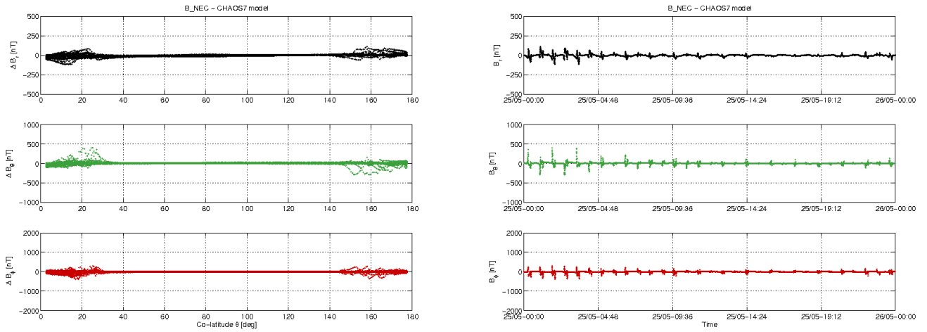
Figure 3-12: S/C C day 25.05: time series of B_{NEC} - B_{Chaos} residuals (right) and B_{NEC} - B_{Chaos} vs colatitude (left).
