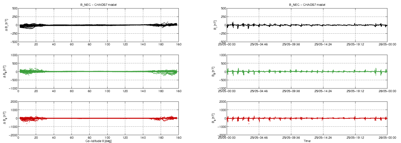
Figure 3-11: S/C B day 25.05: time series of B_{NEC} - B_{Chaos} residuals (right) and B_{NEC} - B_{Chaos} vs colatitude (left).
