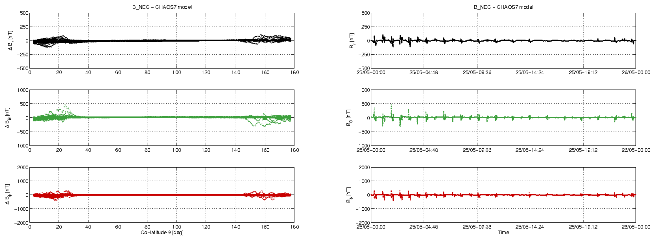
Figure 3-10: S/C A day 25.05: time series of B_{NEC} - B_{Chaos} residuals (right) and B_{NEC} - B_{Chaos} vs colatitude (left).
