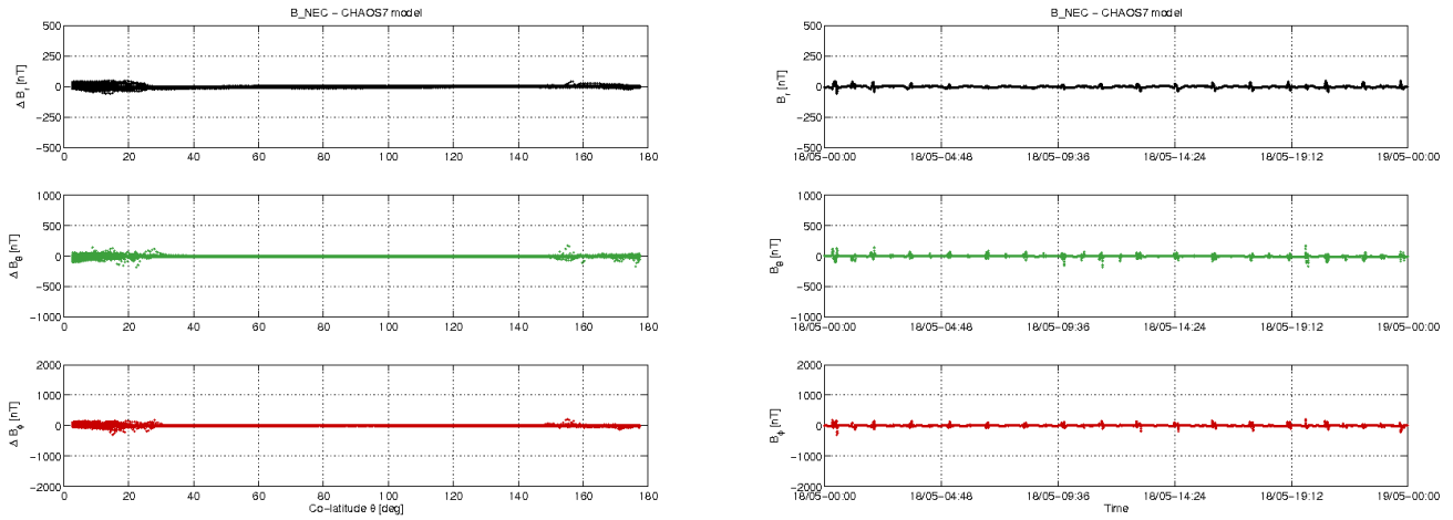
Figure 3-10: S/C A day 18/05: time series of B_{NEC} - B_{Chaos} residuals (right) and B_{NEC} - B_{Chaos} vs colatitude (left).
