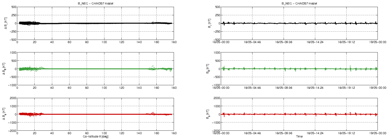
Figure 3-12: S/C C day 18/05: time series of B_{NEC} - B_{Chaos} residuals (right) and B_{NEC} - B_{Chaos} vs colatitude (left).
