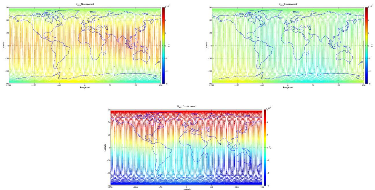
Figure 3-9: S/C C, world map plots of the geomagnetic field and components measured during monitoring period 18/05-24/05. From top to bottom: B_{NEC} components (North, East, and Centre) of magnetic field from VFM measurement.
