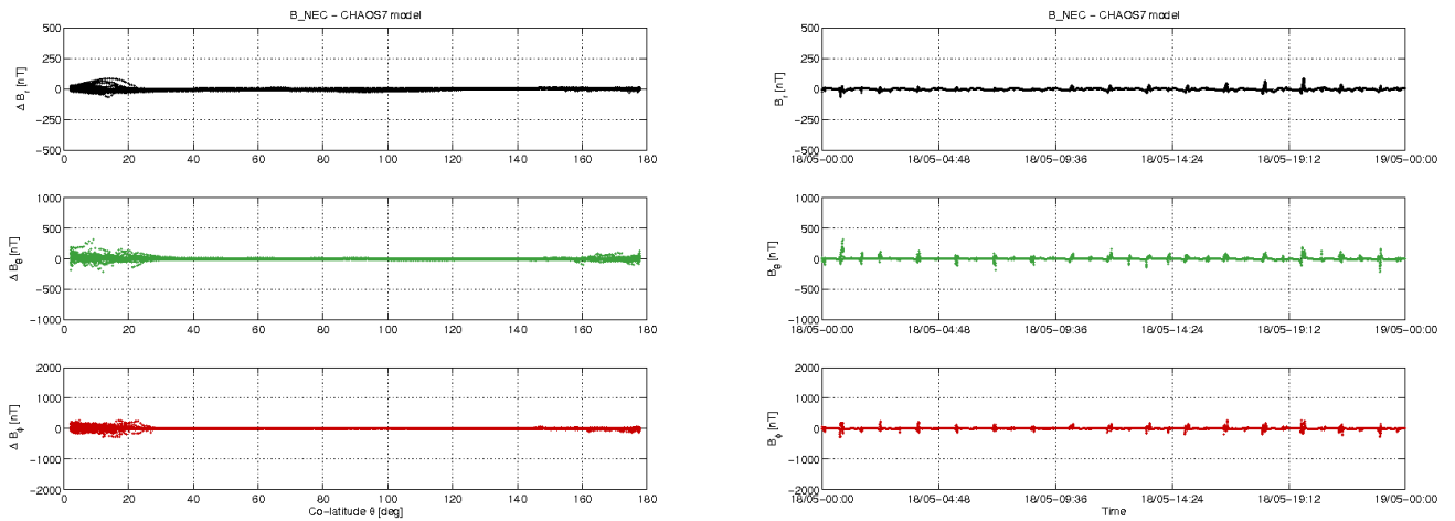
Figure 3-11: S/C B day 18/05: time series of B_{NEC} - B_{Chaos} residuals (right) and B_{NEC} - B_{Chaos} vs colatitude (left).
