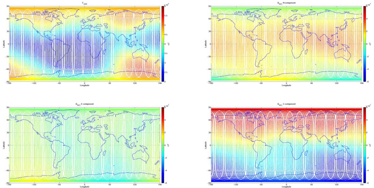
Figure 3-7: S/C A, world map plots of the geomagnetic field and components measured during monitoring period 18/05-24/05. From top to bottom: F-magnetic field from ASM measurement, B_{NEC} components (North, East, and Centre) of magnetic field from VFM measurement.
