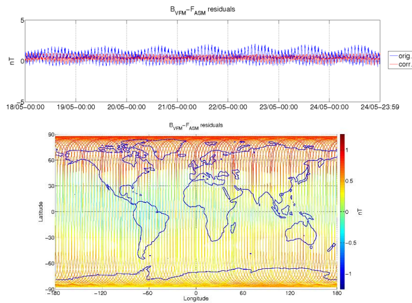
Figure 3-6: ASM-VFM residuals for S/C B, during monitoring period 18/05-24/05. In top figure are plotted: difference between |B_{VFM}| and F_{ASM} (without dB_{Sun} correction) (blue colour), and the residuals with dB_{Sun} corrections (red colour). In bottom figure residuals are presented on the world map.
