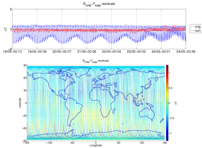
Figure 3-5: ASM-VFM residuals for S/C A, during monitoring period 18/05-24/05. In top figure are plotted: difference between |B_{VFM}| and F_{ASM} (without dB_{Sun} correction) (blue colour), and the residuals with dB_{Sun} corrections (red colour). In bottom figure residuals are presented on the world map.
