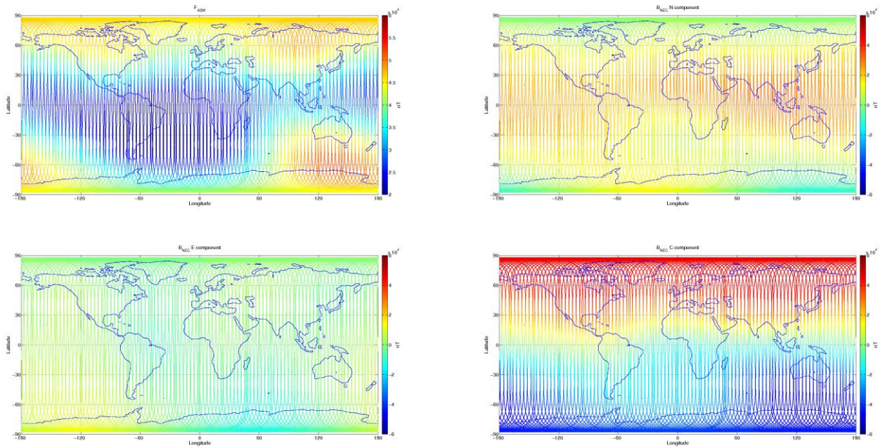
Figure 3-8: S/C B, world map plots of the geomagnetic field and components measured during monitoring period 18/05-24/05. From top to bottom: F-magnetic field from ASM measurement, B_{NEC} components (North, East, and Centre) of magnetic field from VFM measurement.
