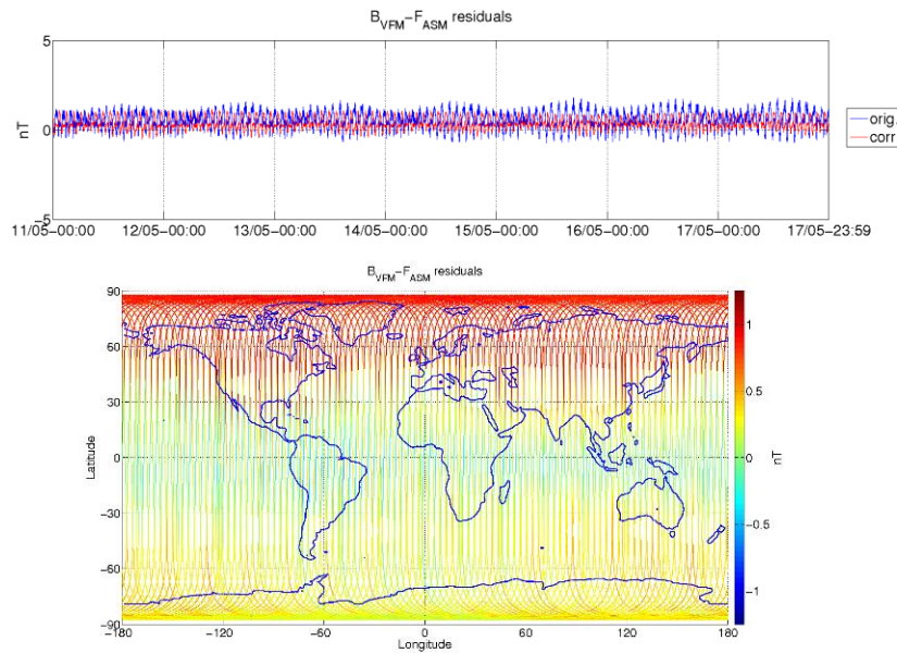
Figure 3-6: ASM-VFM residuals for S/C B, during monitoring period 11/05-17/05. In top figure are plotted: difference between |B_{VFM}| and F_{ASM} (without dB Sun correction) (blue colour), and the residuals with dB Sun corrections (red colour). In bottom figure residuals are presented on the world map.
