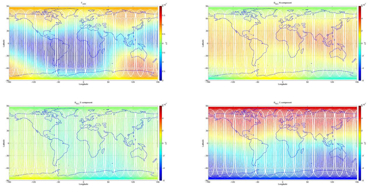
Figure 3-7: S/C A, world map plots of the geomagnetic field and components measured during monitoring period 11/05-17/05. From top to bottom: F-magnetic field from ASM measurement, B_{NEC} components (North, East, and Centre) of magnetic field from VFM measurement.
