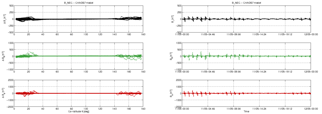
Figure 3-10: S/C A day 11/05: time series of B_{NEC} - B_{Chaos} residuals (right) and B_{NEC} - B_{Chaos} vs colatitude (left).
