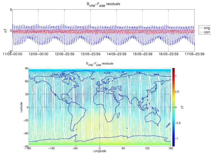
Figure 3-5: ASM-VFM residuals for S/C A, during monitoring period 11/05-17/05. In top figure are plotted: difference between |B_{VFM}| and F_{ASM} (without dB_{Sun} correction) (blue colour), and the residuals with dB_{Sun} corrections (red colour). In bottom figure residuals are presented on the world map.
