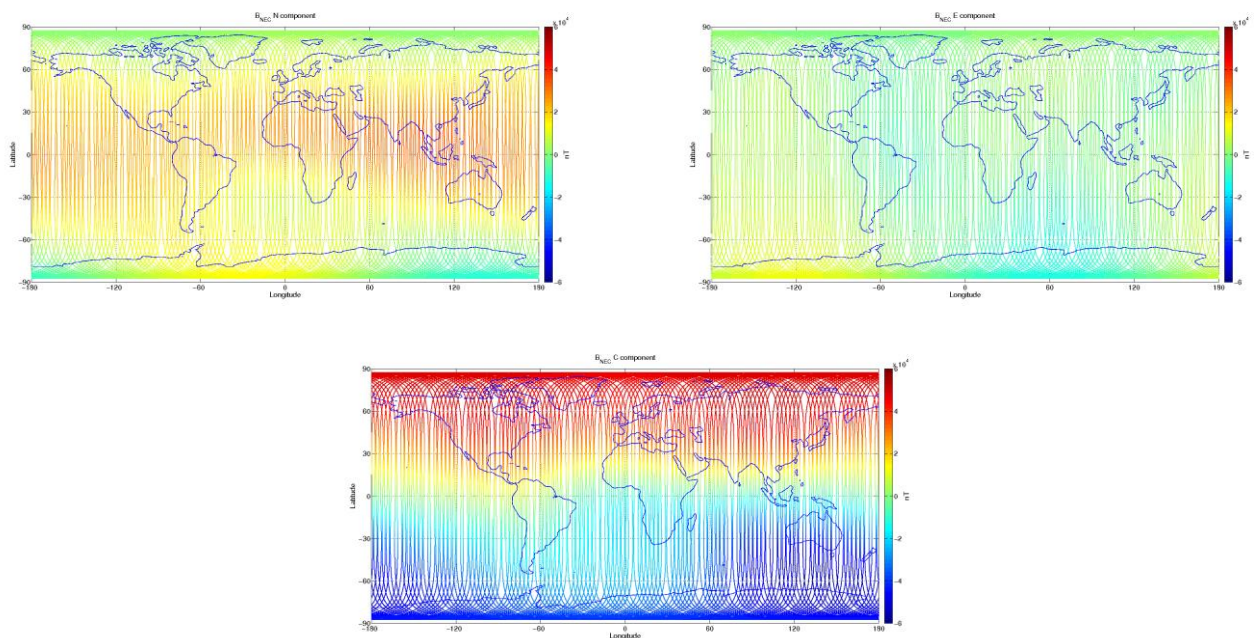
Figure 3-9: S/C C, world map plots of the geomagnetic field and components measured during monitoring period 11/05-17/05. From top to bottom: B_{NEC} components (North, East, and Centre) of magnetic field from VFM measurement.
