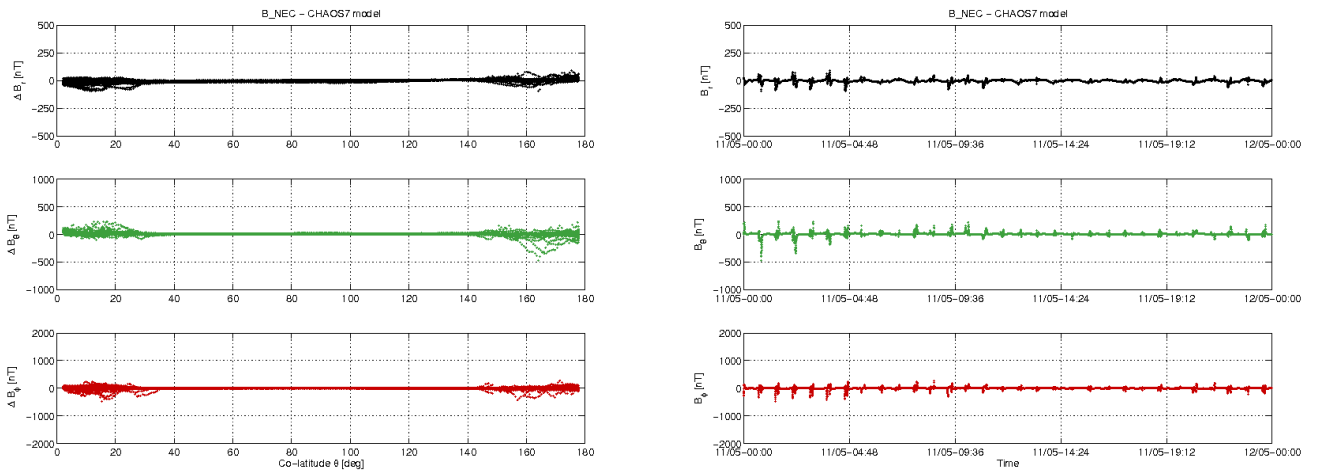
Figure 3-11: S/C B day 11/05: time series of B_{NEC} - B_{Chaos} residuals (right) and B_{NEC} - B_{Chaos} vs colatitude (left).
