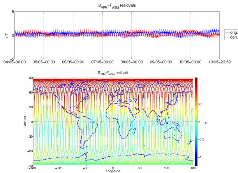
Figure 3-6: ASM-VFM residuals for S/C B, during monitoring period 04/05-10/05. In top figure are plotted: difference between |B_{VFM}| and F_{ASM} (without dB_{Sun} correction) (blue colour), and the residuals with dB_{Sun} corrections (red colour). In bottom figure residuals are presented on the world map.
