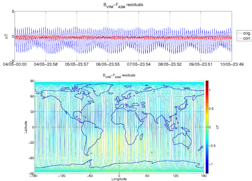
Figure 3-5: ASM-VFM residuals for S/C A, during monitoring period 04/05-10/05. In top figure are plotted: difference between |B_{VFM}| and F_{ASM} (without dB_{Sun} correction) (blue colour), and the residuals with dB_{Sun} corrections (red colour). In bottom figure residuals are presented on the world map.
