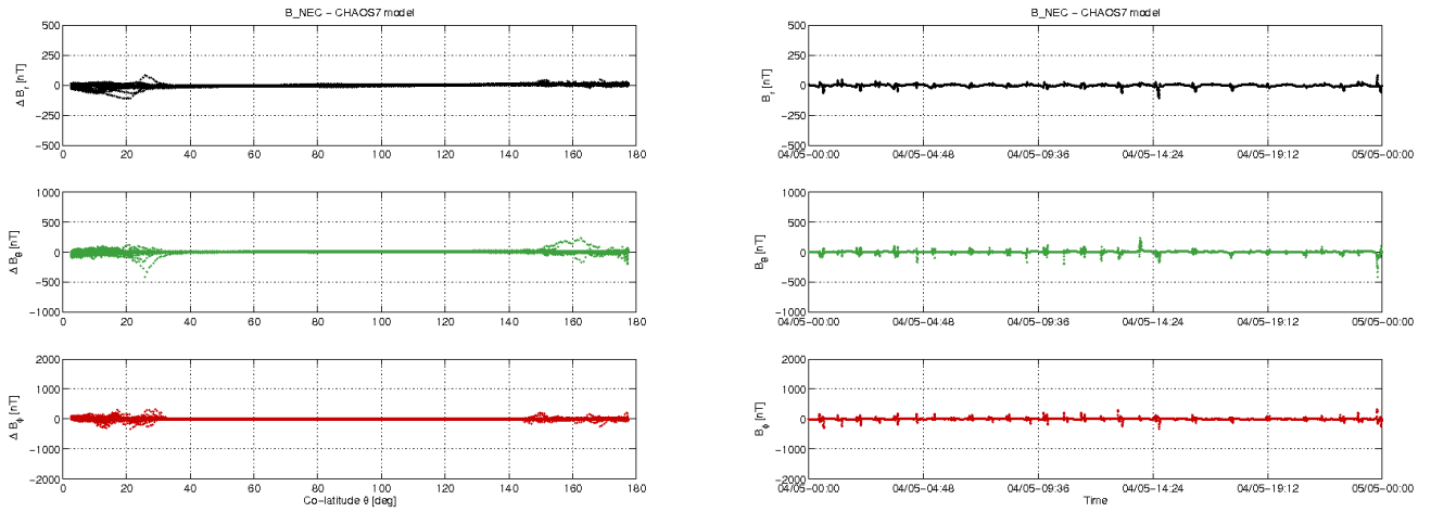
Figure 3-12: S/C C day 04/05: time series of B_{NEC} - B_{Chaos} residuals (right) and B_{NEC} - B_{Chaos} vs colatitude (left).
