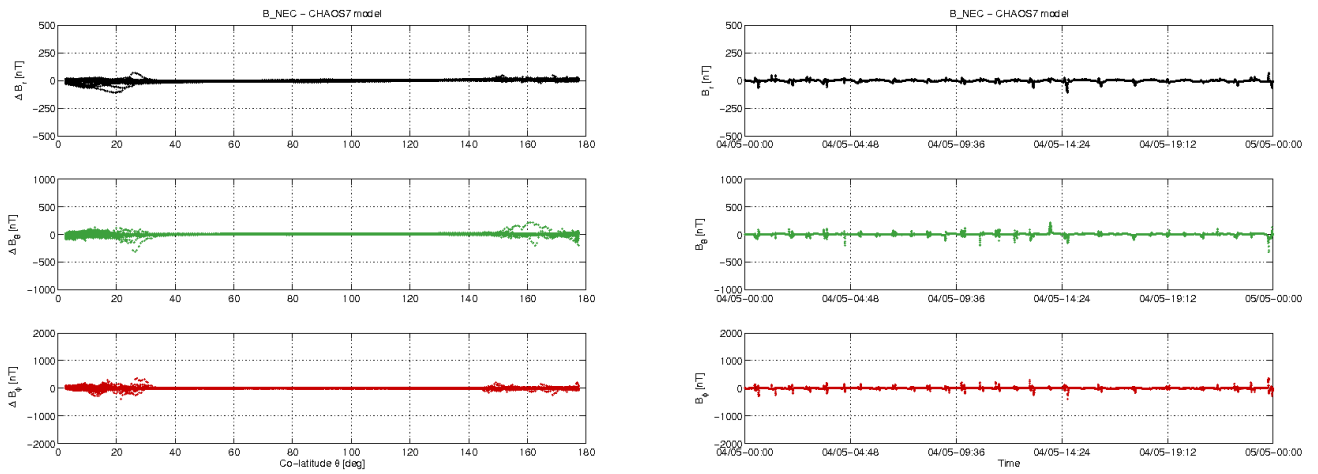
Figure 3-10: S/C A day 04/05: time series of B_{NEC} - B_{Chaos} residuals (right) and B_{NEC} - B_{Chaos} vs colatitude (left).
