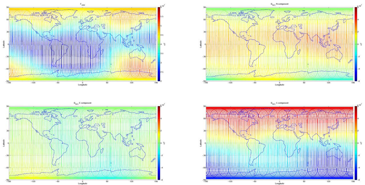
Figure 3-8: S/C B, world map plots of the geomagnetic field and components measured during monitoring period 04/05-10/05. From top to bottom: F-magnetic field from ASM measurement, B_{NEC} components (North, East, and Centre) of magnetic field from VFM measurement.
