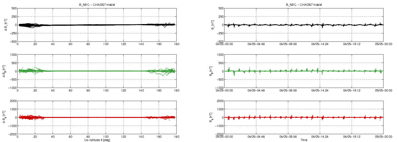
Figure 3-11: S/C B day 04/05 : time series of B_{NEC} - B_{Chaos} residuals (right) and B_{NEC} - B_{Chaos} vs colatitude (left).
