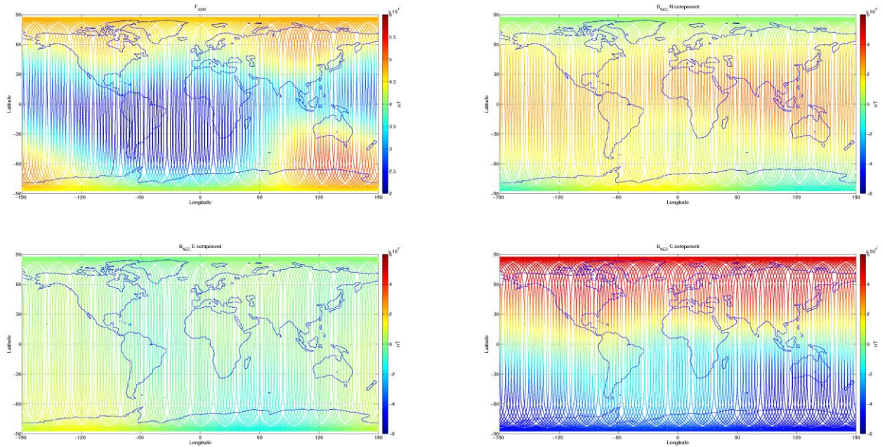
Figure 3-7: S/C A, world map plots of the geomagnetic field and components measured during monitoring period 04/05-10/05. From top to bottom: F-magnetic field from ASM measurement, B_{NEC} components (North, East, and Centre) of magnetic field from VFM measurement.
