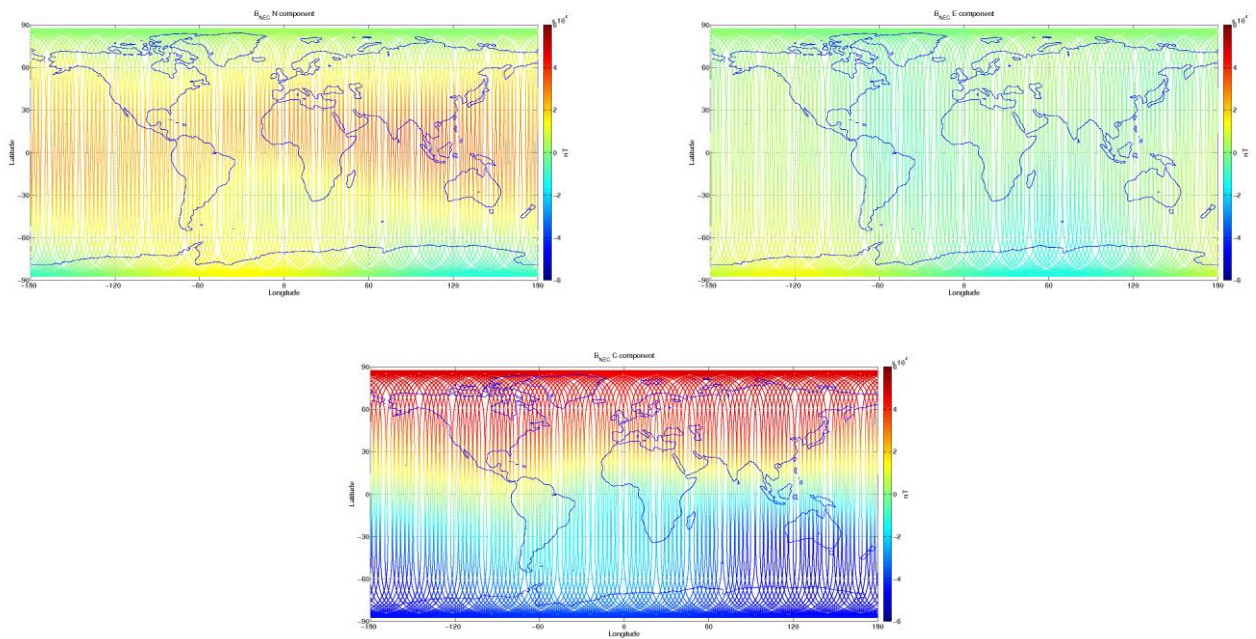
Figure 3-9: S/C C, world map plots of the geomagnetic field and components measured during monitoring period 27/04-03/05. From top to bottom: B_{NEC} components (North, East, and Centre) of magnetic field from VFM measurement.
