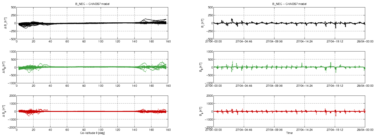
Figure 3-10: S/C A day 27/04: time series of B_{NEC} - B_{Chaos} residuals (right) and B_{NEC} - B_{Chaos} vs colatitude (left).
