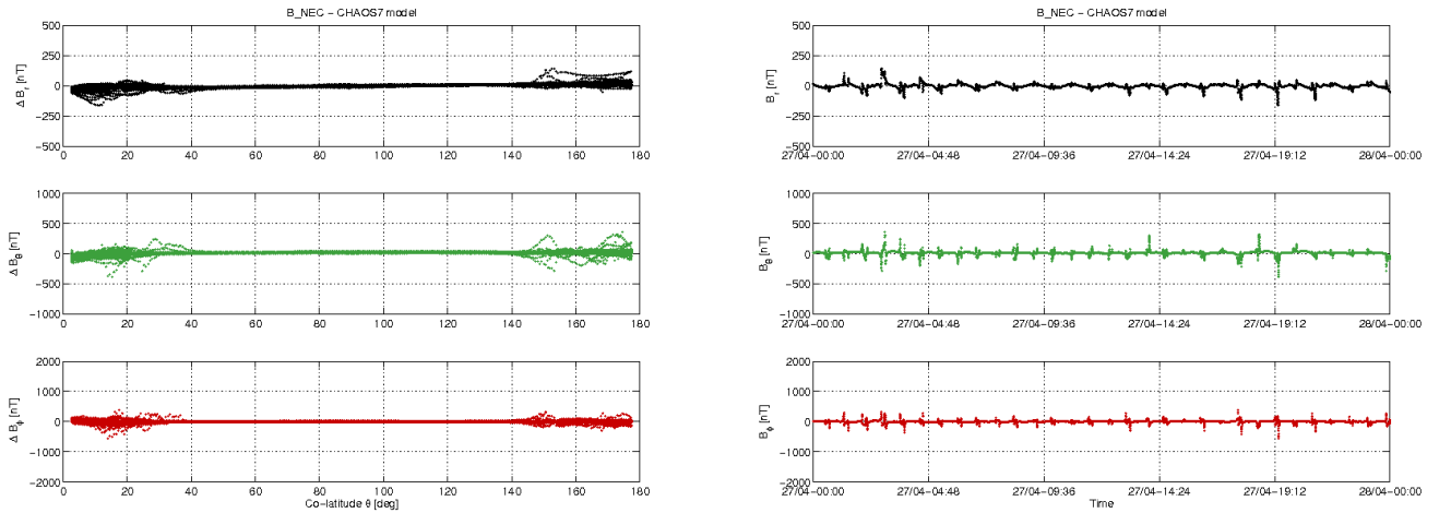
Figure 3-12: S/C C day 27/04: time series of B_{NEC} - B_{Chaos} residuals (right) and B_{NEC} - B_{Chaos} vs colatitude (left).
