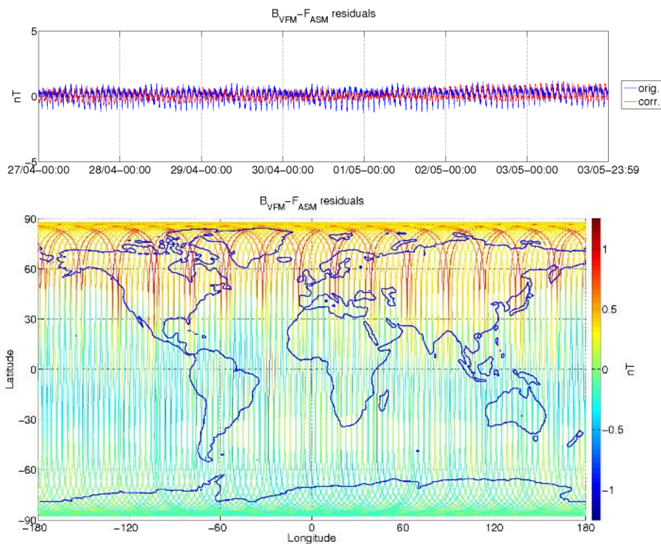
Figure 3-6: ASM-VFM residuals for S/C B, during monitoring period 27/04-03/05. In top figure are plotted: difference between |B_{VFM}| and F_{ASM} (without dB_{Sun} correction) (blue colour), and the residuals with dB_{Sun} corrections (red colour). In bottom figure residuals are presented on the world map.
