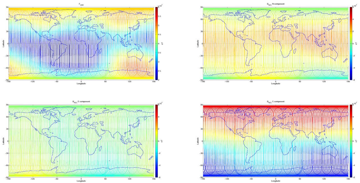
Figure 3-8: S/C B, world map plots of the geomagnetic field and components measured during monitoring period 27/04-03/05. From top to bottom: F-magnetic field from ASM measurement, B_{NEC} components (North, East, and Centre) of magnetic field from VFM measurement.
