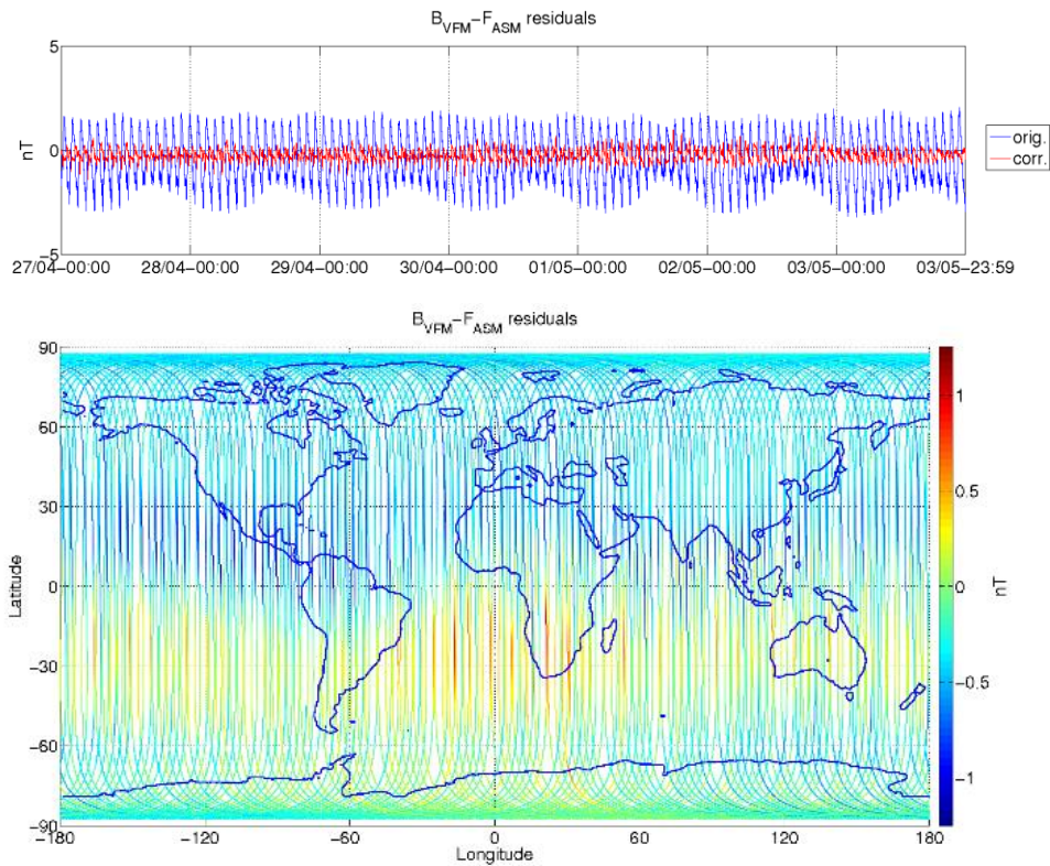
Figure 3-5: ASM-VFM residuals for S/C A, during monitoring period 27/04-03/05. In top figure are plotted: difference between |B_{VFM}| and F_{ASM} (without dB_{Sun} correction) (blue colour), and the residuals with dB_{Sun} corrections (red colour). In bottom figure residuals are presented on the world map.
