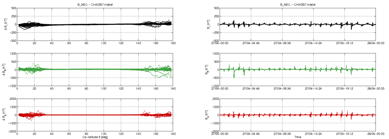
Figure 3-11: S/C B day 27/04: time series of B_{NEC} - B_{Chaos} residuals (right) and B_{NEC} - B_{Chaos} vs colatitude (left).
