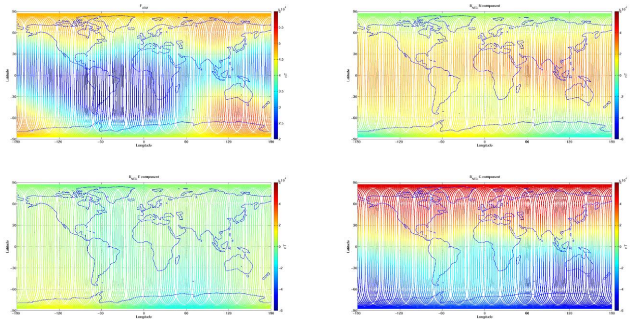
Figure 3-7: S/C A, world map plots of the geomagnetic field and components measured during monitoring period 27/04-03/05. From top to bottom: F-magnetic field from ASM measurement, B_{NEC} components (North, East, and Centre) of magnetic field from VFM measurement.
