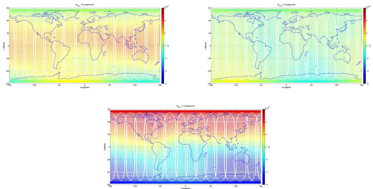
Figure 3-9: S/C C, world map plots of the geomagnetic field and components measured during monitoring period 06/04-12/04. From top to bottom: B_{NEC} components (North, East, and Centre) of magnetic field from VFM measurement.
