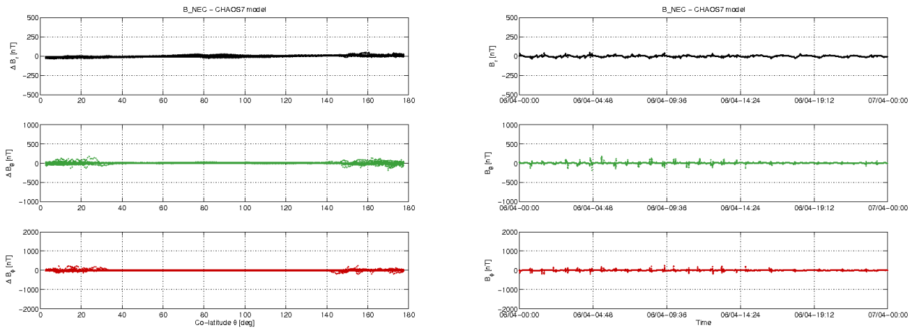
Figure 3-10: S/C A day 06/04: time series of B_{NEC} - B_{Chaos} residuals (right) and B_{NEC} - B_{Chaos} vs colatitude (left).
