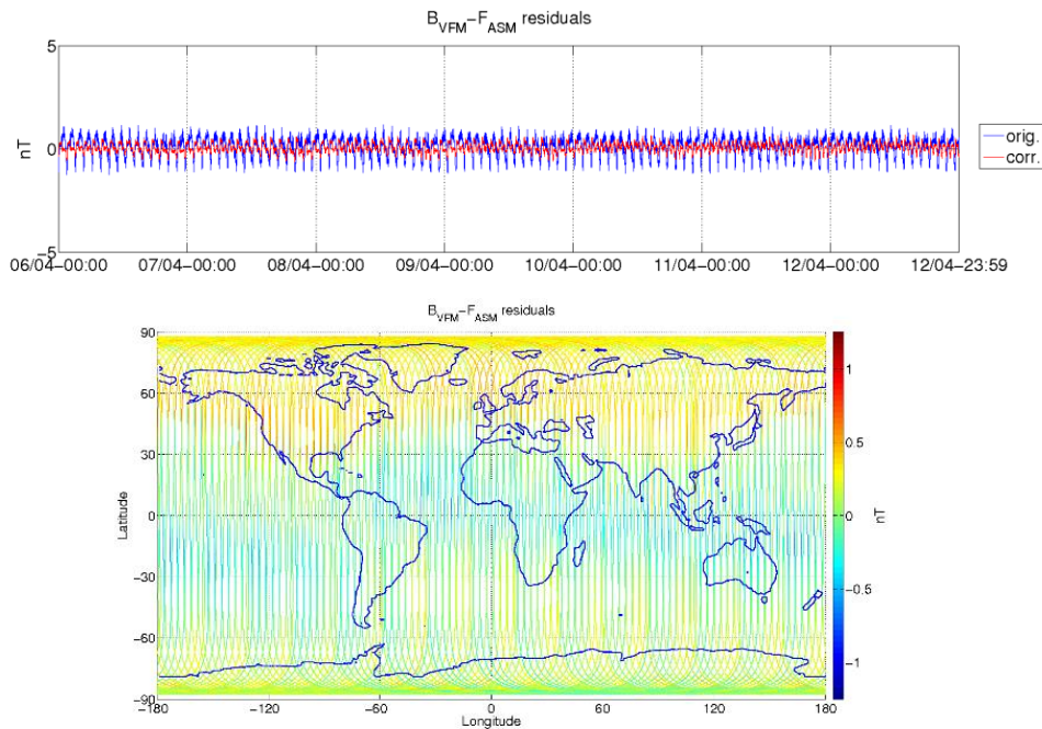
Figure 3-6: ASM-VFM residuals for S/C B, during monitoring period 06/04-12/04. In top figure are plotted: difference between |B_{VFM}| and F_{ASM} (without dB Sun correction) (blue colour), and the residuals with dB Sun corrections (red colour). In bottom figure residuals are presented on the world map.
