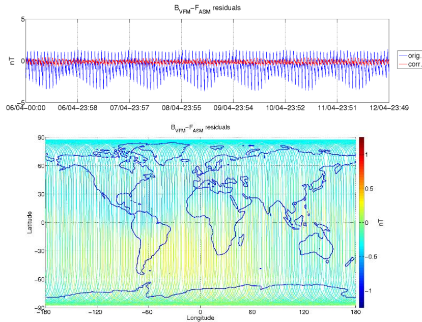
Figure 3-5: ASM-VFM residuals for S/C A, during monitoring period 06/04-12/04. In top figure are plotted: difference between |B_{VFM}| and F_{ASM} (without dB_{Sun} correction) (blue colour), and the residuals with dB_{Sun} corrections (red colour). In bottom figure residuals are presented on the world map.
