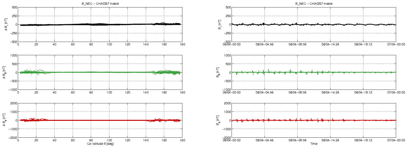
Figure 3-12: S/C C day 06/04: time series of B_{NEC} - B_{Chaos} residuals (right) and B_{NEC} - B_{Chaos} vs colatitude (left).
