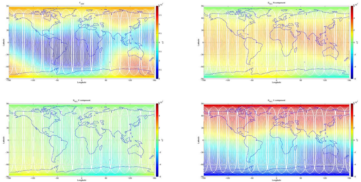
Figure 3-7: S/C A, world map plots of the geomagnetic field and components measured during monitoring period 06/04-12/04. From top to bottom: F-magnetic field from ASM measurement, B_{NEC} components (North, East, and Centre) of magnetic field from VFM measurement.
