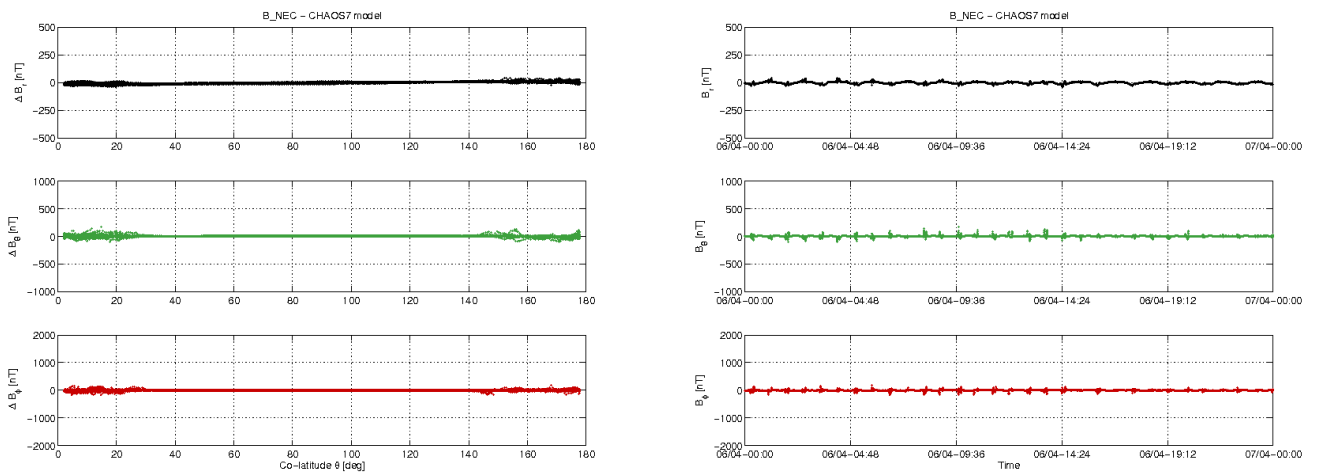
Figure 3-11: S/C B day 06/04: time series of B_{NEC} - B_{Chaos} residuals (right) and B_{NEC} - B_{Chaos} vs colatitude (left).
