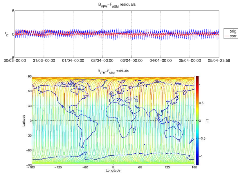
Figure 3-6: ASM-VFM residuals for S/C B, during monitoring period 30/03-05/04. In top figure are plotted: difference between |B_{VFM}| and F_{ASM} (without dB_Sun correction) (blue colour), and the residuals with dB_Sun corrections (red colour). In bottom figure residuals are presented on the world map.
