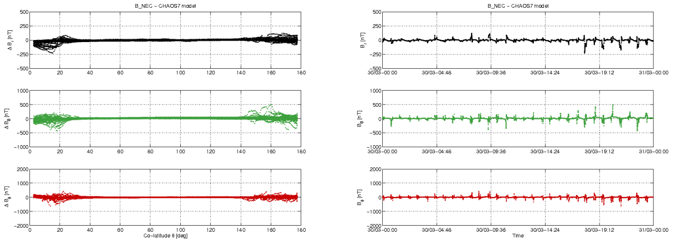
Figure 3-12: S/C C day 30/03: time series of B_{NEC} - B_{Chaos} residuals (right) and B_{NEC} - B_{Chaos} vs colatitude (left).
