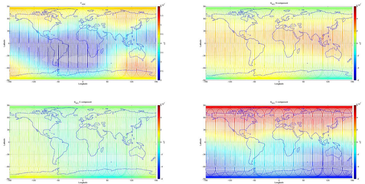
Figure 3-8: S/C B, world map plots of the geomagnetic field and components measured during monitoring period 30/03-05/04. From top to bottom: F-magnetic field from ASM measurement, B_{NEC} components (North, East, and Centre) of magnetic field from VFM measurement.
