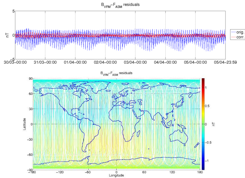
Figure 3-5: ASM-VFM residuals for S/C A, during monitoring period 30/03-05/04. In top figure are plotted: difference between |B_{VFM}| and F_{ASM} (without dB_Sun correction) (blue colour), and the residuals with dB_Sun corrections (red colour). In bottom figure residuals are presented on the world map.
