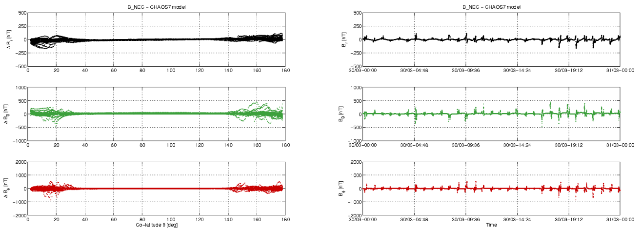
Figure 3-11: S/C B day 30/03: time series of B_{NEC} - B_{Chaos} residuals (right) and B_{NEC} - B_{Chaos} vs colatitude (left).
