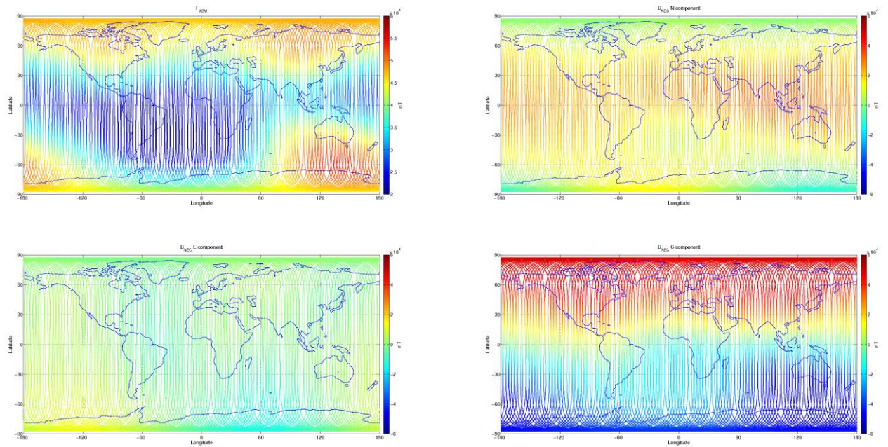
Figure 3-7: S/C A, world map plots of the geomagnetic field and components measured during monitoring period 30/03-05/04. From top to bottom: F-magnetic field from ASM measurement, B_{NEC} components (North, East, and Centre) of magnetic field from VFM measurement.
