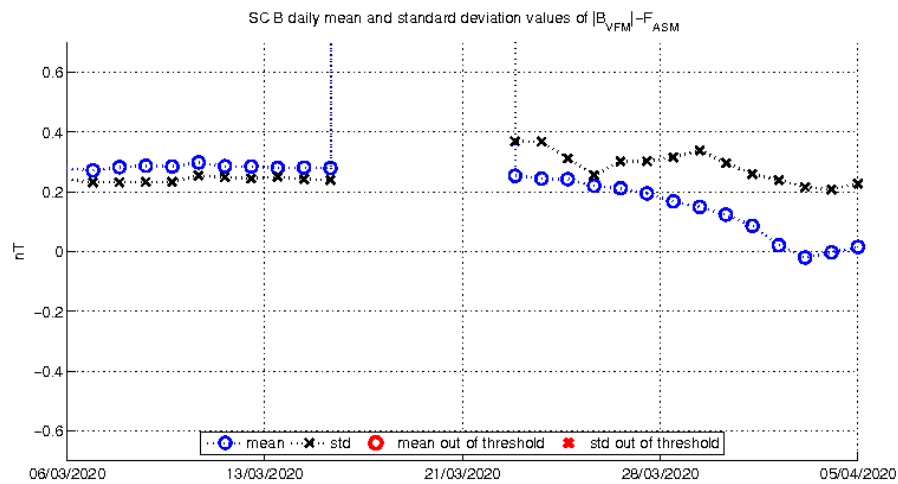
Figure 3-4: Daily mean and standard deviation values of ASM-VFM residuals (defined as dF = |B_{VFM}| - F_{ASM} ) for S/C B. Gap in the data is caused by ASM on Bravo operating in Burst mode that experienced short time gaps. Current L1BOP v3.22 is not able to process AMS burst mode when data gaps occur.
