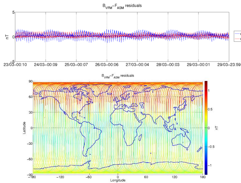
Figure 3-6: ASM-VFM residuals for S/C B, during monitoring period 23/03-29/03. In top figure are plotted: difference between |B_{VFM}| and F_{ASM} (without dB_{Sun} correction) (blue colour), and the residuals with dB_{Sun} corrections (red colour). In bottom figure residuals are presented on the world map.
