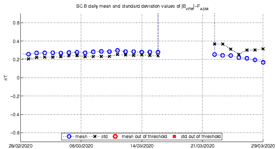
Figure 3-4: Daily mean and standard deviation values of ASM-VFM residuals (defined as dF = |B_{VFM}| - F_{ASM} ) for S/C B. (the gap in the plot reflects ASM Burst mode. L1BOP v3.22 is not able to process Burst mode data with internal gaps)
