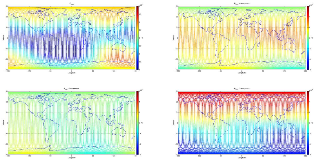
Figure 3-8: S/C B, world map plots of the geomagnetic field and components measured during monitoring period 23/03-29/03. From top to bottom: F-magnetic field from ASM measurement, B_{NEC} components (North, East, and Centre) of magnetic field from VFM measurement.
