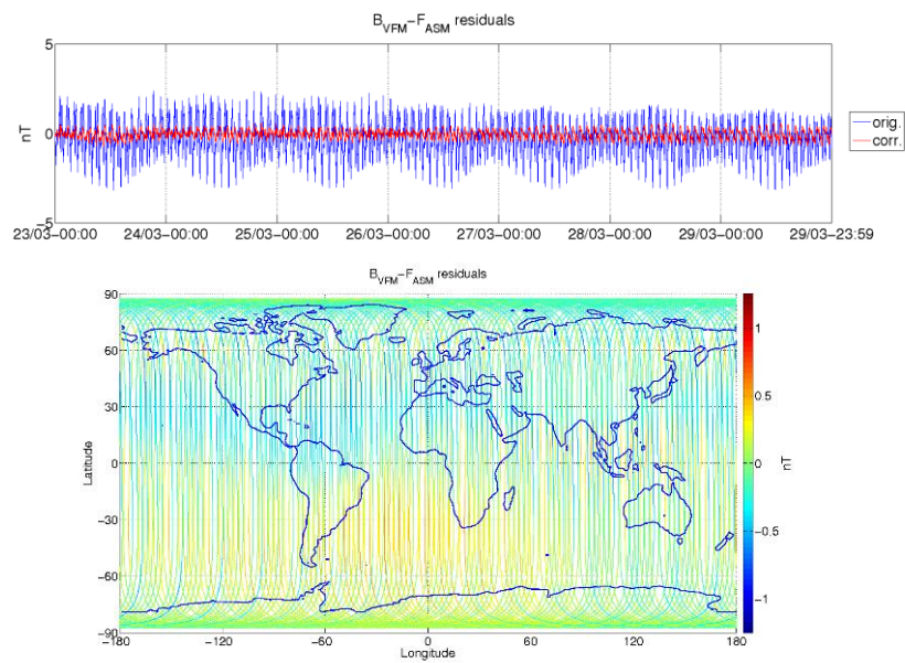
Figure 3-5: ASM-VFM residuals for S/C A, during monitoring period 23/03-29/03. In top figure are plotted: difference between |B_{VFM}| and F_{ASM} (without dB_Sun correction) (blue colour), and the residuals with dB_Sun corrections (red colour). In bottom figure residuals are presented on the world map.
