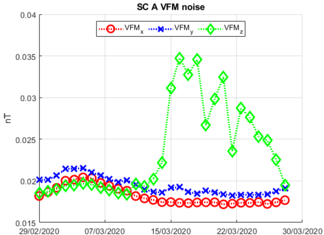
Figure 19 High frequency content. The plot is generated in the following way: data are filtered with high pass Butterworth 3 rd order filter, cut off frequency is set to 5Hz. Then only data in geo-latitude band +/-10deg are selected and daily rms is calculated.
