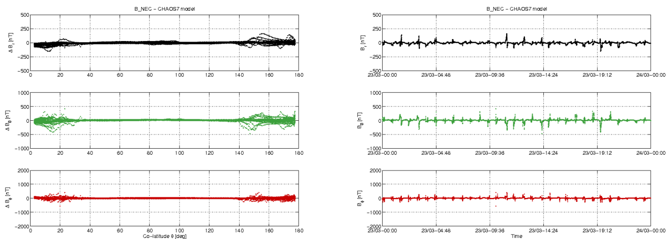
Figure 3-10: S/C A day 23/03: time series of B_{\text{NEC}} - B_{\text{Chaos}} residuals (right) and B_{\text{NEC}} - B_{\text{Chaos}} vs colatitude (left).
