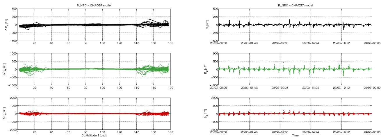
Figure 3-11: S/C B day 23/03: time series of B_{\text{NEC}} - B_{\text{Chaos}} residuals (right) and B_{\text{NEC}} - B_{\text{Chaos}} vs colatitude (left).
