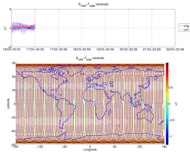
Figure 3-6: ASM-VFM residuals for S/C B, during monitoring period 16/03-22/03. In top figure are plotted: difference between |B_{VFM}| and F_{ASM} (without dB_{Sun} correction) (blue colour), and the residuals with dB_{Sun} corrections (red colour). In bottom figure residuals are presented on the world map.
