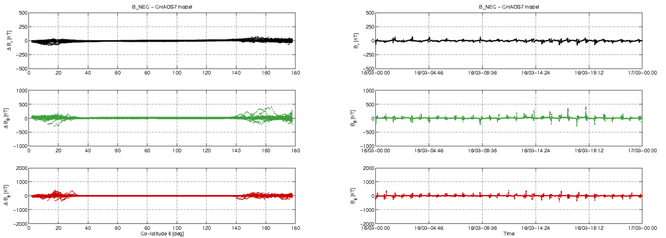
Figure 3-11: S/C B day 16.03 S/C B: time series of B_{NEC} - B_{Chaos} residuals (right) and B_{NEC} - B_{Chaos} vs colatitude (left).
