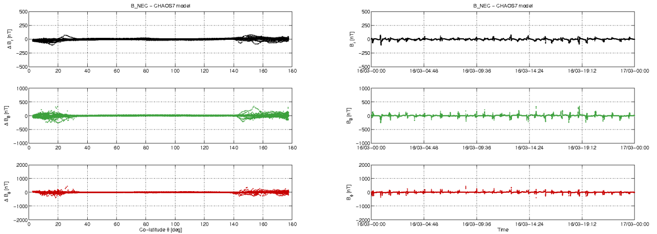
Figure 3-12: S/C C day 1603: time series of B_{NEC} - B_{Chaos} residuals (right) and B_{NEC} - B_{Chaos} vs colatitude (left).
