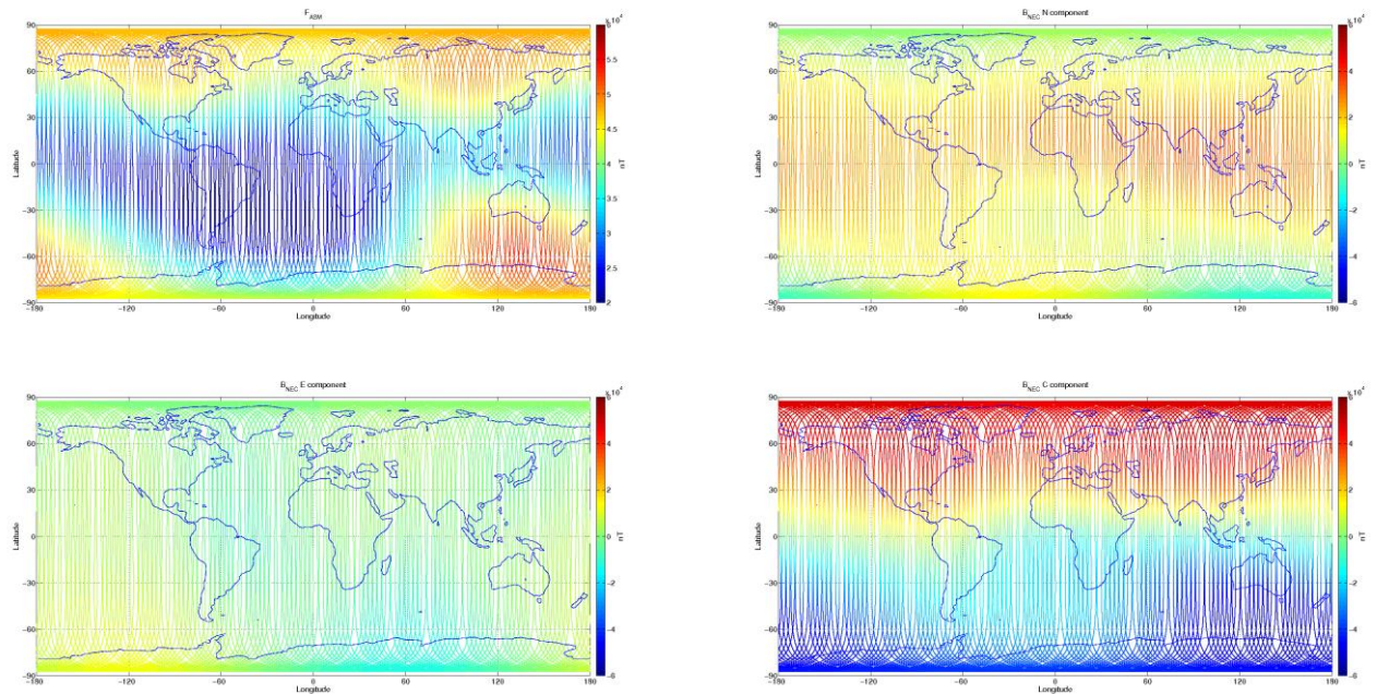
Figure 3-7: S/C A, world map plots of the geomagnetic field and components measured during monitoring period 16/03-22/03. From top to bottom: F-magnetic field from ASM measurement, B_{NEC} components (North, East, and Centre) of magnetic field from VFM measurement.
