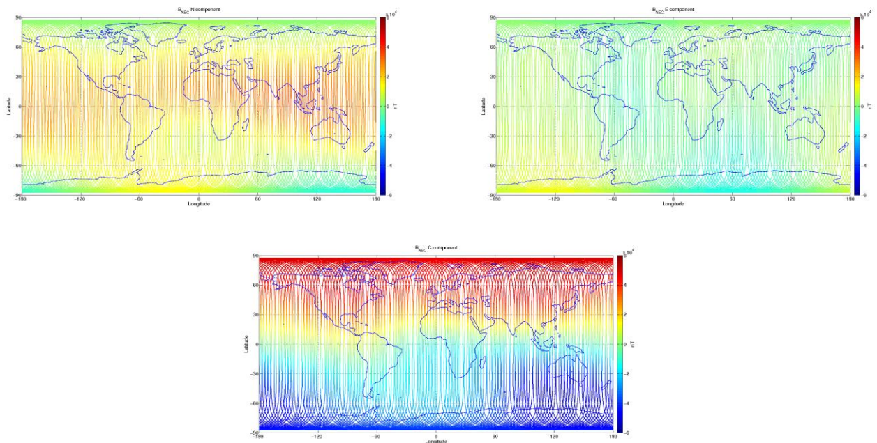
Figure 3-9: S/C C, world map plots of the geomagnetic field and components measured during monitoring period 16/03-22/03. From top to bottom: B_{NEC} components (North, East, and Centre) of magnetic field from VFM measurement.
