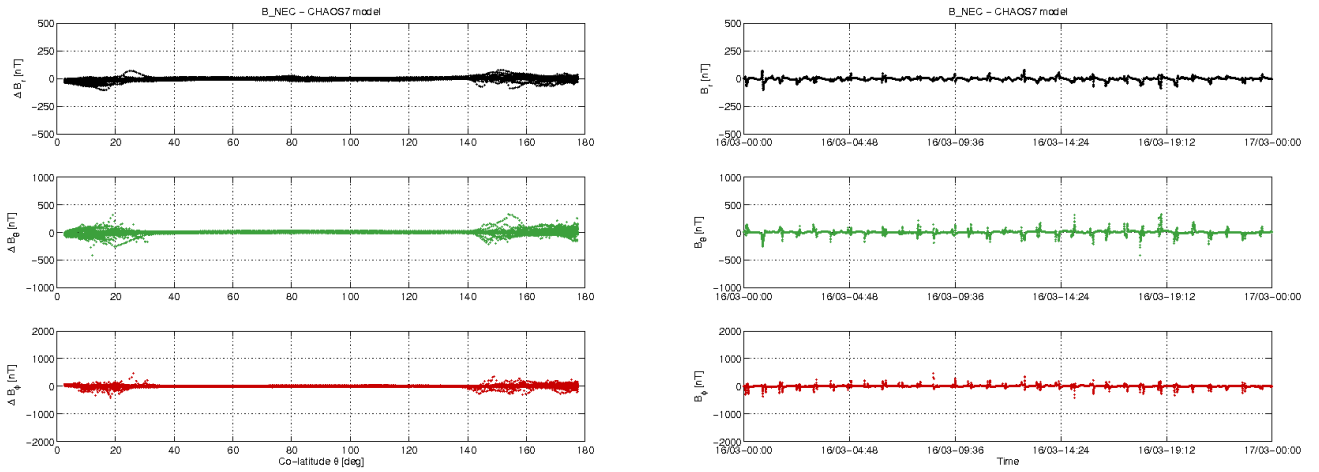
Figure 3-10: S/C A day 16.03: time series of B_{NEC} - B_{Chaos} residuals (right) and B_{NEC} - B_{Chaos} vs colatitude (left).
