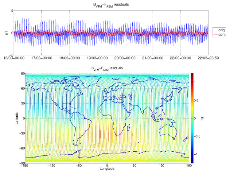
Figure 3-5: ASM-VFM residuals for S/C A, during monitoring period 16/03-22/03. In top figure are plotted: difference between |B_{VFM}| and F_{ASM} (without dB_{Sun} correction) (blue colour), and the residuals with dB_{Sun} corrections (red colour). In bottom figure residuals are presented on the world map.
