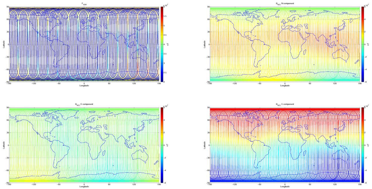
Figure 3-8: S/C B, world map plots of the geomagnetic field and components measured during monitoring period 16/03-22/03. From top to bottom: F-magnetic field from ASM measurement, B_{NEC} components (North, East, and Centre) of magnetic field from VFM measurement.
