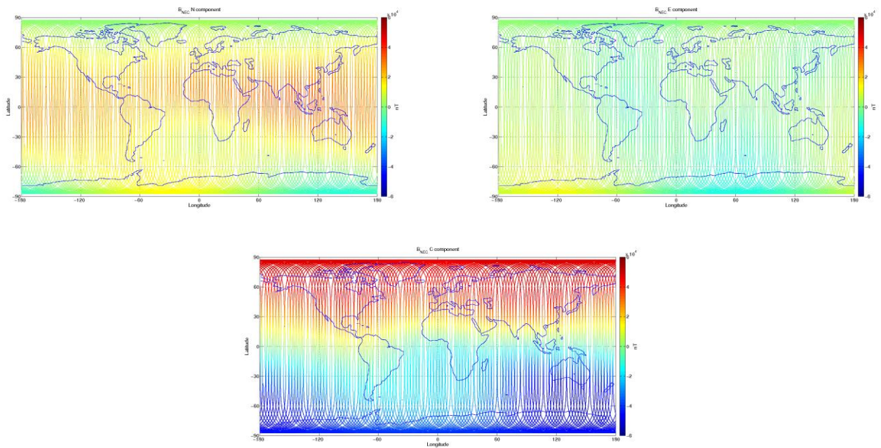
Figure 3-9: S/C C, world map plots of the geomagnetic field and components measured during monitoring period 09/03-15/03. From top to bottom: B_{NEC} components (North, East, and Centre) of magnetic field from VFM measurement.
