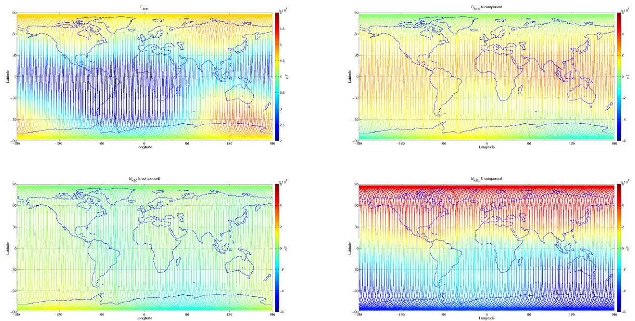
Figure 3-8: S/C B, world map plots of the geomagnetic field and components measured during monitoring period 09/03-15/03. From top to bottom: F-magnetic field from ASM measurement, B_{NEC} components (North, East, and Centre) of magnetic field from VFM measurement.
