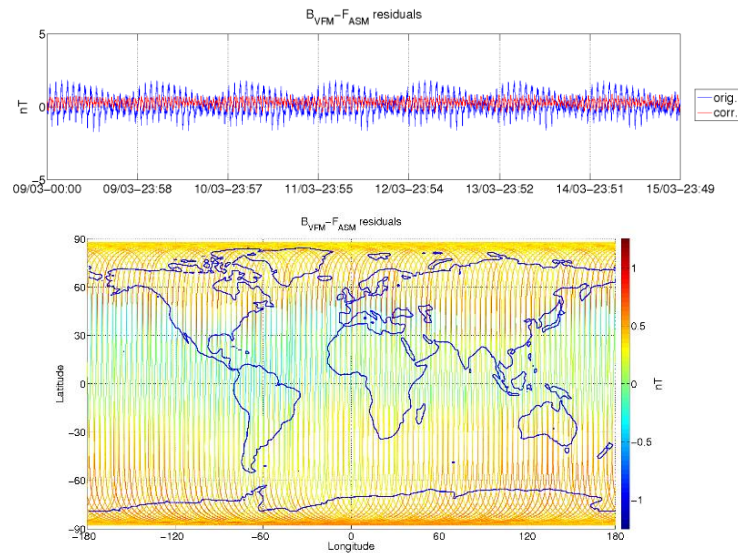
Figure 3-6: ASM-VFM residuals for S/C B, during monitoring period 09/03-15/03. In top figure are plotted: difference between |B_{VFM}| and F_{ASM} (without dB_{Sun} correction) (blue colour), and the residuals with dB_{Sun} corrections (red colour). In bottom figure residuals are presented on the world map.
