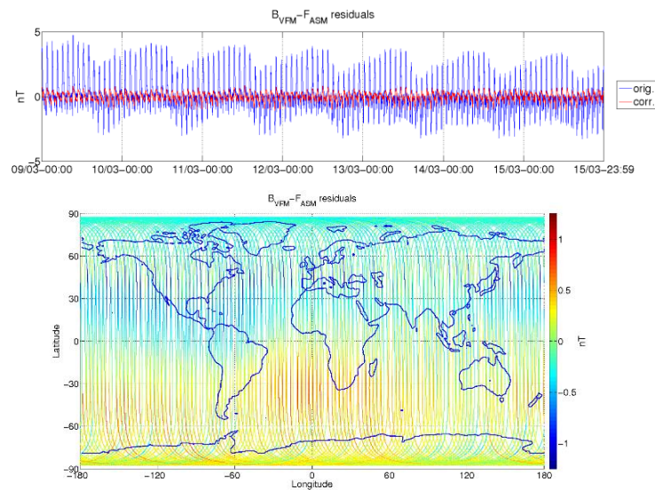
Figure 3-5: ASM-VFM residuals for S/C A, during monitoring period 09/03-15/03. In top figure are plotted: difference between |B_{VFM}| and F_{ASM} (without dB_{Sun} correction) (blue colour), and the residuals with dB_{Sun} corrections (red colour). In bottom figure residuals are presented on the world map.
