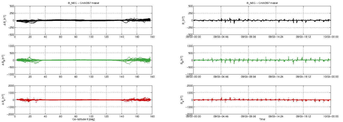
Figure 3-10: S/C A day 09.03: time series of B_{NEC} - B_{Chaos} residuals (right) and B_{NEC} - B_{Chaos} vs colatitude (left).
