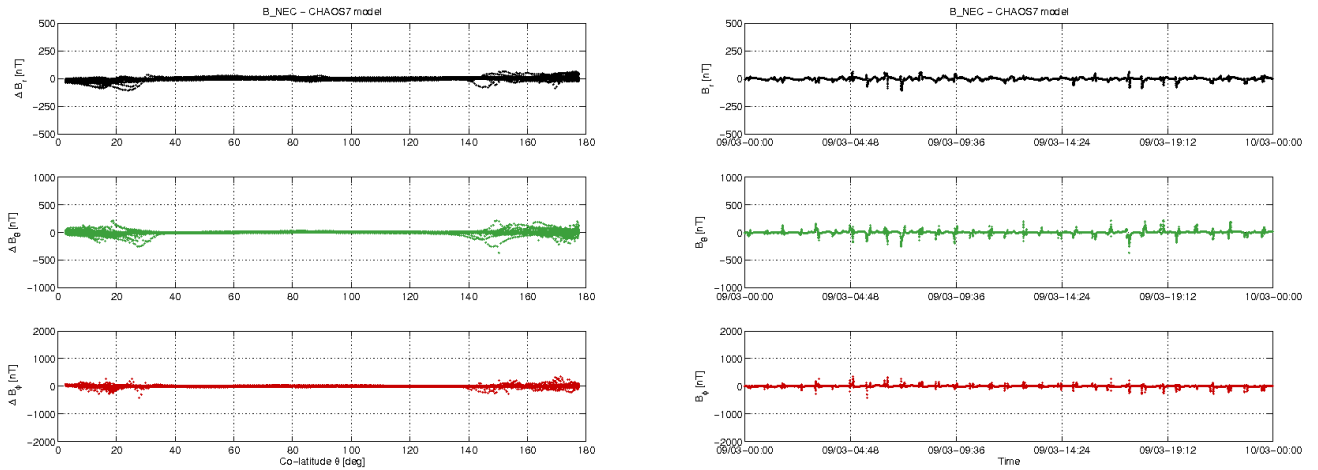
Figure 3-12: S/C C day 09/03: time series of B_{NEC} - B_{Chaos} residuals (right) and B_{NEC} - B_{Chaos} vs colatitude (left).
