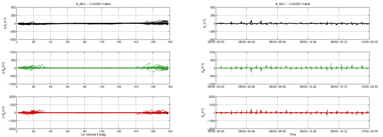
Figure 3-11: S/C B day 09.03: time series of B_{NEC} - B_{Chaos} residuals (right) and B_{NEC} - B_{Chaos} vs colatitude (left).
