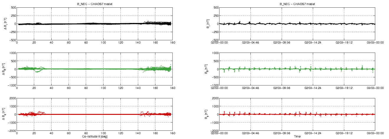
Figure 3-11: S/C B day 02.03: time series of B_{NEC} - B_{Chaos} residuals (right) and B_{NEC} - B_{Chaos} vs colatitude (left).
