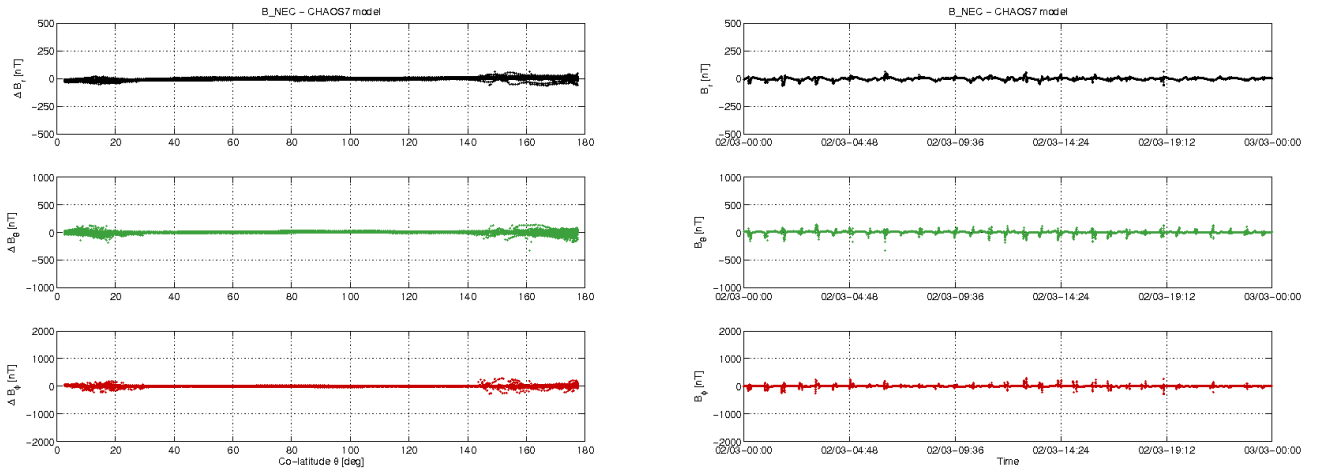
Figure 3-10: S/C A day 02.03: time series of B_{NEC} - B_{Chaos} residuals (right) and B_{NEC} - B_{Chaos} vs colatitude (left).
