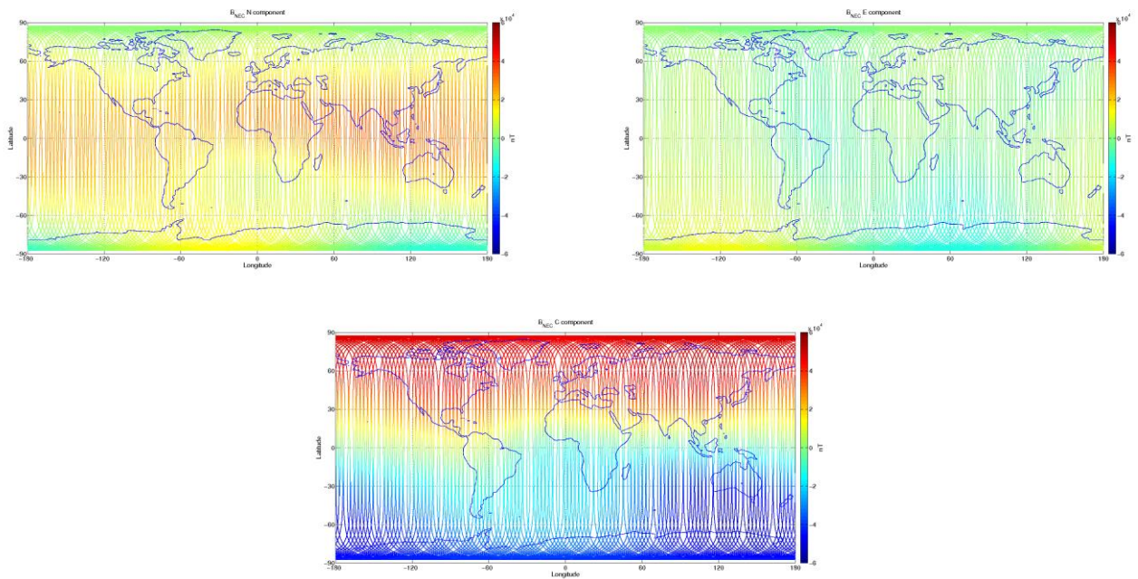
Figure 3-9: S/C C, world map plots of the geomagnetic field and components measured during monitoring period 02/03-08/03. From top to bottom: B_{NEC} components (North, East, and Centre) of magnetic field from VFM measurement.
