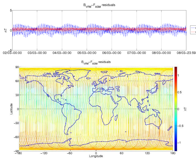
Figure 3-6: ASM-VFM residuals for S/C B, during monitoring period 02/03-08/03. In top figure are plotted: difference between |B_{VFM}| and F_{ASM} (without dB_Sun correction) (blue colour), and the residuals with dB_Sun corrections (red colour). In bottom figure residuals are presented on the world map.
