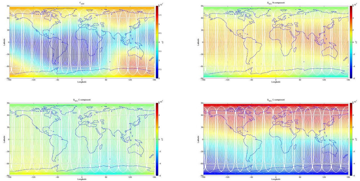
Figure 3-7: S/C A, world map plots of the geomagnetic field and components measured during monitoring period 02/03-08/03. From top to bottom: F-magnetic field from ASM measurement, B_{NEC} components (North, East, and Centre) of magnetic field from VFM measurement.
