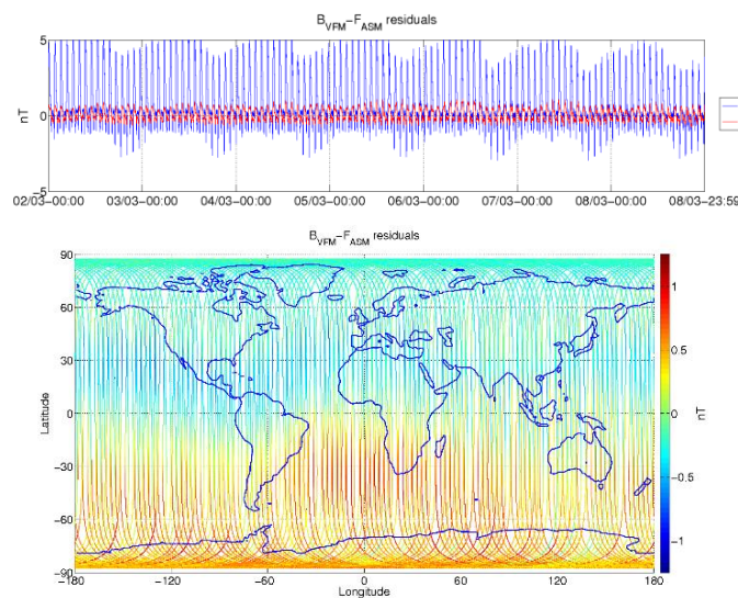
Figure 3-5: ASM-VFM residuals for S/C A, during monitoring period 02/03-08/03. In top figure are plotted: difference between |B_{VFM}| and F_{ASM} (without dB_{Sun} correction) (blue colour), and the residuals with dB_{Sun} corrections (red colour). In bottom figure residuals are presented on the world map.
