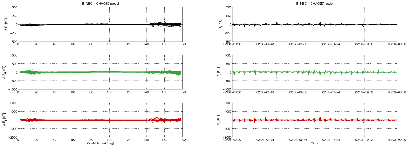
Figure 3-12: S/C C day 02.03: time series of B_{NEC} - B_{Chaos} residuals (right) and B_{NEC} - B_{Chaos} vs colatitude (left).
