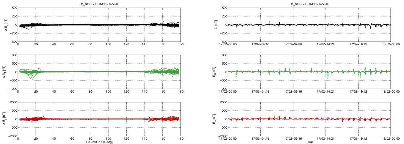
Figure 3-11: S/C B day 17.02: time series of B_{NEC} - B_{Chaos} residuals (right) and B_{NEC} - B_{Chaos} vs colatitude (left).
