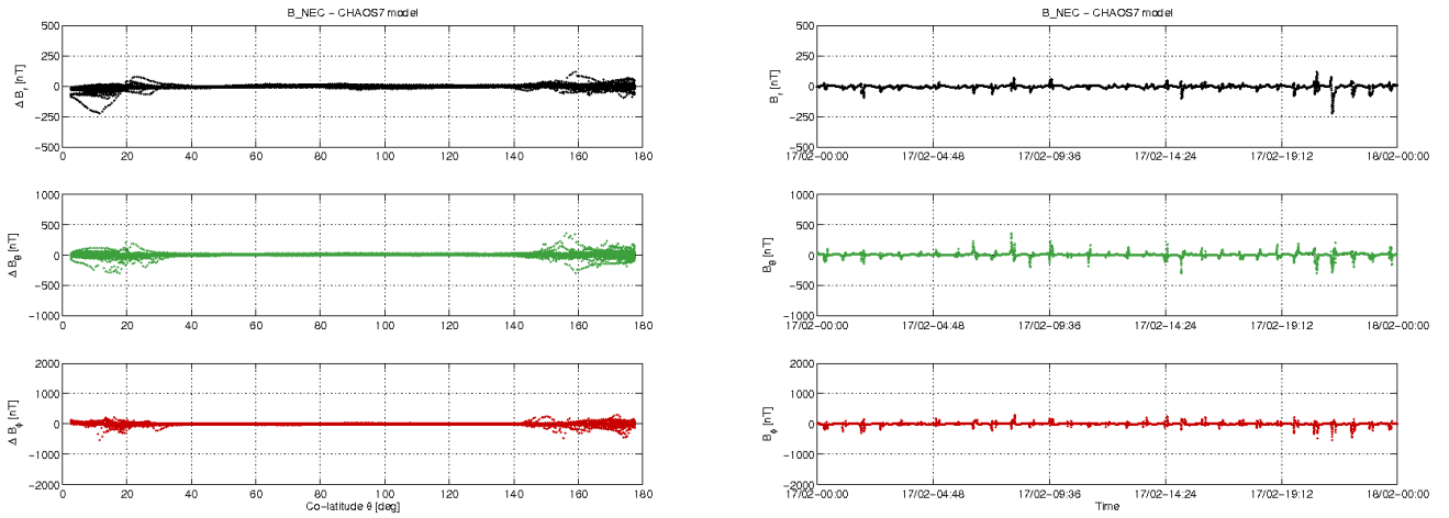
Figure 3-10: S/C A day 17.02: time series of B_{NEC} - B_{Chaos} residuals (right) and B_{NEC} - B_{Chaos} vs colatitude (left).
