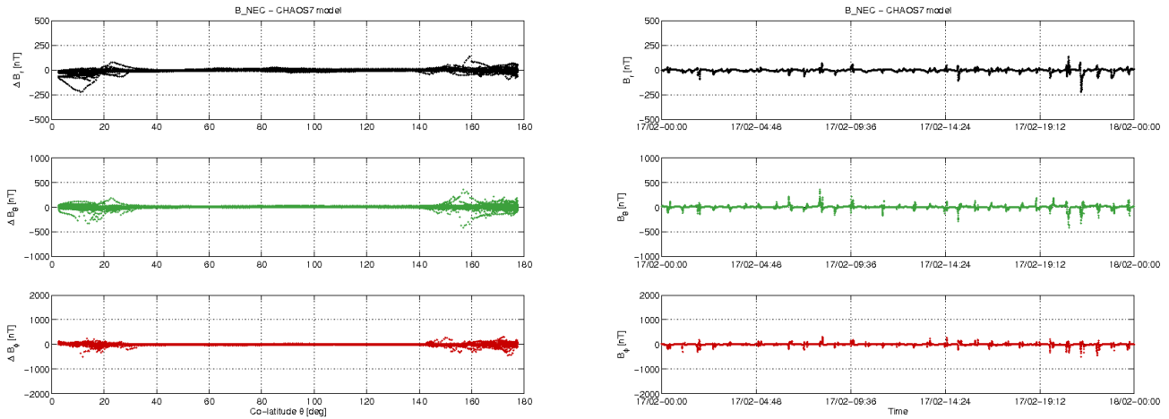
Figure 3-12: S/C C day 17.02: time series of B_{NEC} - B_{Chaos} residuals (right) and B_{NEC} - B_{Chaos} vs colatitude (left).
