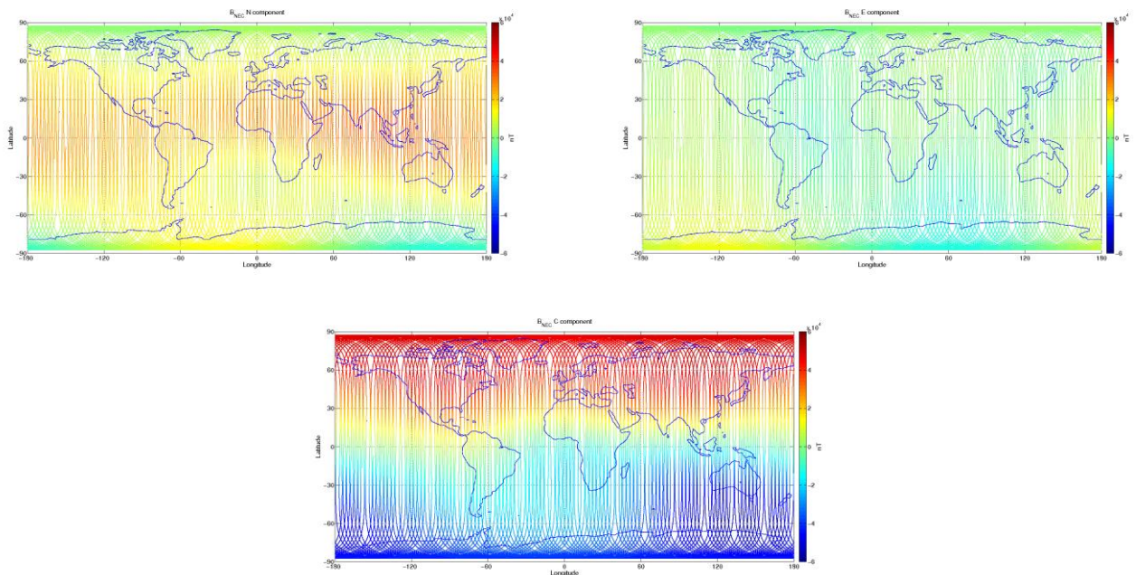
Figure 3-9: S/C C, world map plots of the geomagnetic field and components measured during monitoring period 17/02-23/02. From top to bottom: B_{NEC} components (North, East, and Centre) of magnetic field from VFM measurement.
