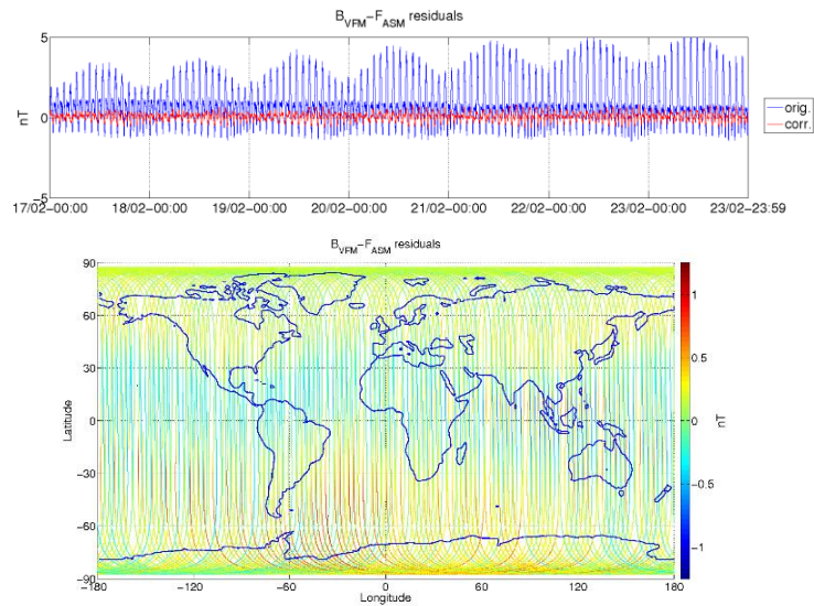
Figure 3-5: ASM-VFM residuals for S/C A, during monitoring period 17/02-23/02. In top figure are plotted: difference between |B_{VFM}| and F_{ASM} (without dB_{Sun} correction) (blue colour), and the residuals with dB_{Sun} corrections (red colour). In bottom figure residuals are presented on the world map.
