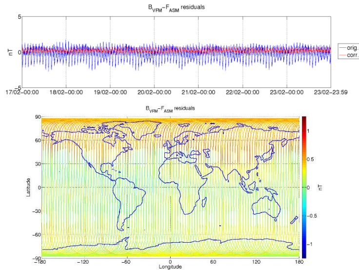
Figure 3-6: ASM-VFM residuals for S/C B, during monitoring period 17/02-23/02. In top figure are plotted: difference between |B_{VFM}| and F_{ASM} (without dB_{Sun} correction) (blue colour), and the residuals with dB_{Sun} corrections (red colour). In bottom figure residuals are presented on the world map.
