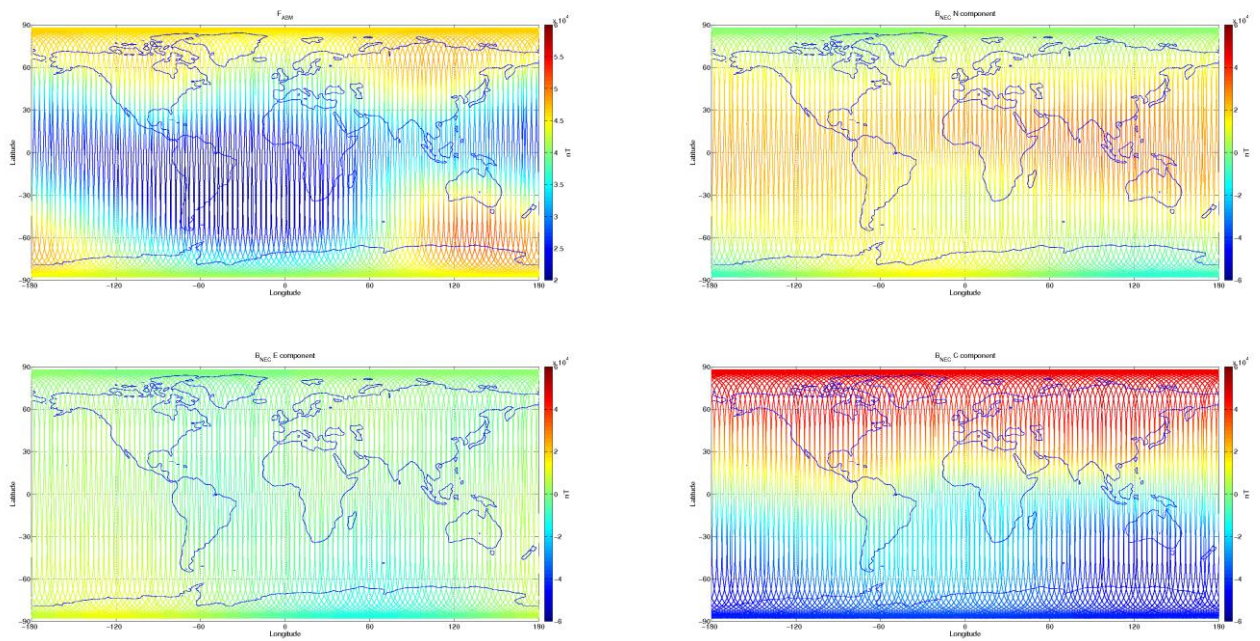
Figure 3-8: S/C B, world map plots of the geomagnetic field and components measured during monitoring period 17/02-23/02. From top to bottom: F-magnetic field from ASM measurement, B_{NEC} components (North, East, and Centre) of magnetic field from VFM measurement.
