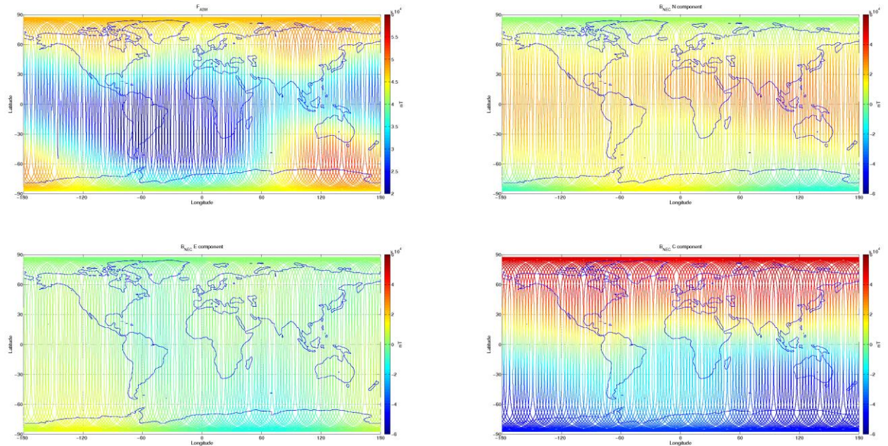
Figure 3-7: S/C A, world map plots of the geomagnetic field and components measured during monitoring period 10/02-16/02. From top to bottom: F-magnetic field from ASM measurement, B_{NEC} components (North, East, and Centre) of magnetic field from VFM measurement.
