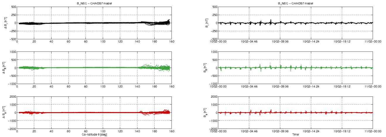
Figure 3-12: S/C C day 10.02: time series of B_{NEC} - B_{Chaos} residuals (right) and B_{NEC} - B_{Chaos} vs colatitude (left).
