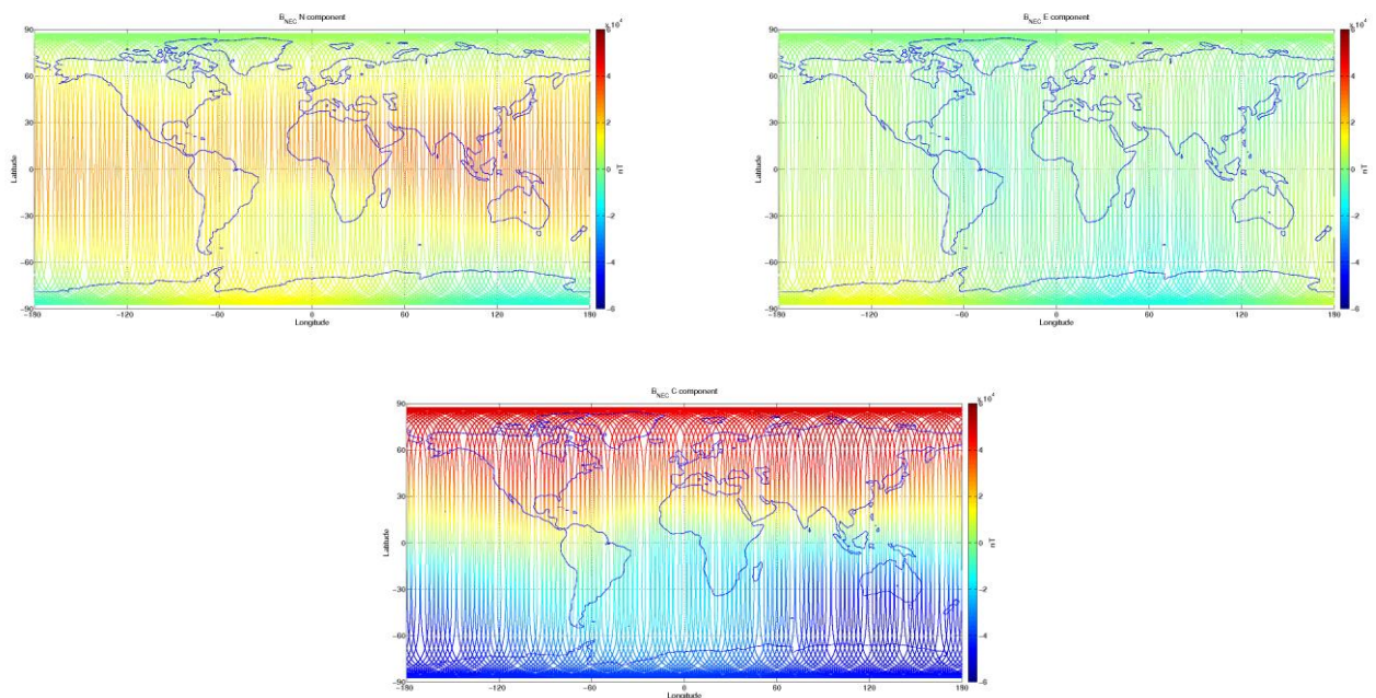
Figure 3-9: S/C C, world map plots of the geomagnetic field and components measured during monitoring period 10/02-16/02. From top to bottom: B_{NEC} components (North, East, and Centre) of magnetic field from VFM measurement.
