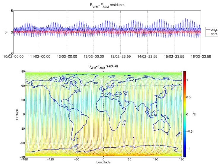
Figure 3-5: ASM-VFM residuals for S/C A, during monitoring period 10/02-16/02. In top figure are plotted: difference between |B_{VFM}| and F_{ASM} (without dB_Sun correction) (blue colour), and the residuals with dB_Sun corrections (red colour). In bottom figure residuals are presented on the world map.
