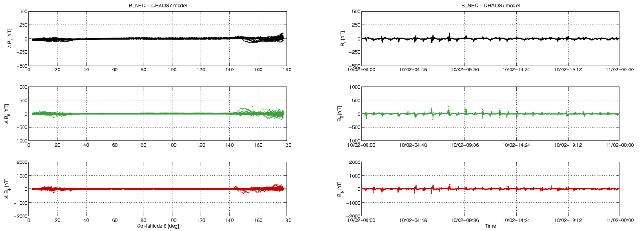
Figure 3-10: S/C A day 10.02: time series of B_{NEC} - B_{Chaos} residuals (right) and B_{NEC} - B_{Chaos} vs colatitude (left).
