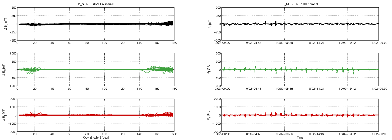
Figure 3-11: S/C B day 10.02: time series of B_{NEC} - B_{Chaos} residuals (right) and B_{NEC} - B_{Chaos} vs colatitude (left).
