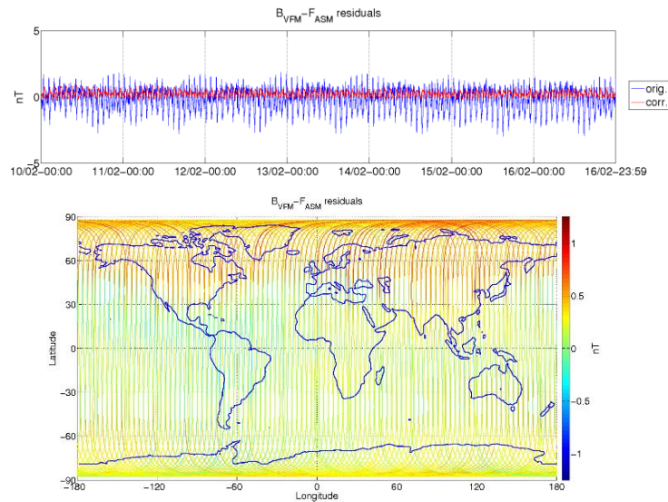
Figure 3-6: ASM-VFM residuals for S/C B, during monitoring period 10/02-16/02. In top figure are plotted: difference between |B_{VFM}| and F_{ASM} (without dB_{Sun} correction) (blue colour), and the residuals with dB_{Sun} corrections (red colour). In bottom figure residuals are presented on the world map.
